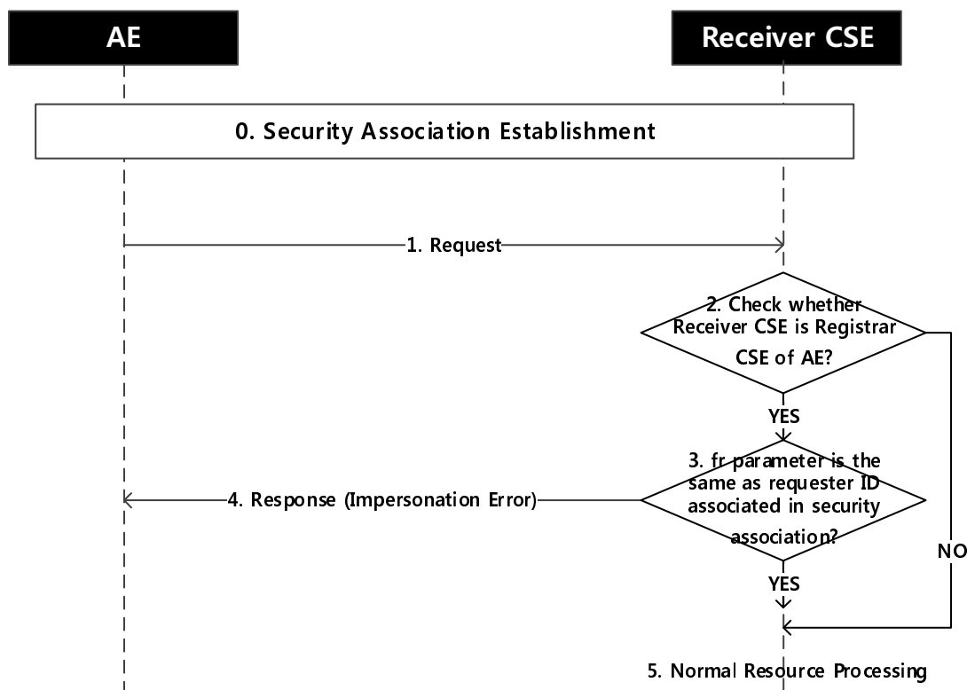
Figure 7.2-1: AE impersonation checking procedure
