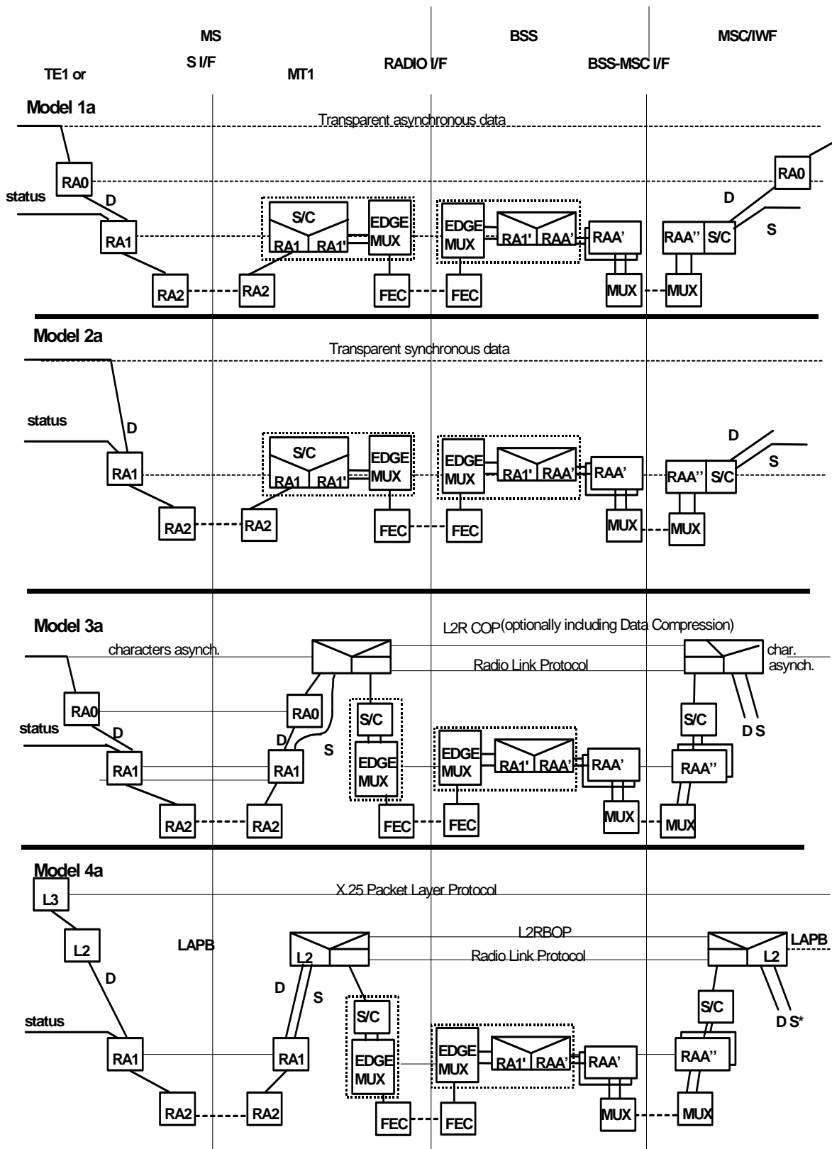
Figure 8 (continued) : Information transfer protocol models for GSM PLMN connections using EDGE channels
