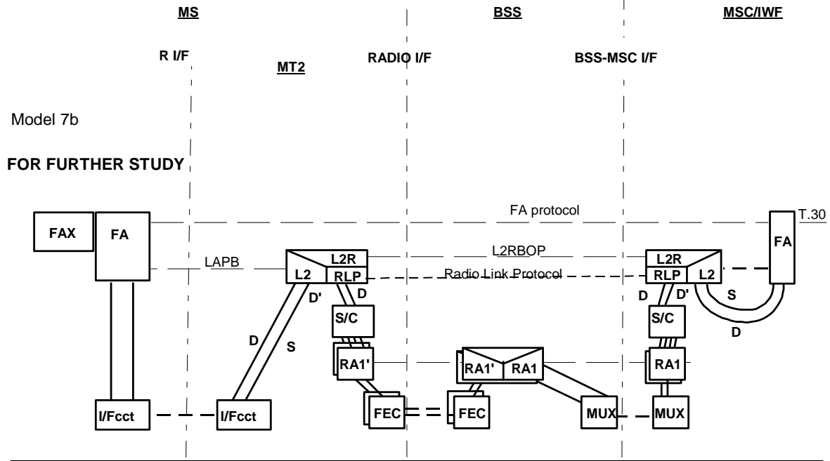
Figure 6 (concluded): Information transfer protocol models for GSM PLMN connections
