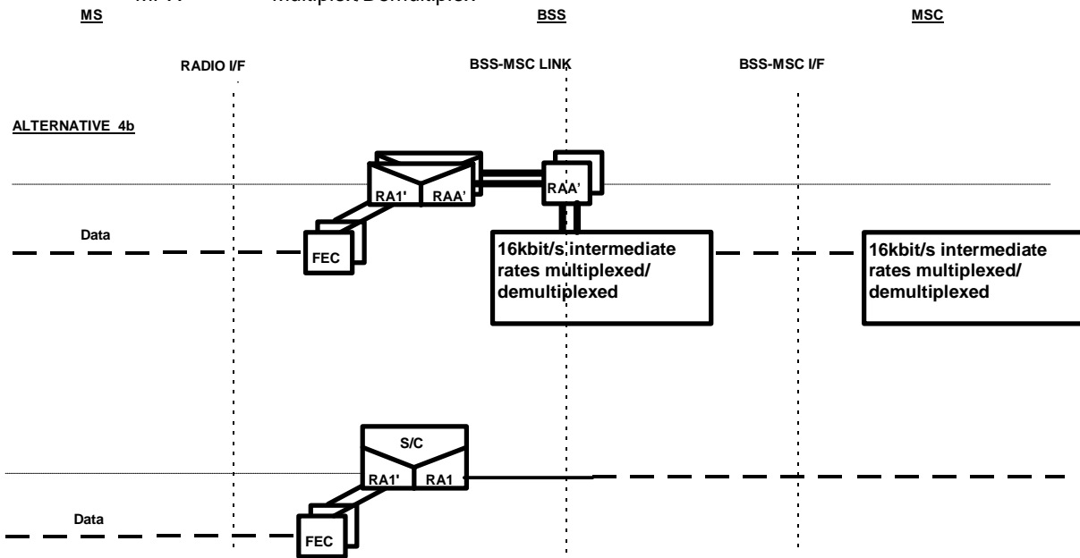
Figure 8 (concluded): Location of transcoding and rate adaptation
