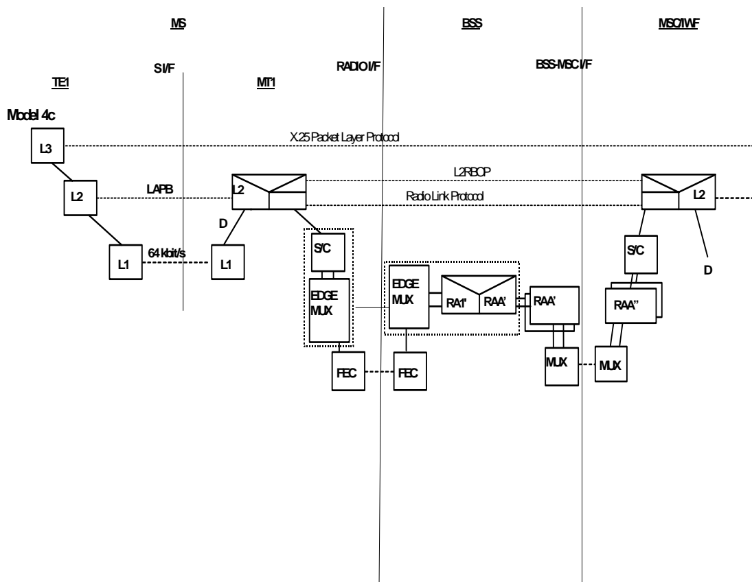
Figure 8 (continued) : Information transfer protocol models for GSM PLMN connections using EDGE channels
