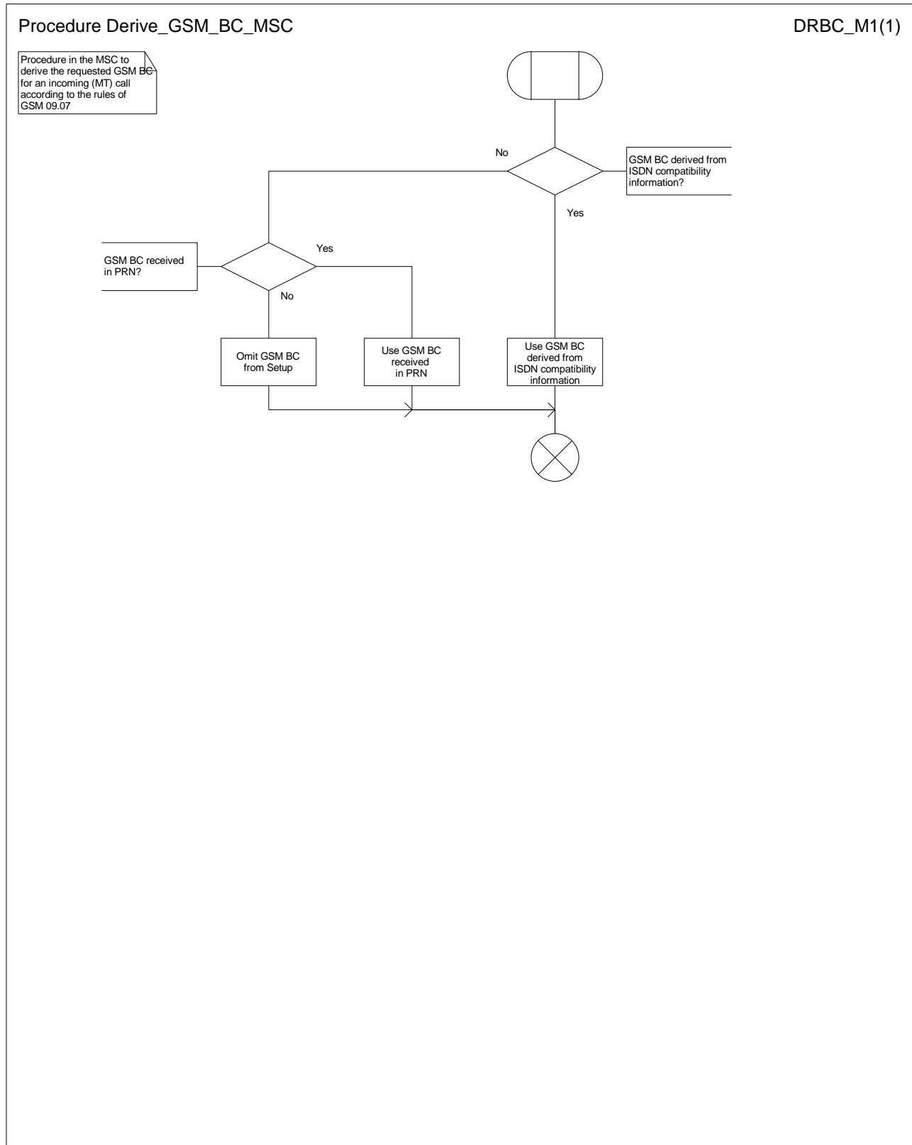
Figure 64: Derive_GSM_BC_MSC
