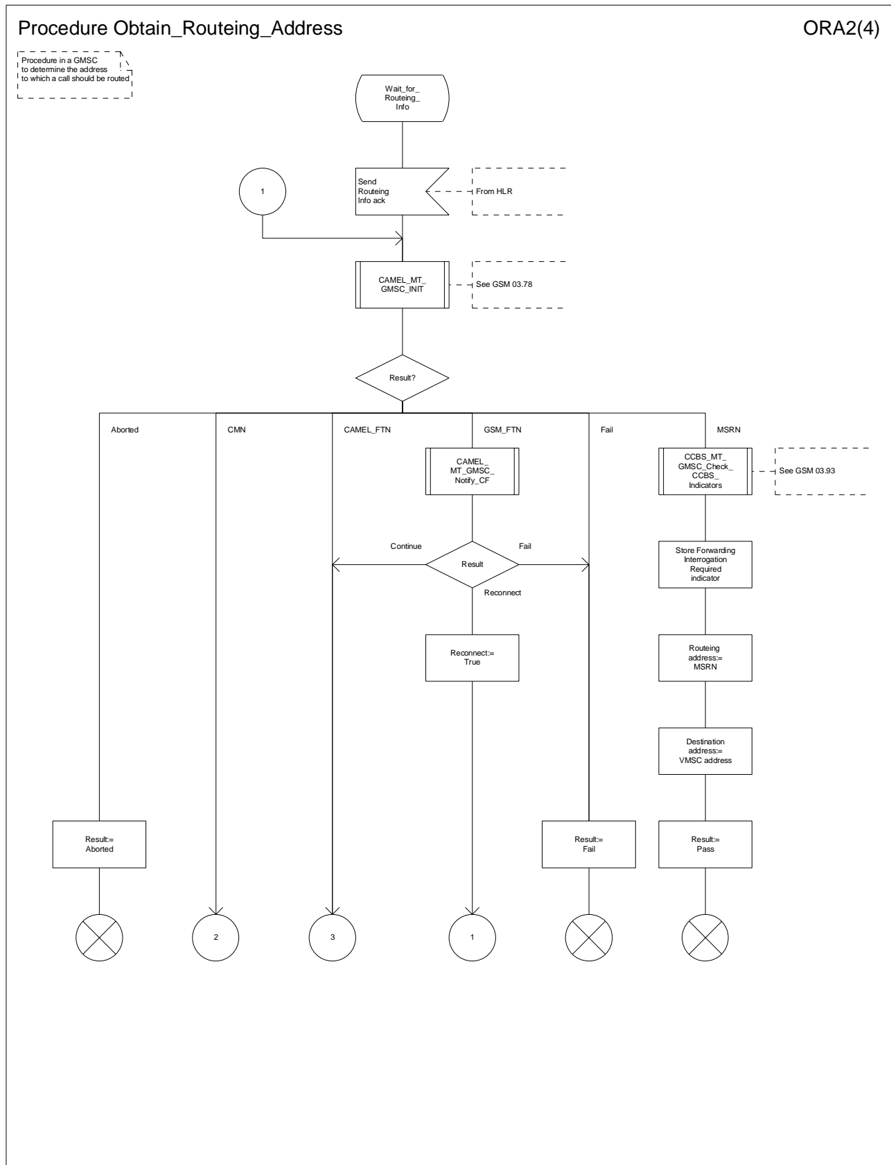
Figure 36b: Procedure Obtain_Routeing_Address (sheet 2)
