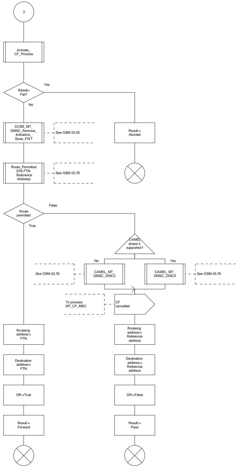
Figure 36d: Procedure Obtain_Routeing_Address (sheet 4)
