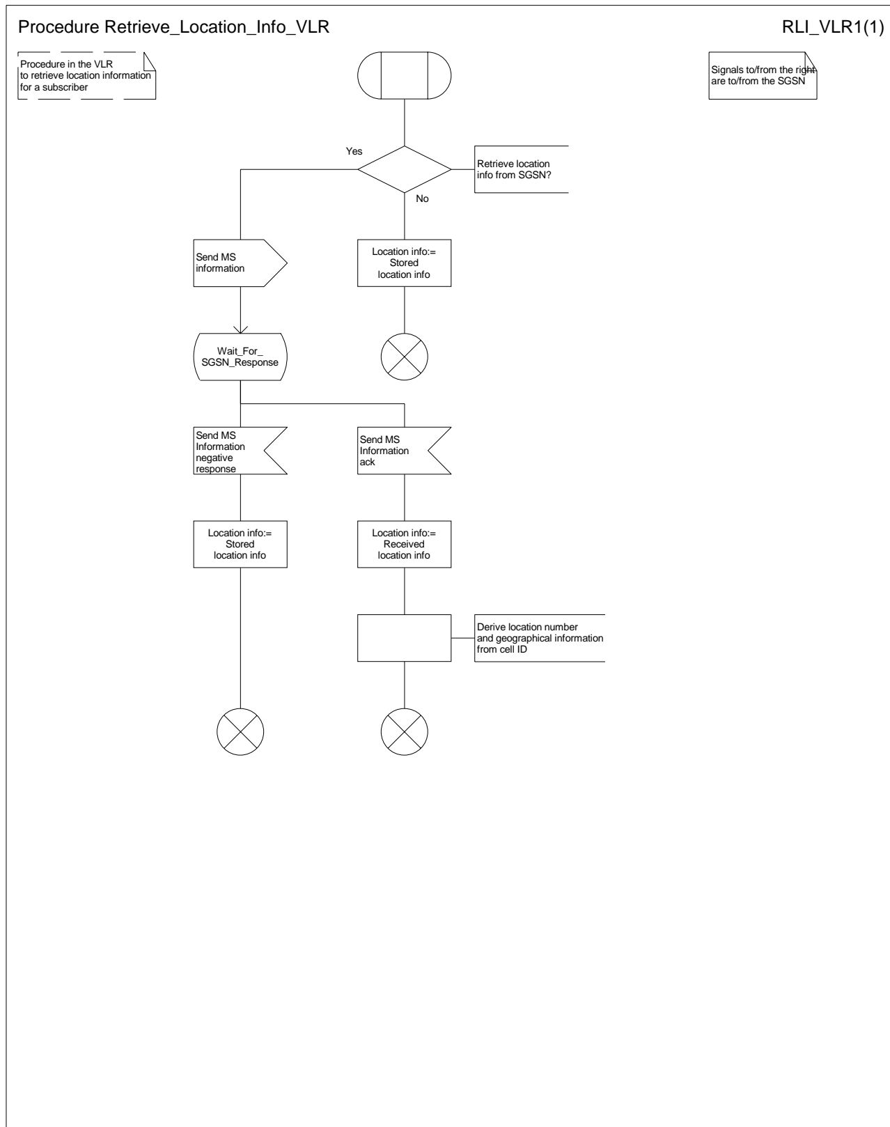
Figure 56c: Procedure Retrieve_Location_Info_VLR
