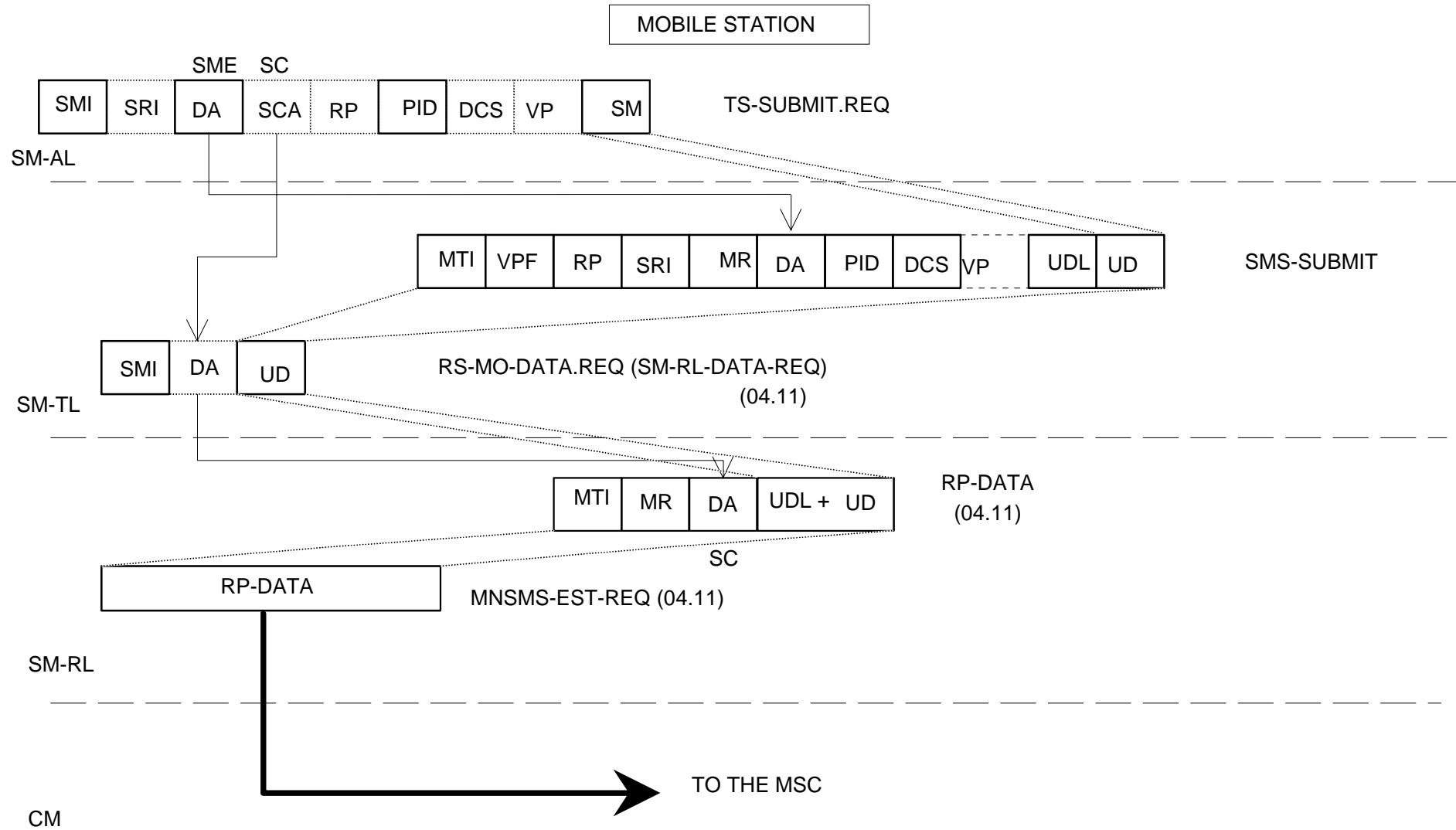
Figure 3.1: Mobile originated short message
