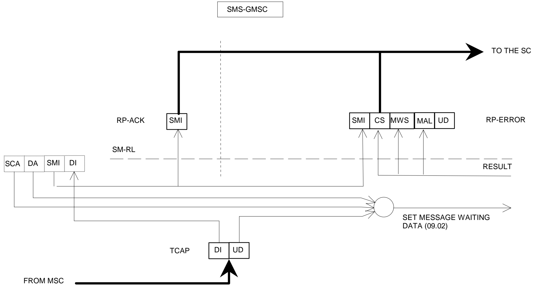
Figure 2.3a: Acknowledgement in the MT case
