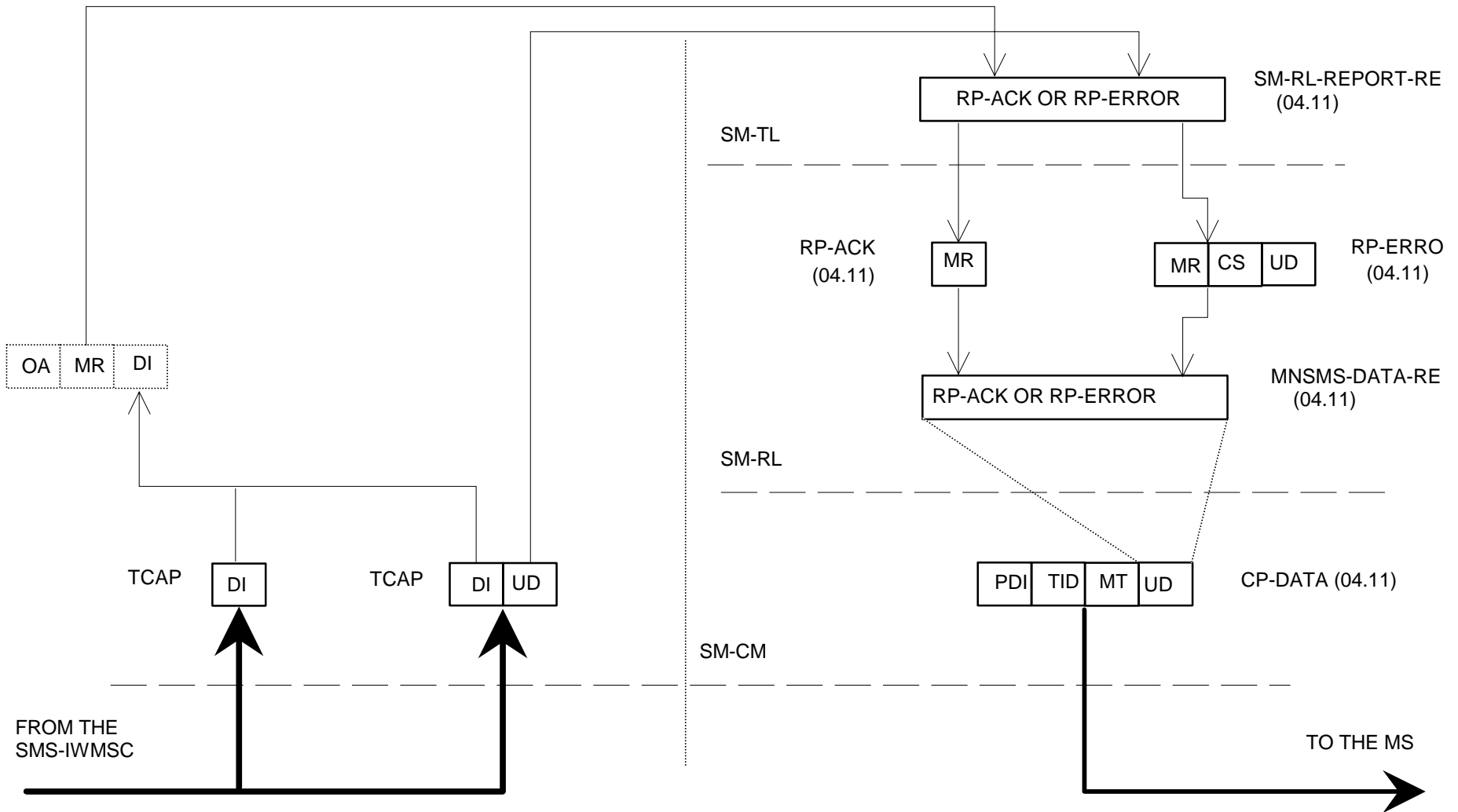
Figure 4.2: Acknowledgement in the MO case
