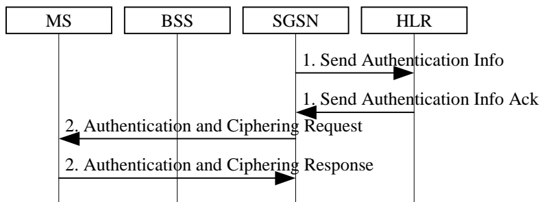
Figure 23: Authentication Procedure
