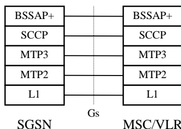
Figure 7: Signalling Plane SGSN - MSC/VLR
