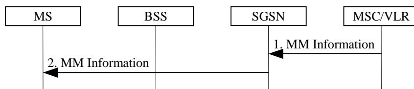
Figure 17: MM Information Procedure
