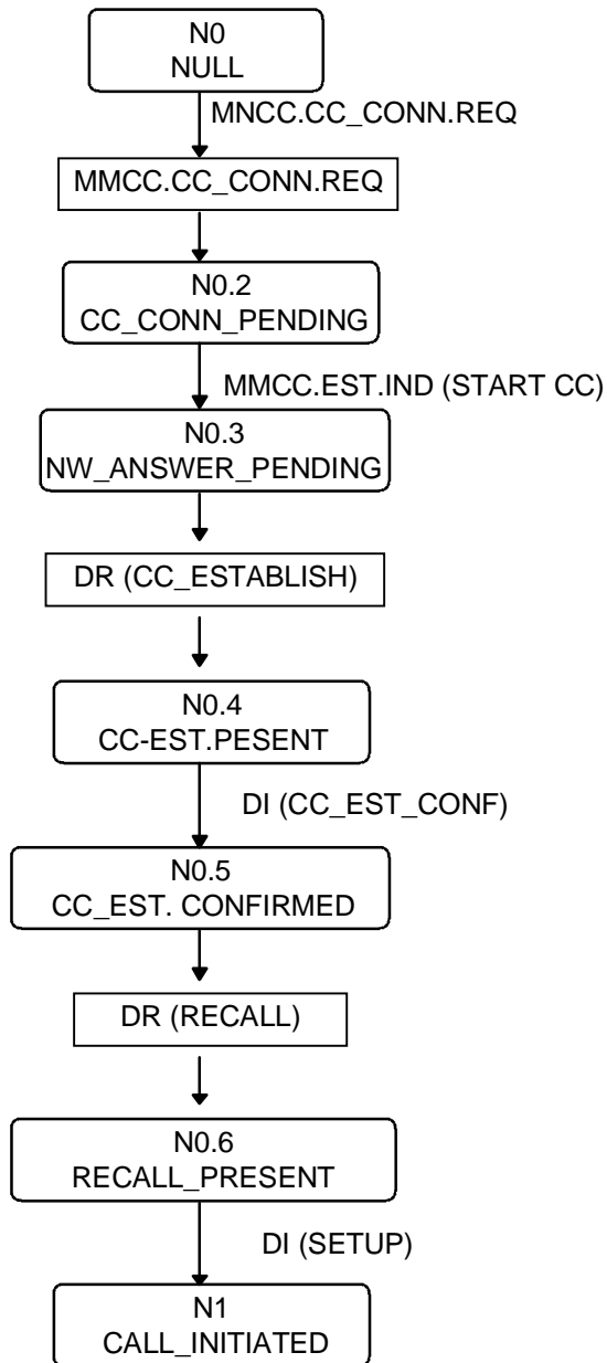
FIGURE 5.1b.1/3GPP TS 04.08: Overview call control protocol/Network side, extension
