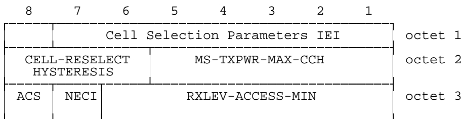
Figure 10.18/3GPP TS 04.08: Cell Selection Parameters information element
