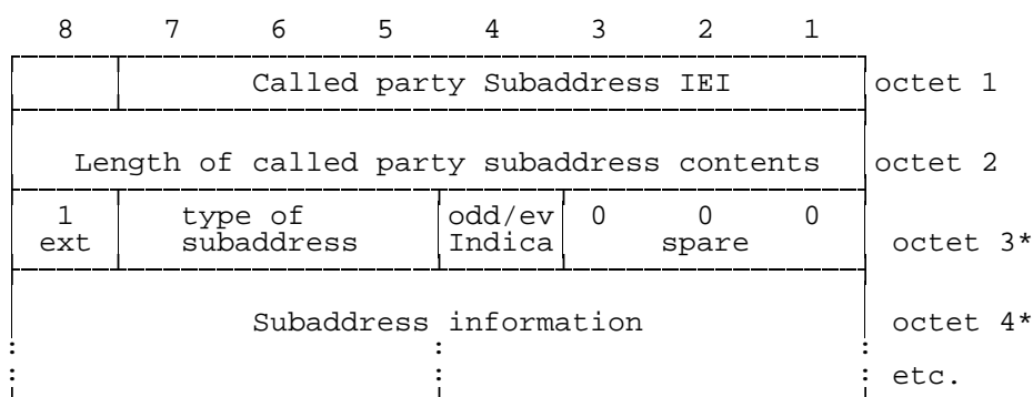
Figure 10.74/3GPP TS 04.08: Called party subaddress
