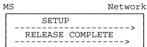
Figure 5.7b/3GPP TS 04.08: Recall acceptance or rejection by user
