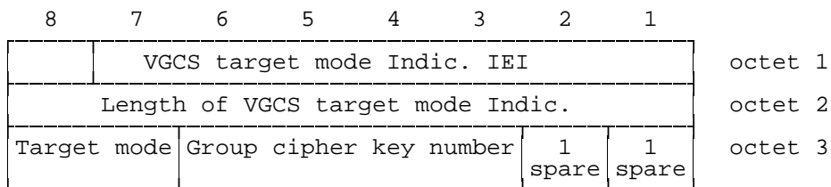
Figure 10.59c/3GPP TS 04.08: VGCS target mode Indication information element
