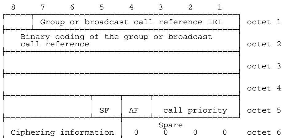
Figure 10.8bis/3GPP TS 04.08: Descriptive Group or Broadcast Call Reference
