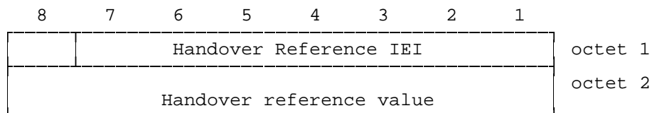
Figure 10.33/3GPP TS 04.08: Handover Reference information element
