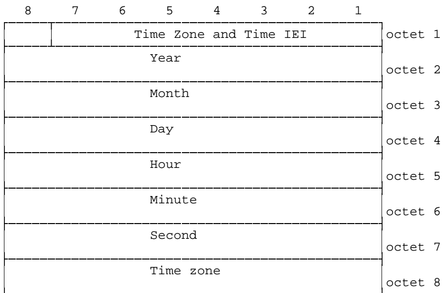
Figure 10.68a/3GPP TS 04.08: Time Zone and Time information element
