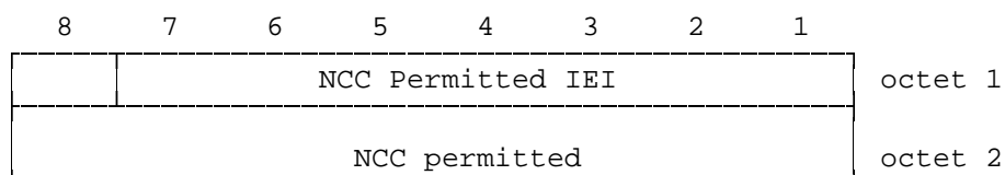
Figure 10.45/3GPP TS 04.08: NCC Permitted information element
