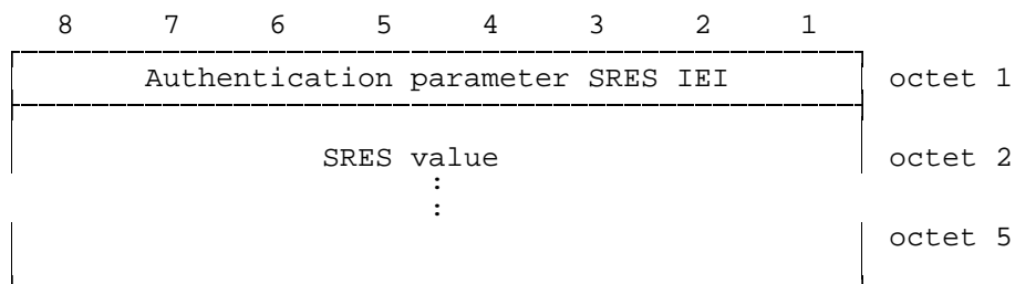
Figure 10.62/3GPP TS 04.08: Authentication Parameter SRES information element
