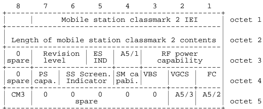
Figure 10.7/3GPP TS 04.08: Mobile Station Classmark 2 information element
