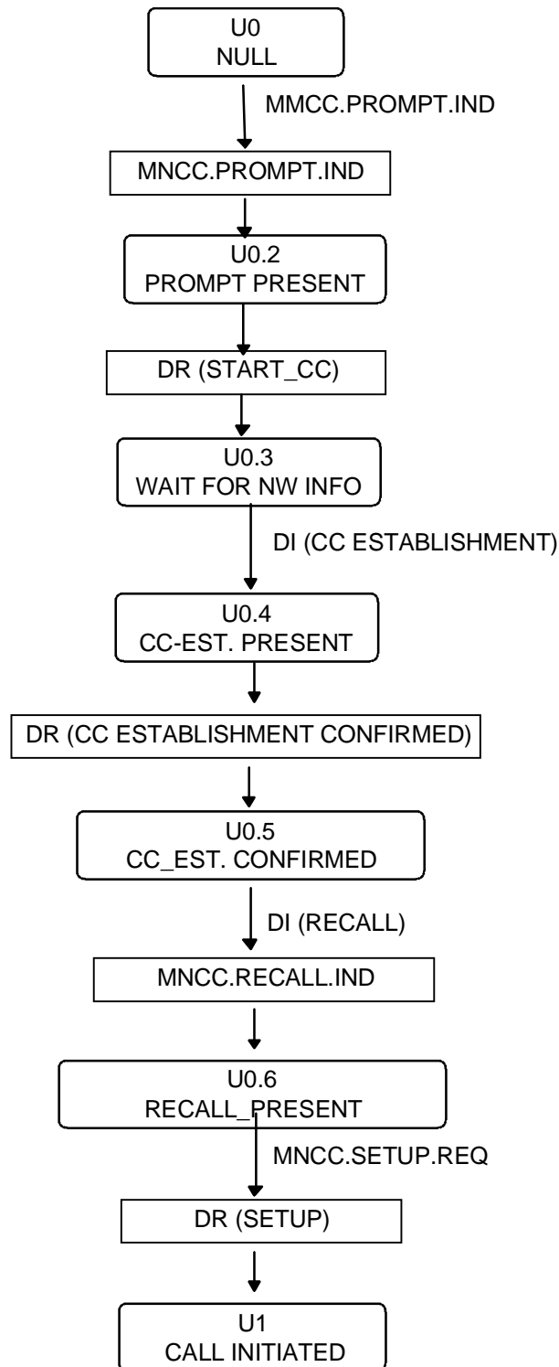
Figure 5.1a.1/3GPP TS 04.08: Overview call control protocol/MS side, extension
