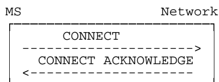
Figure 5.7/3GPP TS 04.08: Call acceptance and active indication at mobile terminating call establishment
