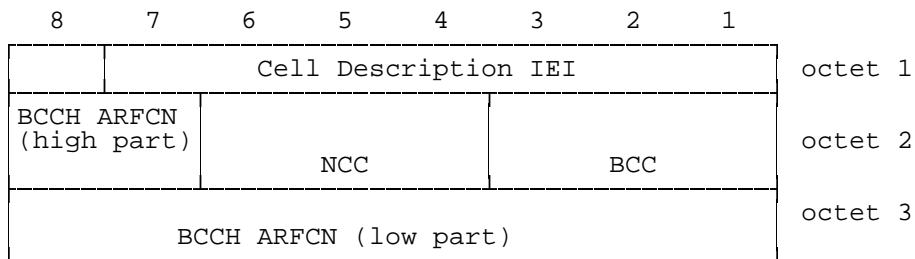
Figure 10.16/3GPP TS 04.08: Cell Description information element
