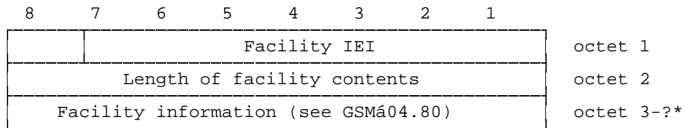
Figure 10.82/3GPP TS 04.08
