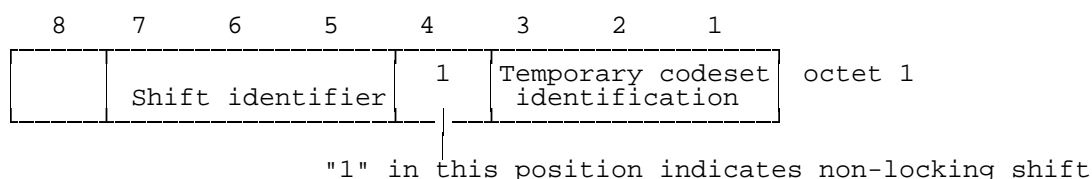
Figure 10.69/3GPP TS 04.08: Non-locking shift element
