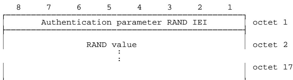
Figure 10.61/3GPP TS 04.08: Authentication Parameter RAND information element
