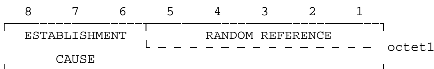
Figure 9.4/3GPP TS 04.08: UPLINK ACCESS message content
