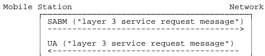
Figure 3.1/3GPP TS 04.08 Service request and contention resolution
