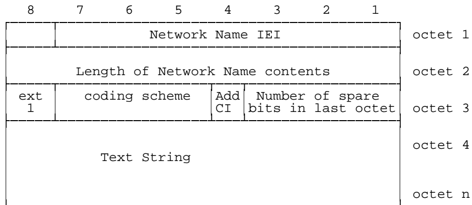
Figure 10.65a/3GPP TS 04.08: Network Name information element
