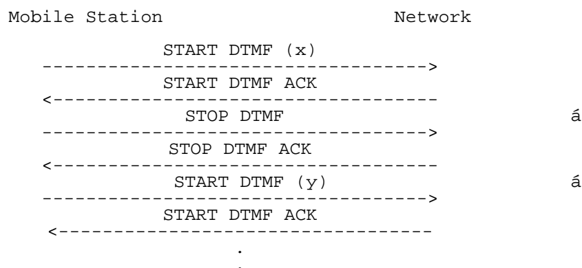
Figure 5.9/3GPP TS 04.08: Multiple DTMF transmission
