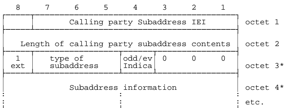
Figure 10.76/3GPP TS 04.08: Calling party subaddress
