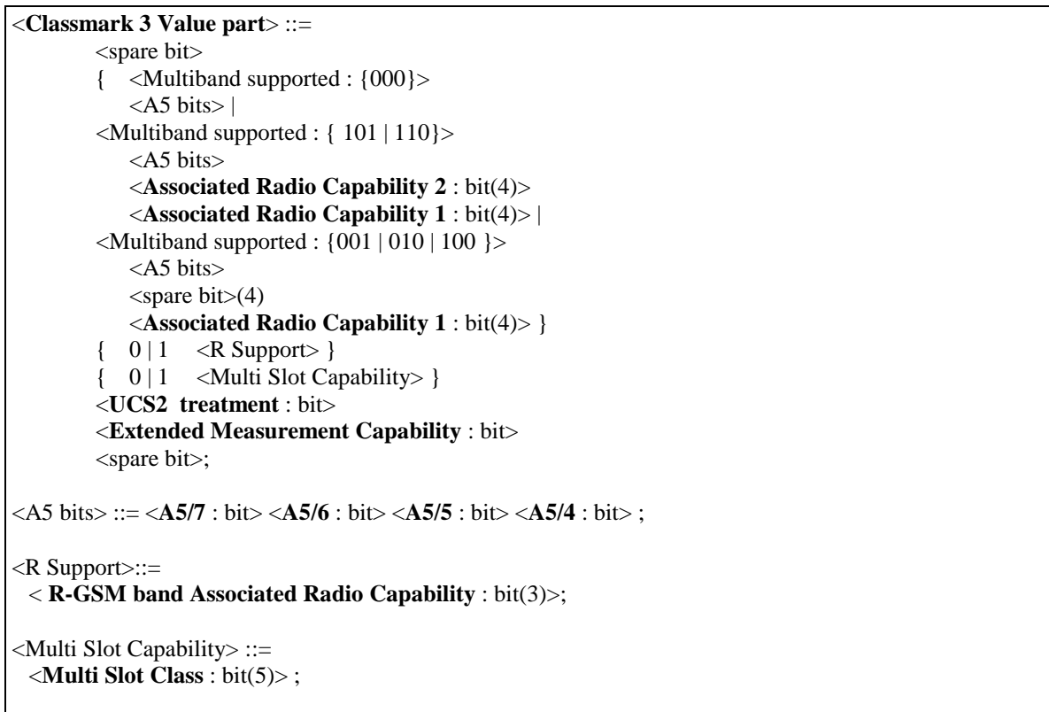
Figure 10.8/3GPP TS 04.08: Mobile Station Classmark 3 information element
