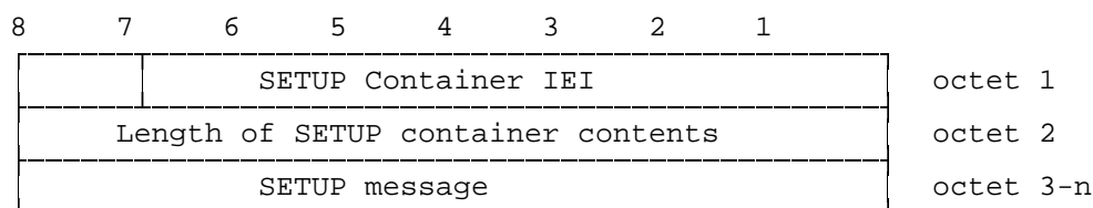
Figure 10.89b/3GPP TS 04.08: Octet j (j = 3, 4 ... n) is the unchanged octet j of the SETUP message.
