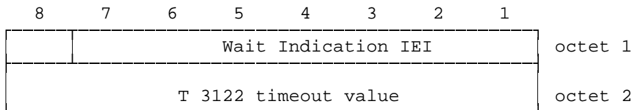
Figure 10.60/3GPP TS 04.08: Wait Indication information element
