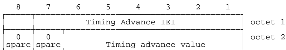
Figure 10.57/3GPP TS 04.08: Timing Advance information element
