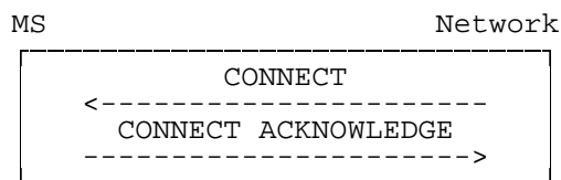
Figure 5.5/3GPP TS 04.08: Call acceptance sequence at mobile originating call establishment
