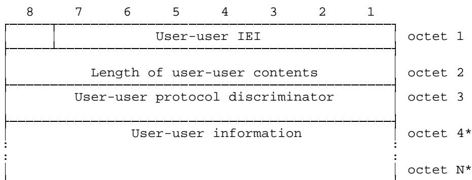
Figure 10.92/3GPP TS 04.08: User-user information element
