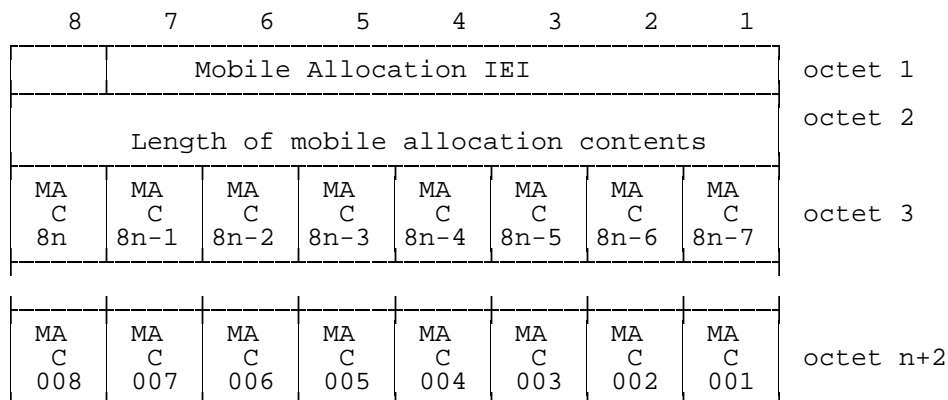
Figure 10.39/3GPP TS 04.08: Mobile Allocation information element
