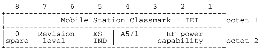
Figure 10.6/3GPP TS 04.08: Mobile Station Classmark 1 information element
