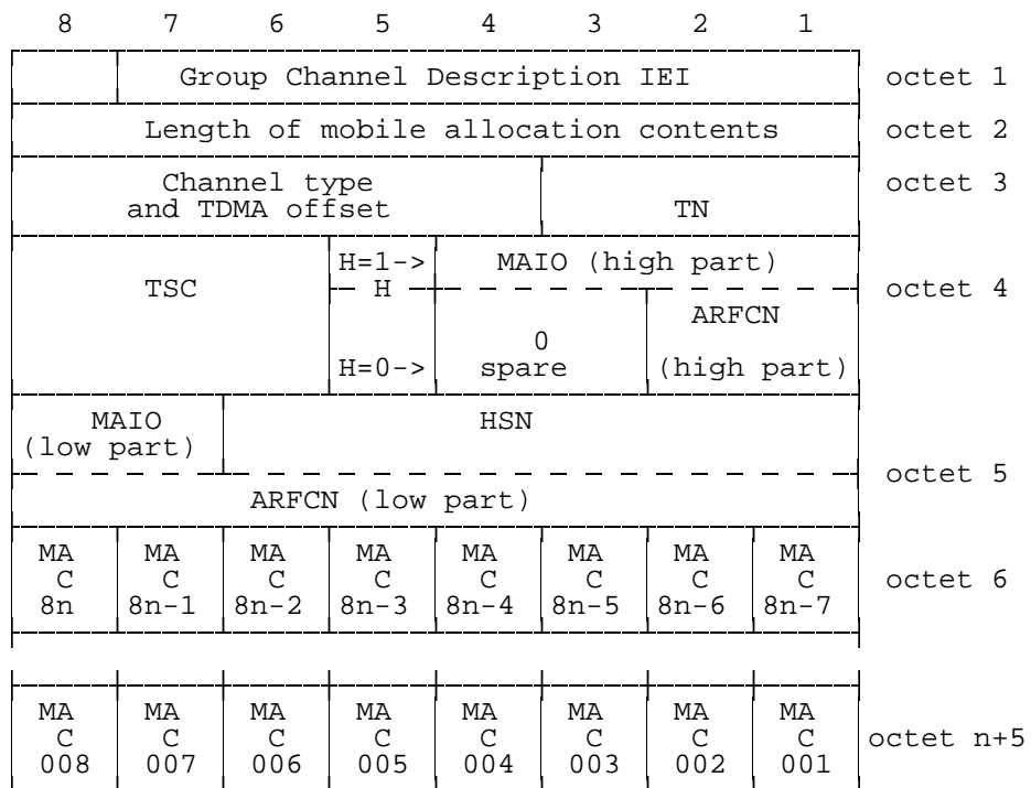
Figure 10.32a/3GPP TS 04.08: Group Channel Description information element
