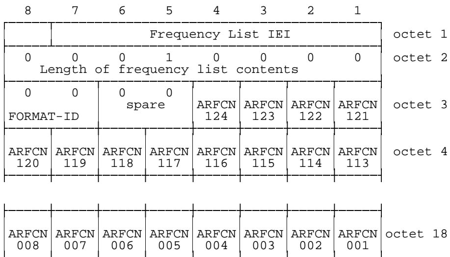
Figure 10.27/3GPP TS 04.08: Frequency List information element, bit map 0 format
