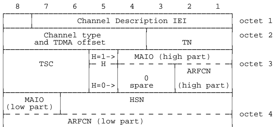
Figure 10.19a/3GPP TS 04.08: Channel Description 2 information element
