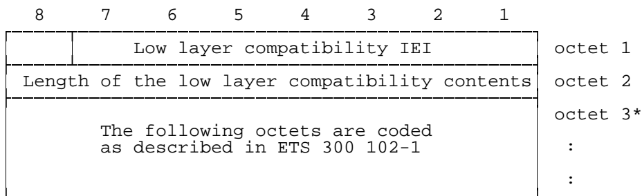
Figure 10.85/3GPP TS 04.08: Low layer compatibility information element
