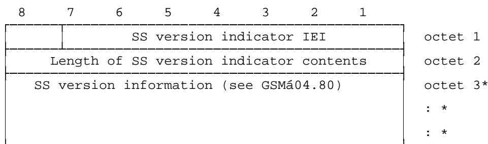
Figure 10.91/3GPP TS 04.08
