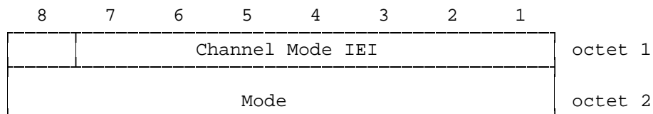
Figure 10.20/3GPP TS 04.08: Channel Mode information element
