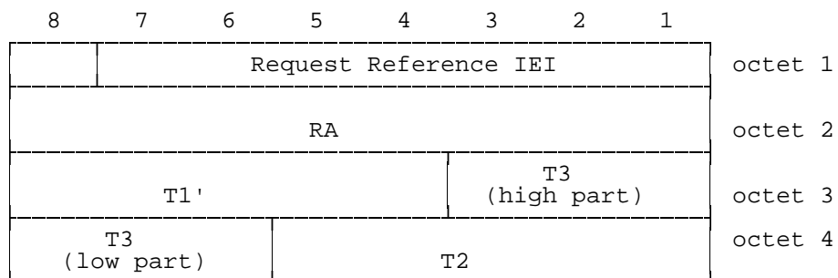
Figure 10.48/3GPP TS 04.08: Request Reference information element
