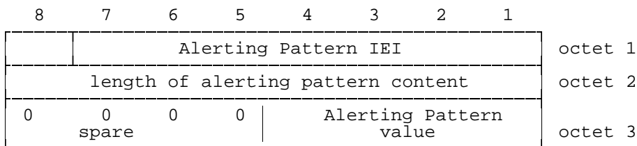
FIGURE 10.93/3GPP TS 04.08: Alerting Pattern information element
