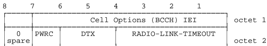
Figure 10.17/3GPP TS 04.08: Cell Options (BCCH) information element
