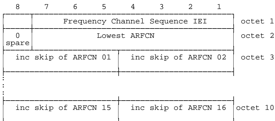
Figure 10.26/3GPP TS 04.08: Frequency Channel Sequence information element
