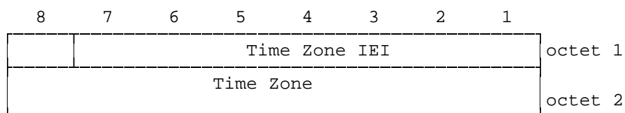
Figure 10.67a/3GPP TS 04.08: Time Zone information element
