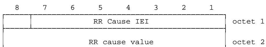
Figure 10.49/3GPP TS 04.08: RR Cause information element
