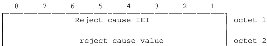
Figure 10.66/3GPP TS 04.08: Reject Cause information element
