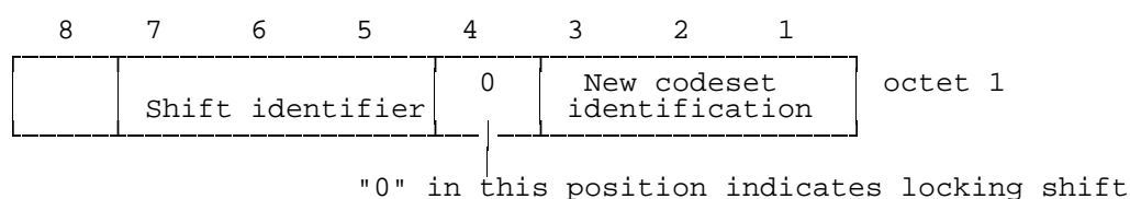
Figure 10.68/3GPP TS 04.08: Locking shift element
