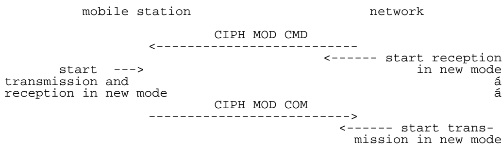
Figure 3.3/3GPP TS 04.08: Cipherring mode setting sequence
