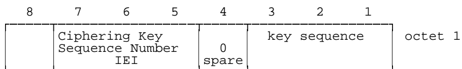
Figure 10.3/3GPP TS 04.08: Cipherng Key Sequence Number information element
