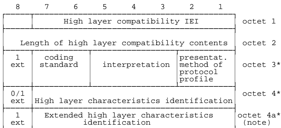
Figure 10.83/3GPP TS 04.08: High layer compatibility information element
