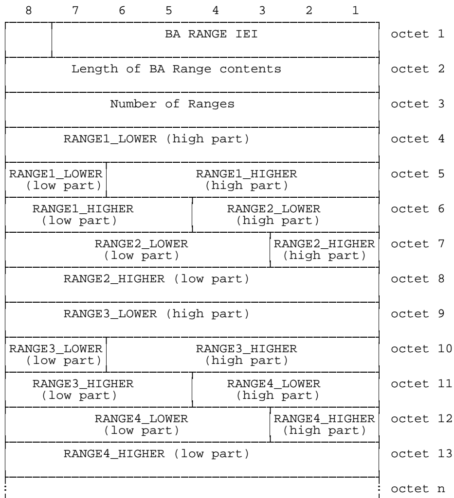
Figure 10.8a/3GPP TS 04.08: BA RANGE information element
