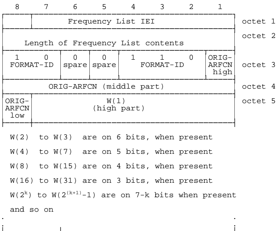
Figure 10.31/3GPP TS 04.08: Frequency List information element (Range 128 format)
