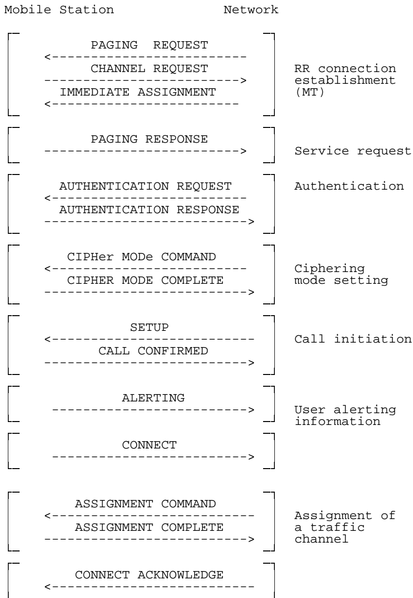
Figure 7.11b/3GPP TS 04.08: Mobile terminating call establishment with OACSU (late assignment)
