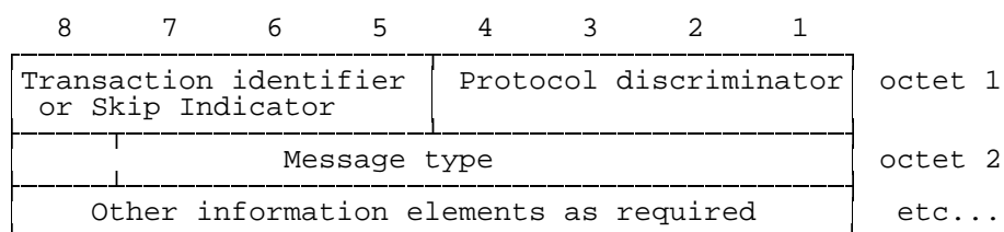
Figure 10.1/3GPP TS 04.08: General message organization example
