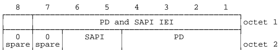
Figure 10.8qua/3GPP TS 04.08: PD and SAPI information element
