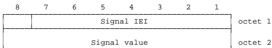
Figure 10.90/3GPP TS 04.08: Signal information element
