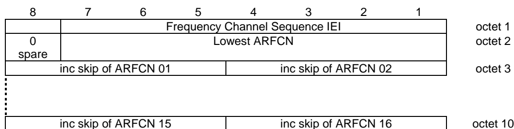
Figure 10.5.2.12.1/3GPP TS 04.18: Frequency Channel Sequence information element
