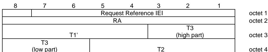
Figure 10.5.2.30.1/3GPP TS 04.18: Request Reference information element
