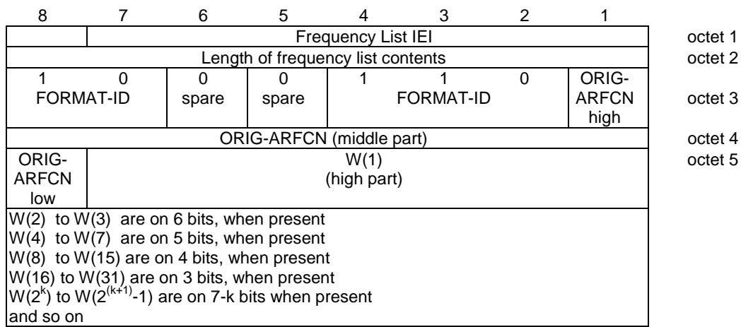
Figure 10.5.2.13.6.1: Frequency List information element (Range 128 format)
