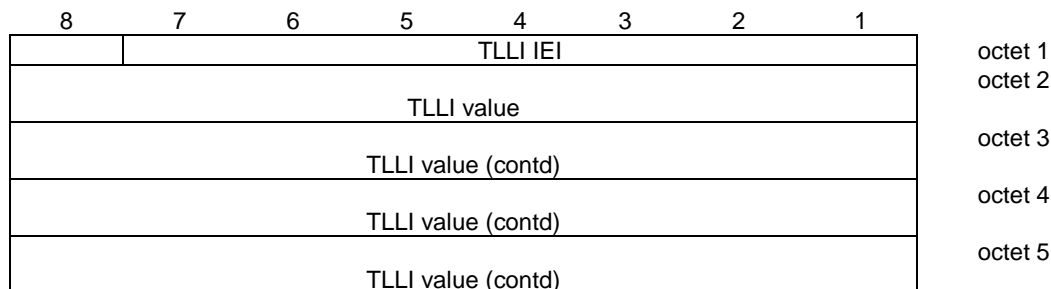
Figure 10.5.69/3GPP TS 04.18 TLLI information element
