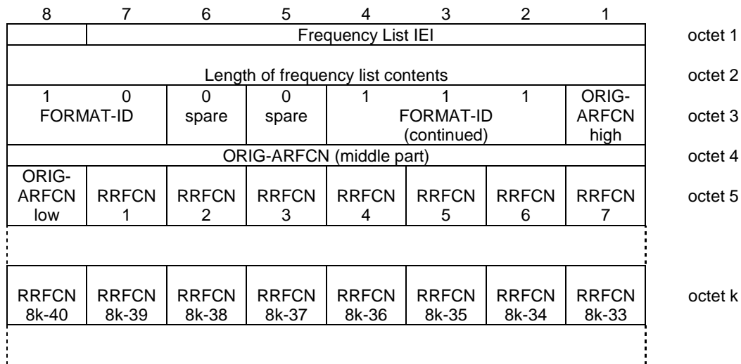
Figure 10.5.40/3GPP TS 04.18 Frequency List information element, variable bit map format
