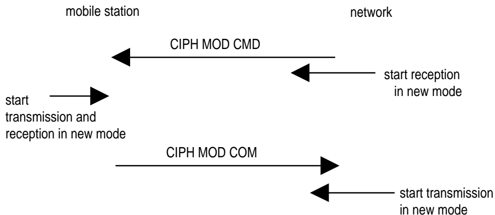
Figure 3.3/3GPP TS 04.18: Ciphering mode setting sequence
