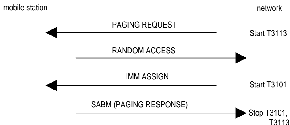
Figure 3.2/3GPP TS 04.18 Paging sequence
