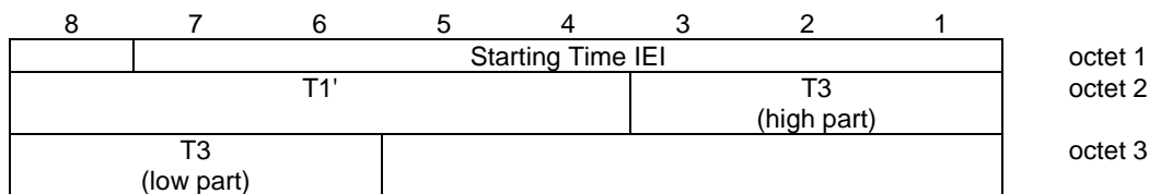
Figure 10.5.65/3GPP TS 04.18 Starting Time information element
