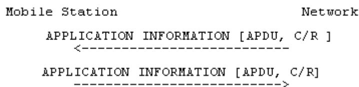
Figure 3.4/3GPP TS 04.18: Application Information Transfer without segmentation
