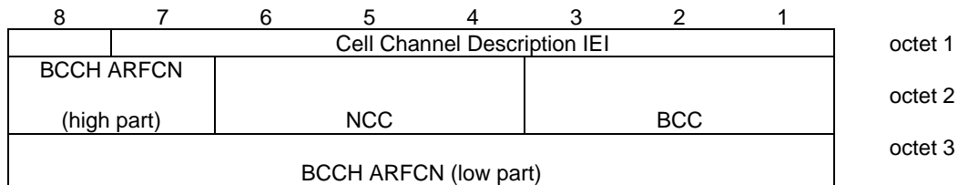
Figure 10.5.20/3GPP TS 04.18 Cell Description information element
