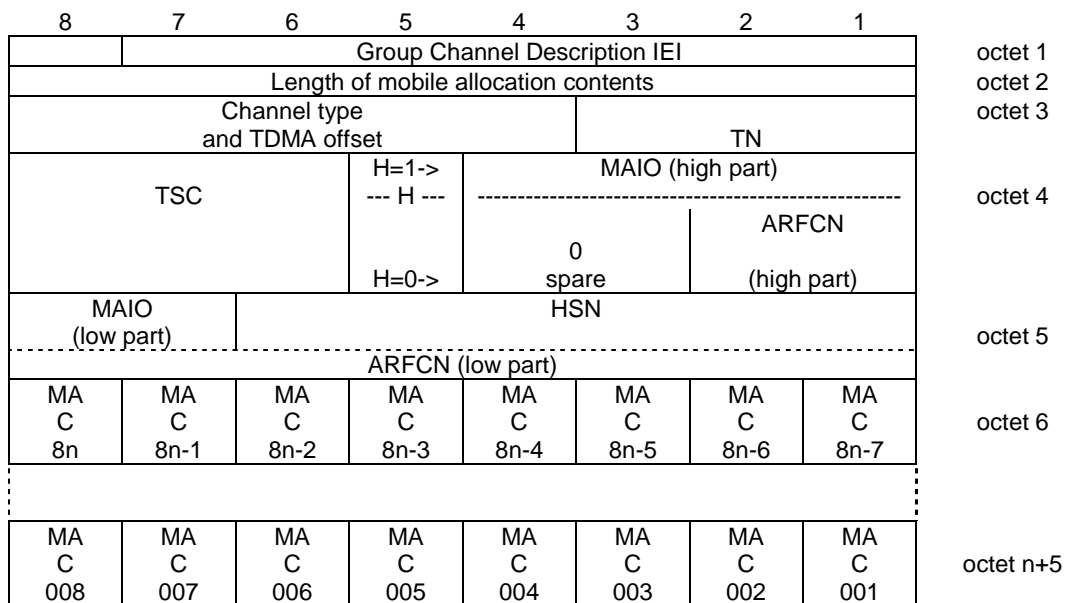
Figure 10.5.41/3GPP TS 04.18 Group Channel Description information element
