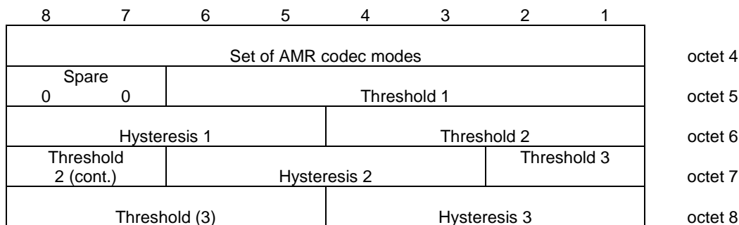
Figure 10.5.2.47d/3GPP TS 04.18: Parameters for multirate speech field for the MR version 1 when a set of four modes is chosen
