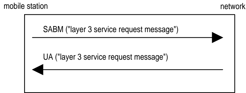
Figure 3.1/3GPP TS 04.18 Service request and contention resolution
