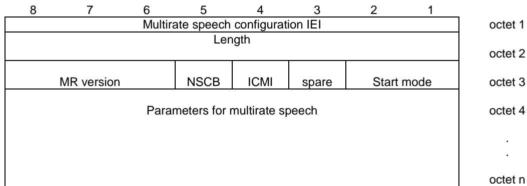
Figure 10.5.2.47/3GPP TS 04.18 MultiRate configuration information element
