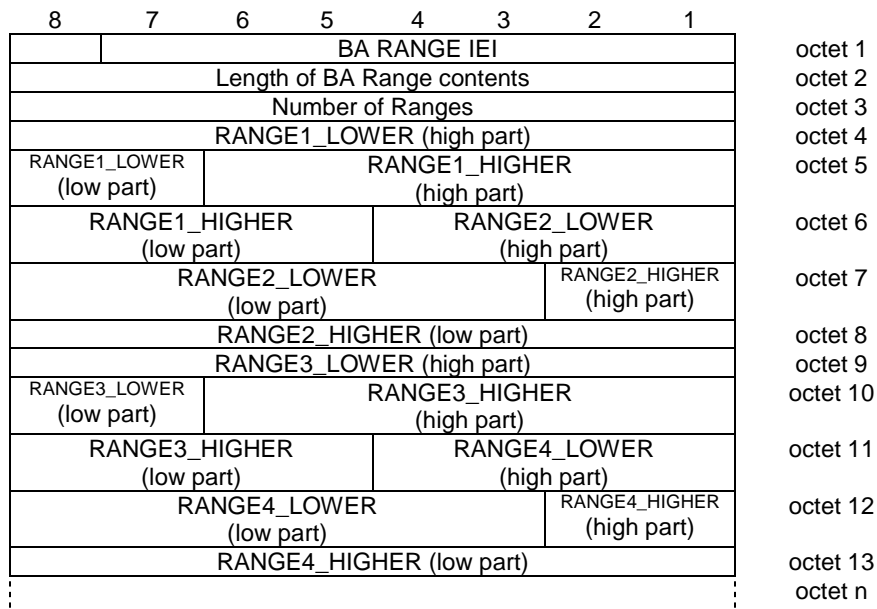
Figure 10.5.12/3GPP TS 04.18 BA RANGE information element
