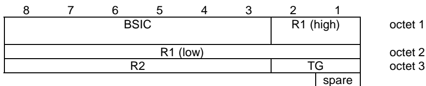
Figure 9.3b/3GPP TS 04.18: COMPACT Frame synchronization information element
