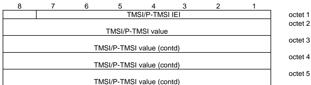
Figure 10.5.70/3GPP TS 04.18 TMSI/P-TMSI information element
