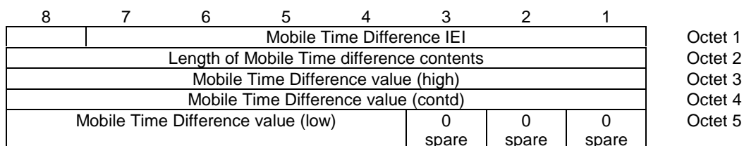
Figure 10.5.50/3GPP TS 04.18 Mobile Time Difference information element
