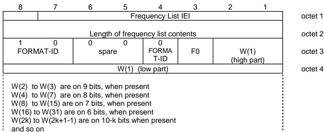
Figure 10.5.36/3GPP TS 04.18 Frequency List information element (Range 1024 format)
