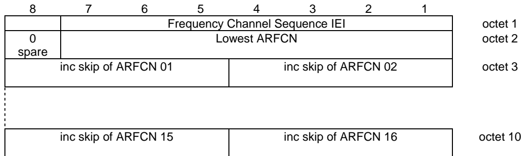
Figure 10.5.34/3GPP TS 04.18 Frequency Channel Sequence information element
