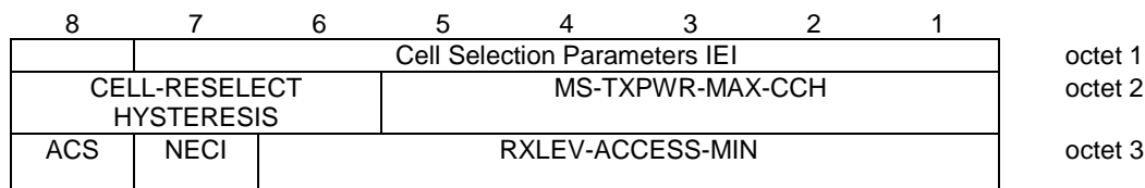
Figure 10.5.23/3GPP TS 04.18 Cell Selection Parameters information element
