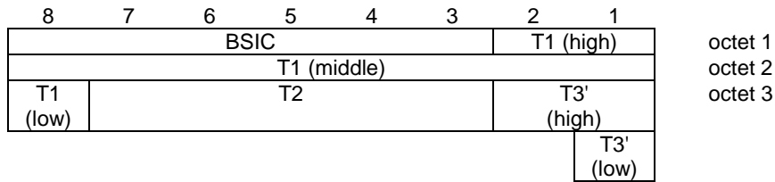
Figure 9.3a/3GPP TS 04.18: Frame synchronization information element
