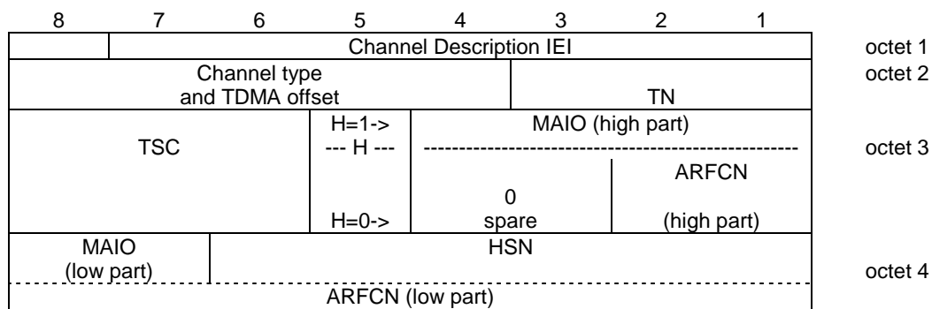
Figure 10.5.26/3GPP TS 04.18 Channel Description 2 information element
