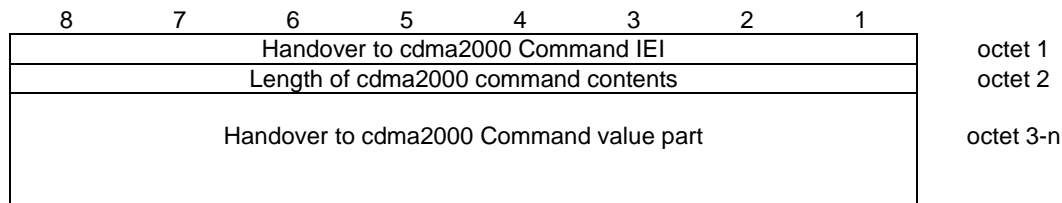
Figure 10.5.2.52/3GPP TS 04.18: Handover to cdma2000 Command information element
