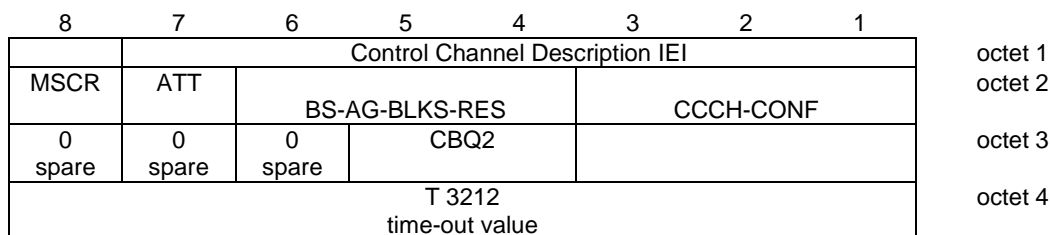
Figure 10.5.33/3GPP TS 04.18 Control Channel Description information element
