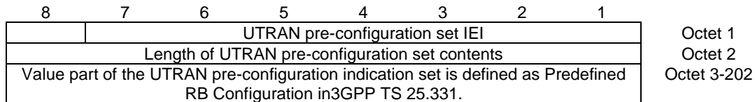
Figure 10.5.27/3GPP TS 04.18: UTRAN pre-configuration set information element
