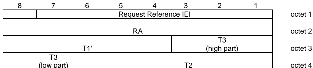
Figure 10.5.61/3GPP TS 04.18 Request Reference information element
