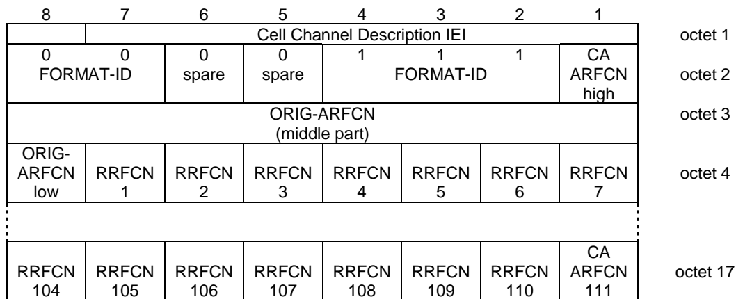
Figure 10.5.19/3GPP TS 04.18 Cell Channel Description information element, variable bit map format
