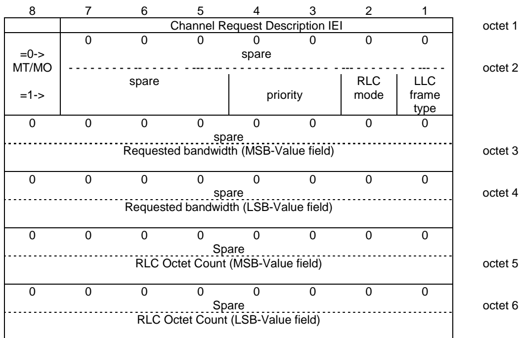
Figure 10.5.30/3GPP TS 04.18 Channel Request Description information element
