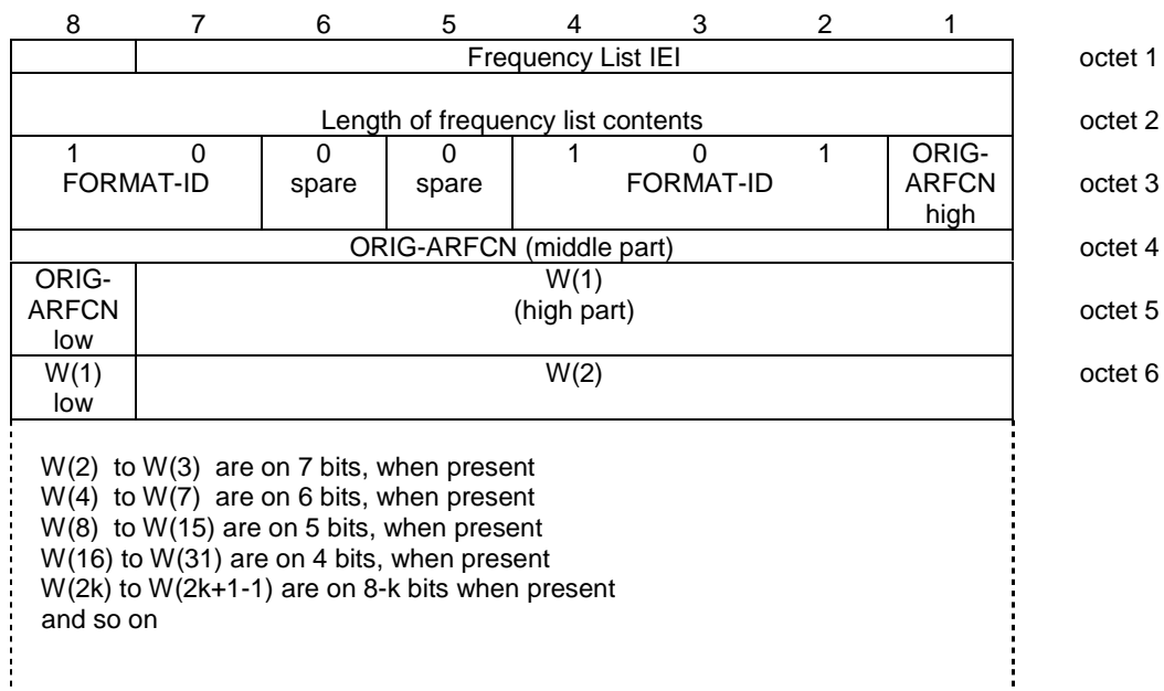
Figure 10.5.38/3GPP TS 04.18 Frequency List information element (Range 256 format)
