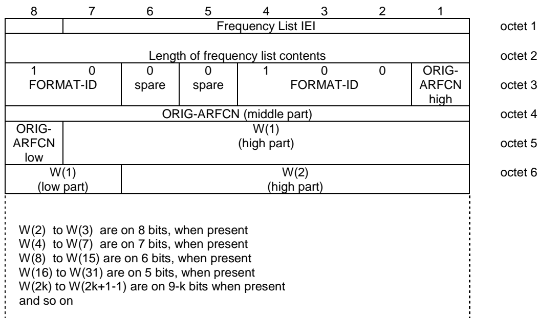
Figure 10.5.37/3GPP TS 04.18 Frequency List information element (Range 512 format)
