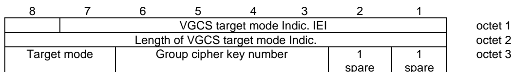
Figure 10.5.71/3GPP TS 04.18 VGCS target mode Indication information element
