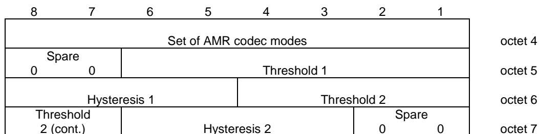
Figure 10.5.2.47c/3GPP TS 04.18: Parameters for multirate speech field for the MR version 1 when a set of three codec modes is chosen
