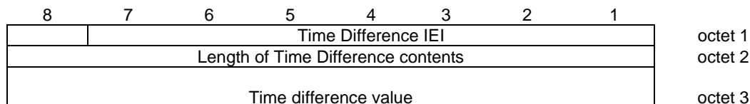
Figure 10.5.68/3GPP TS 04.18 Time Difference information element
