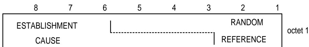
Figure 9.1/3GPP TS 04.18: CHANNEL REQUEST message content
