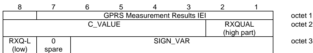
Figure 10.5.48/3GPP TS 04.18 GPRS Measurement Results information element
