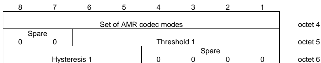
Figure 10.5.2.47b/3GPP TS 04: Parameters for multirate speech field for the MR version 1 when a set with two codec modes is chosen
