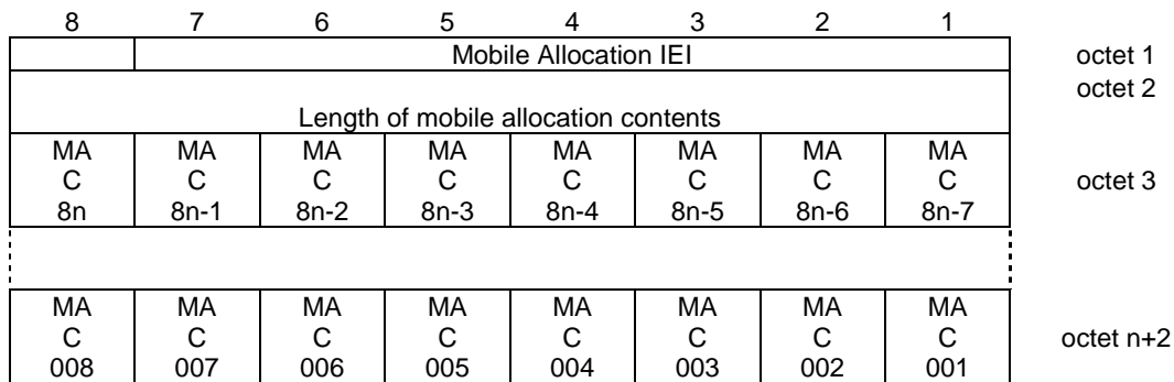
Figure 10.5.49/3GPP TS 04.18 Mobile Allocation information element
