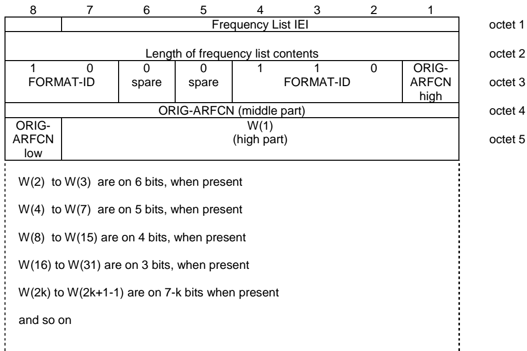
Figure 10.5.39/3GPP TS 04.18 Frequency List information element (Range 128 format)
