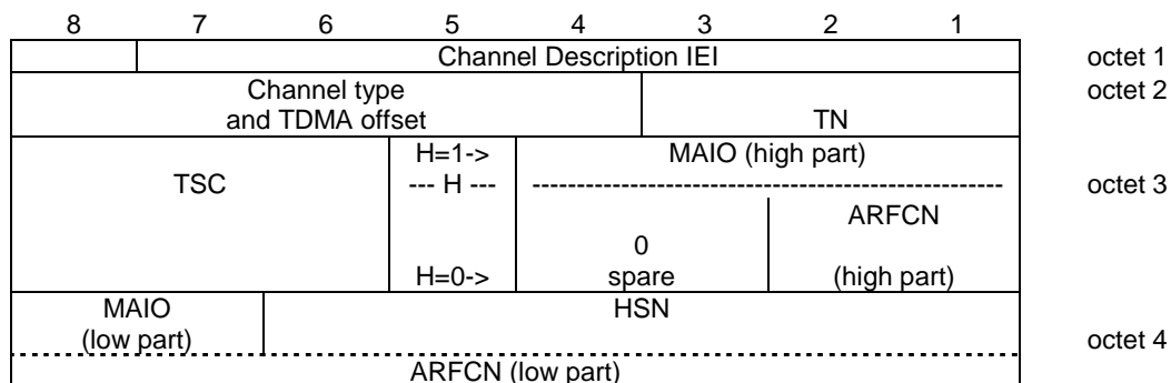
Figure 10.5.25/3GPP TS 04.18 Channel Description information element
