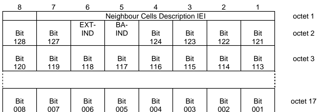
Figure 10.5.53/3GPP TS 04.18 Neighbour Cells Description information element
