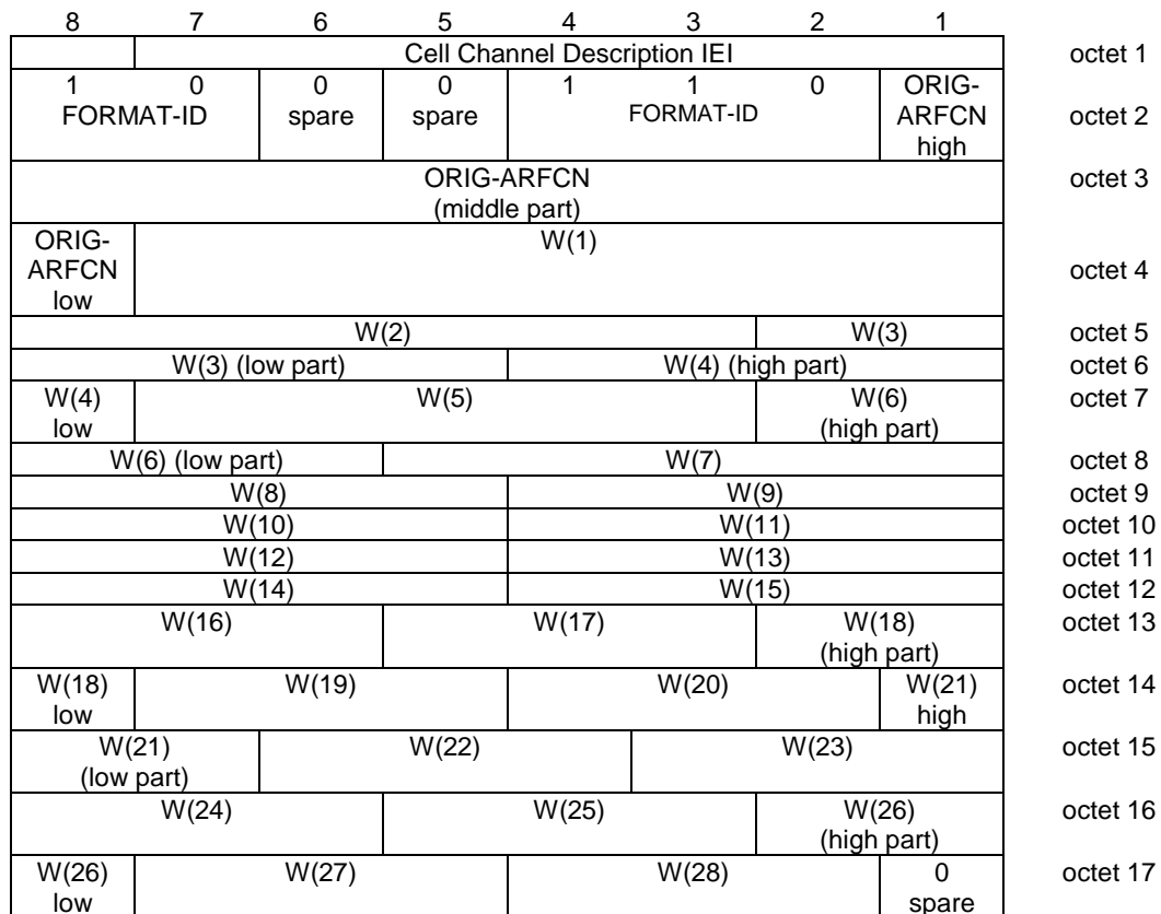
Figure 10.5.18/3GPP TS 04.18 Cell Channel Description information element, range 128 format
