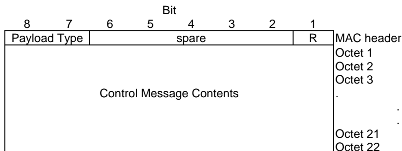
Figure 8: Uplink RLC/MAC control block together with its MAC header
