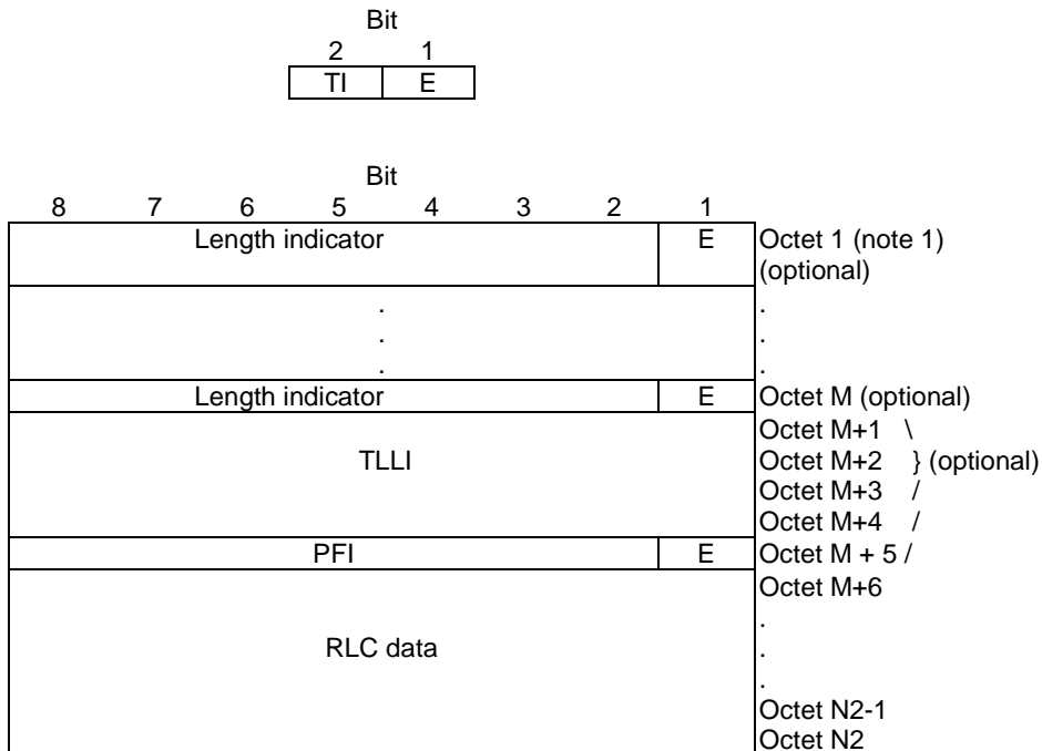
Figure 11: Uplink EGPRS RLC data block
