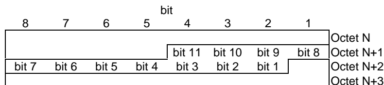
Figure 18: Field mapping within RLC/MAC messages
