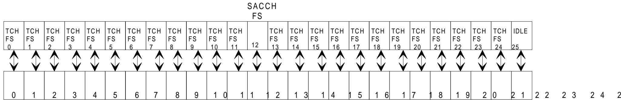
Figure 7a: TDMA frame mapping for TCH/FS + SACCH/FS
