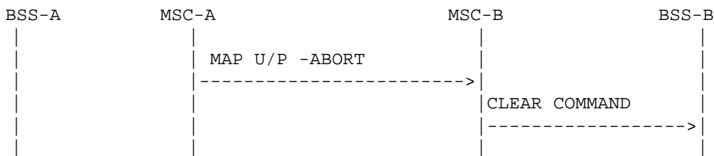
Figure 10: Signalling for Basic Inter-MSC Handover completion (Negative outcome)
