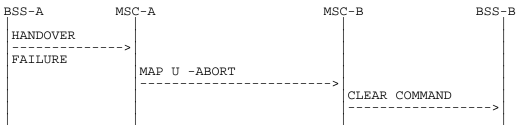
Figure 7: Signalling for Basic Inter-MSC Handover execution (Negative outcomes)
