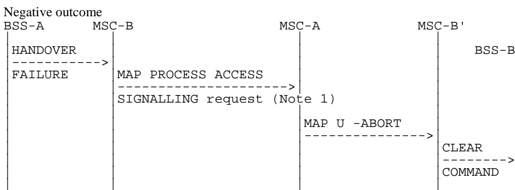
Figure 20: Signalling for Subsequent Inter-MSC Handover to third MSC (MSC-B') completion (Unsuccessful completion of the procedure)
