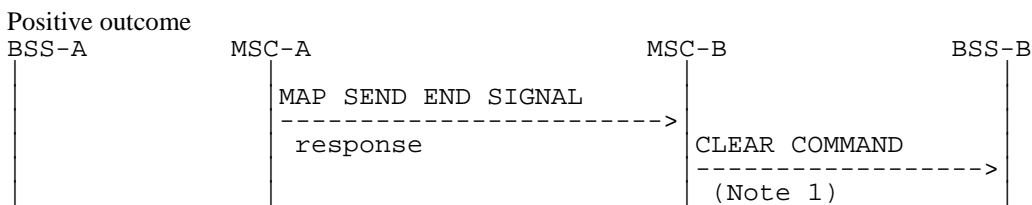
Figure 8: Signalling for Basic Inter-MSC Handover completion
