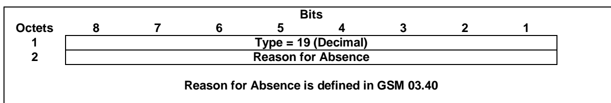
Figure 23A: MS Not Reachable Reason Information Element
