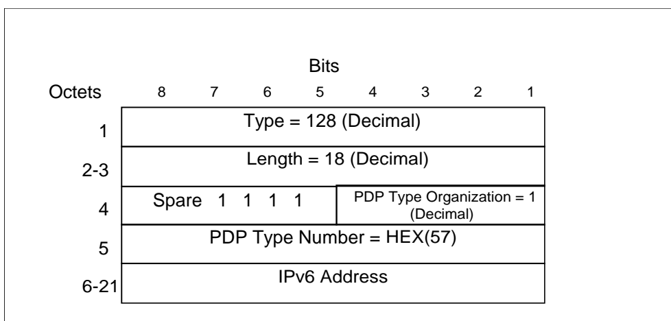
Figure 27: End User Address information element for IPv6
