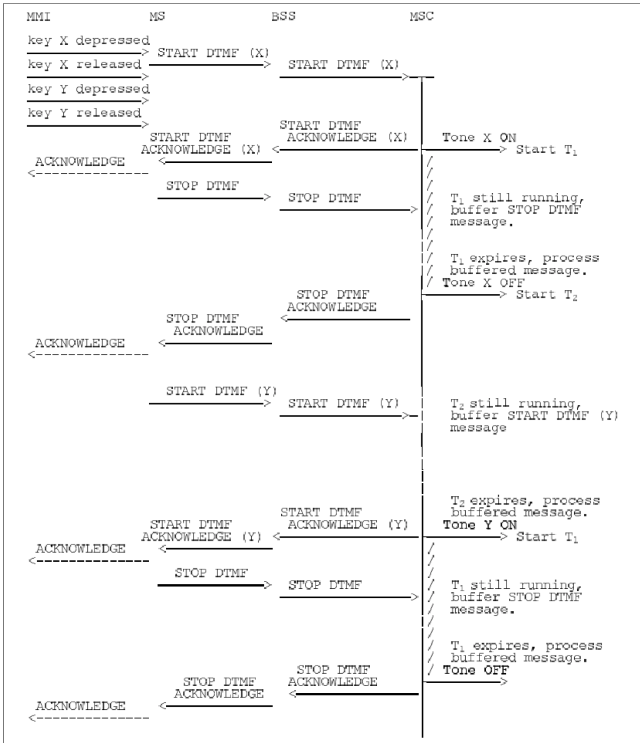
Figure 4: Two Single DTMF Transmissions, Short Gap Between Key Presses
