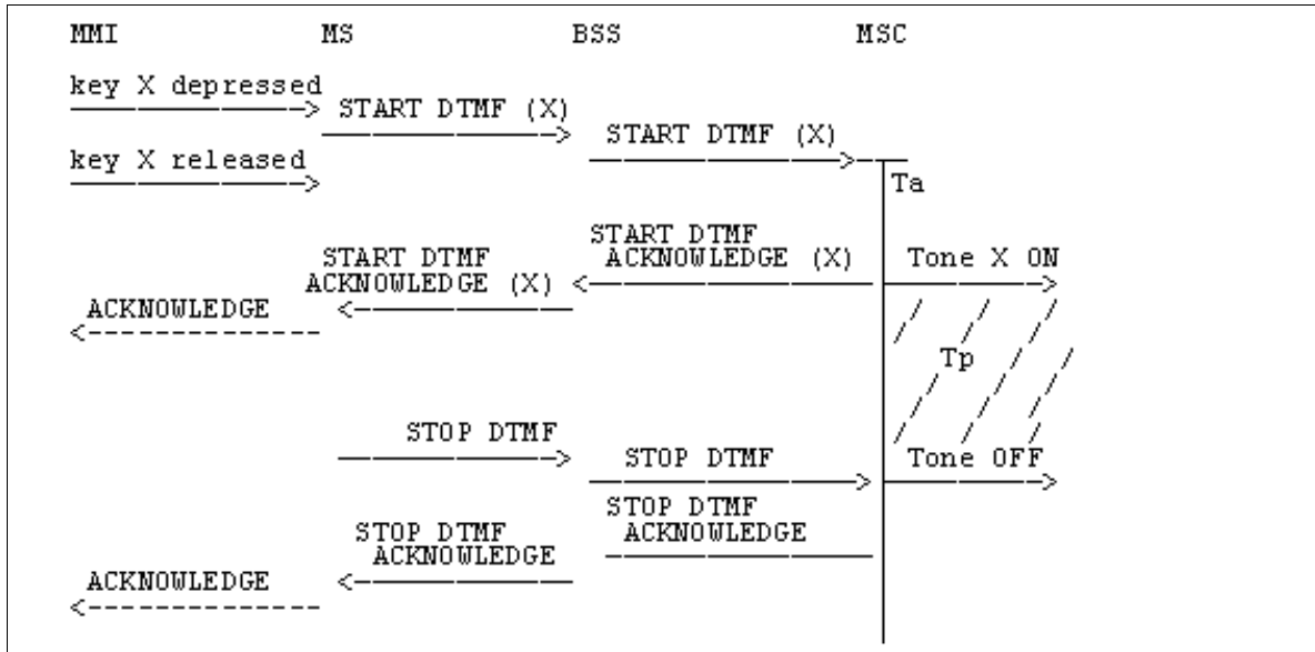
Figure 2: Single DTMF Transmission, Short Key Press
