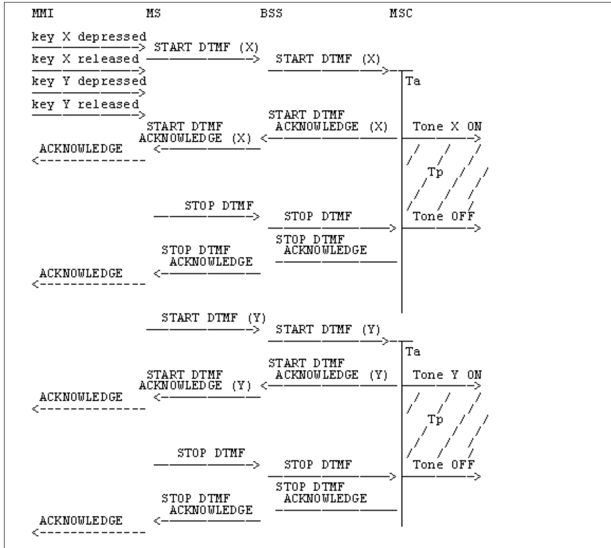
Figure 3: Two Single DTMF Transmission
