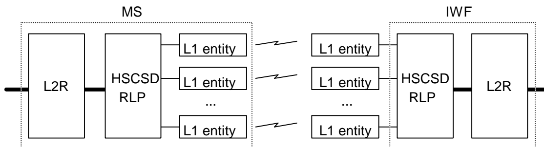
Figure 9a: The HSCSD concept in non-transparent mode
