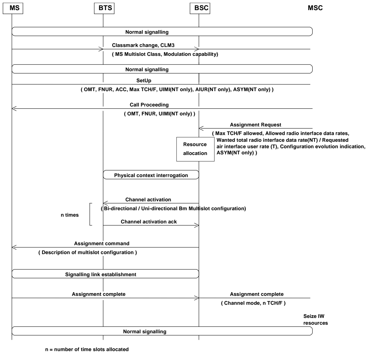
Figure 3: Mobile originated call establishment
