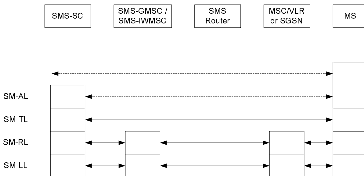
Figure 7: Protocol layer overview for the Short Message Service
