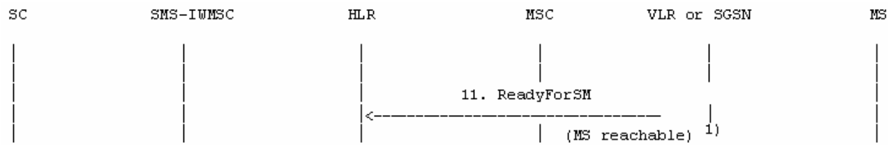
Figure 20a: The alert procedure when the MS becomes reachable, MNRf, MNRg or both are set and MCEF is not set
