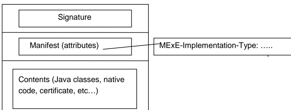
Figure 7: Signed packages
