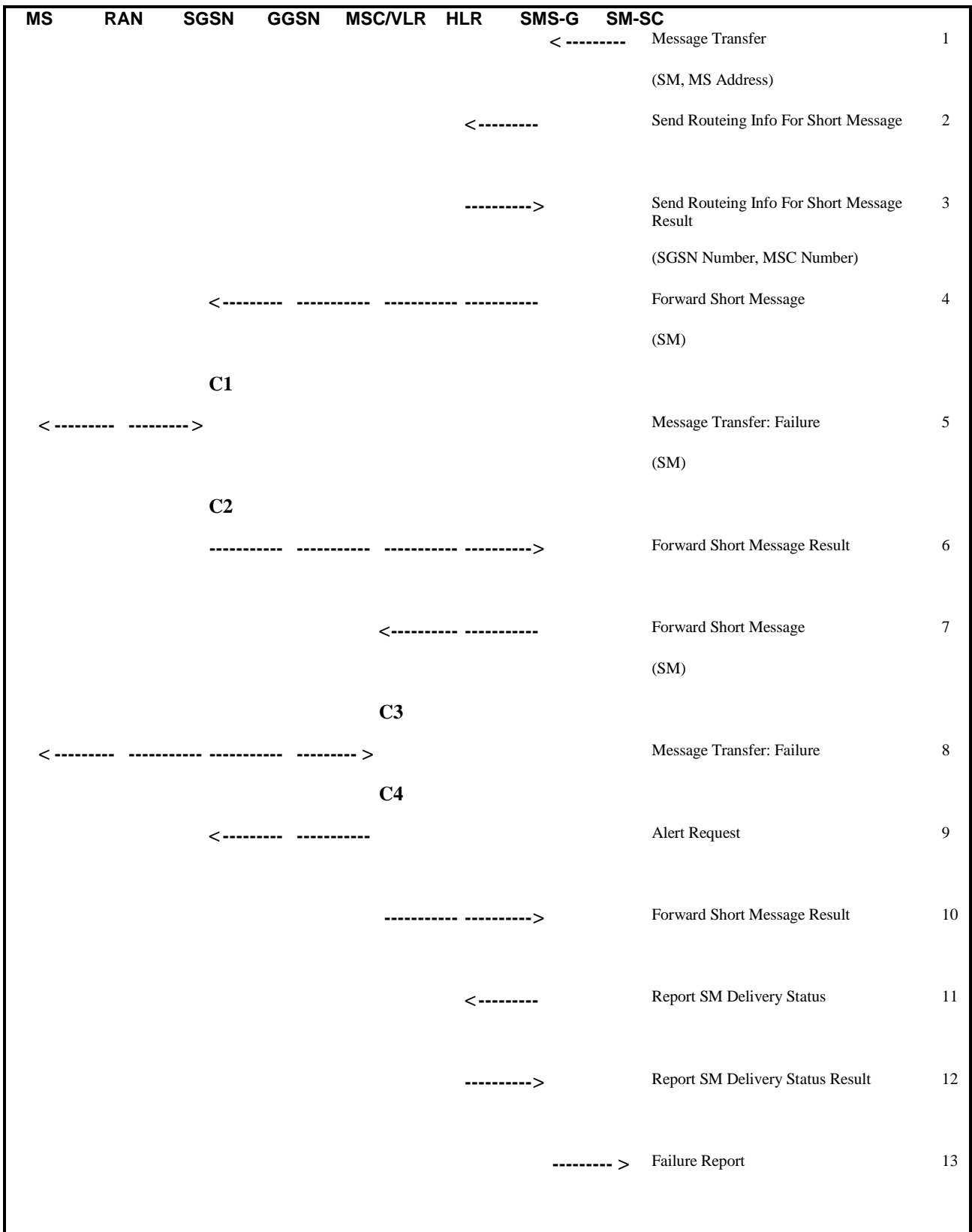
Figure 97: MT SMS Transfer, Unsuccessful
