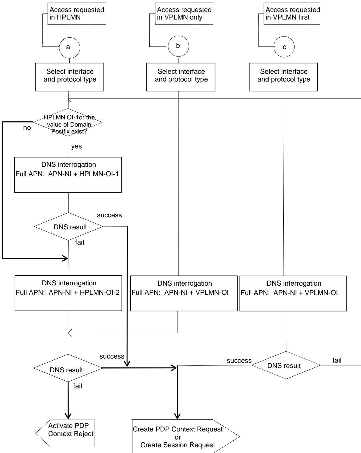
Figure A.6: SDL Diagram 6
