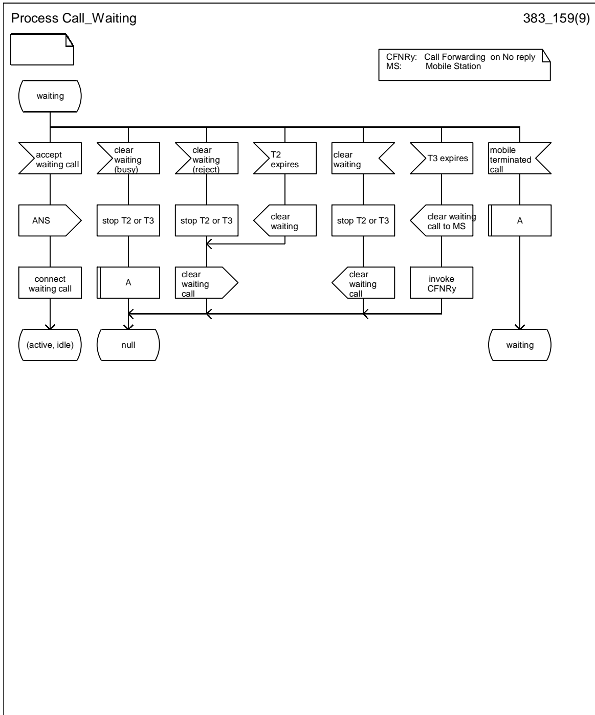
Figure 1.5 (sheet 9 of 10): Overall SDL diagram of call waiting
