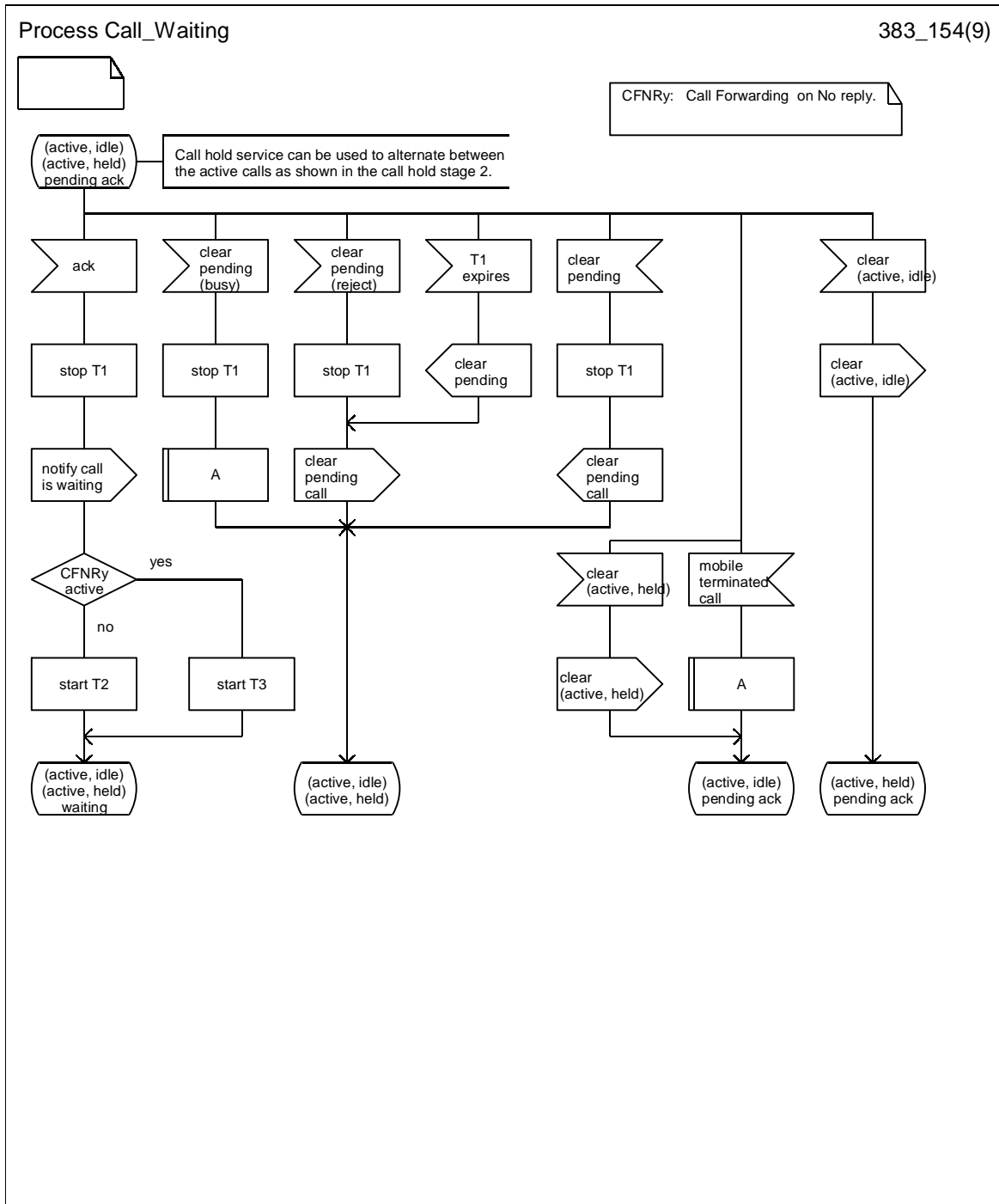
Figure 1.5 (sheet 4 of 10): Overall SDL diagram of call waiting
