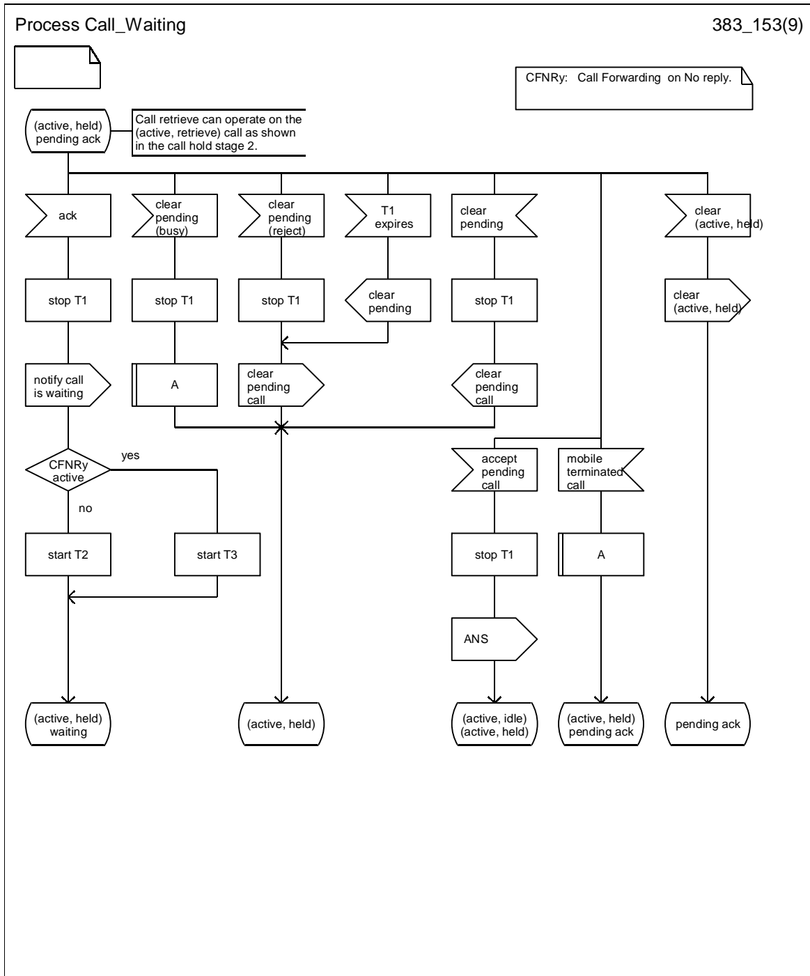
Figure 1.5 (sheet 3 of 10): Overall SDL diagram of call waiting
