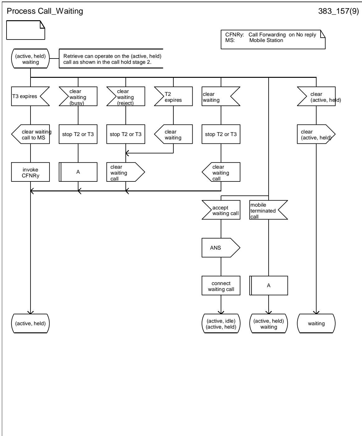
Figure 1.5 (sheet 7 of 10): Overall SDL diagram of call waiting
