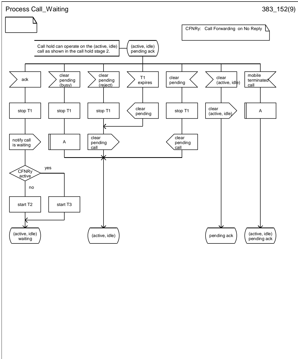
Figure 1.5 (sheet 2 of 10): Overall SDL diagram of call waiting
