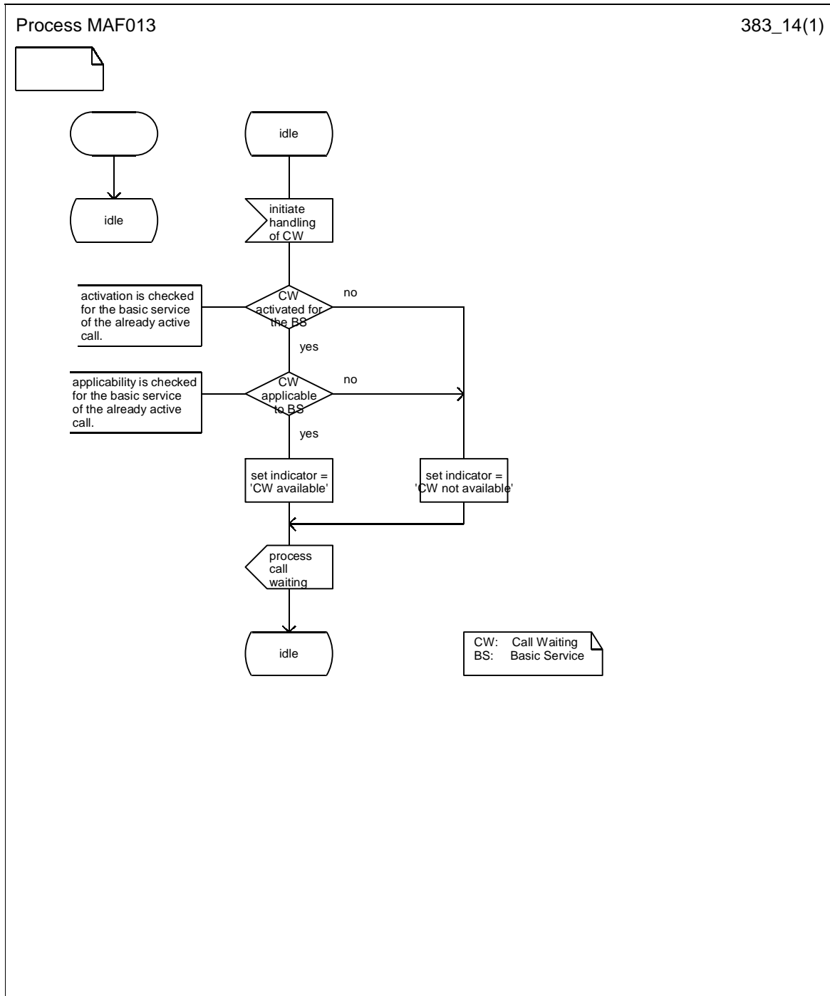
Figure 1.4: MAF013 Call waiting related authorisations examination (VLR)
