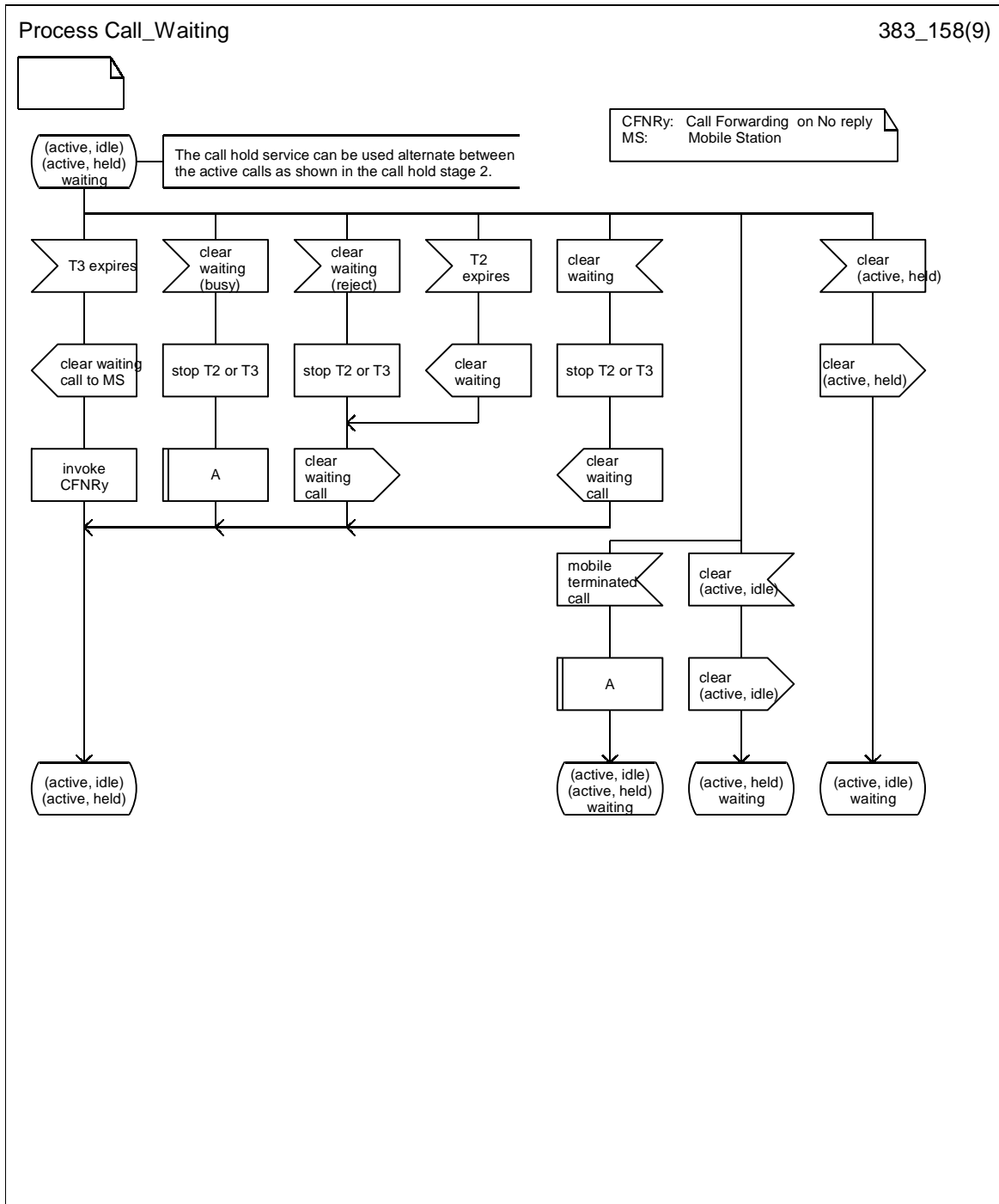
Figure 1.5 (sheet 8 of 10): Overall SDL diagram of call waiting
