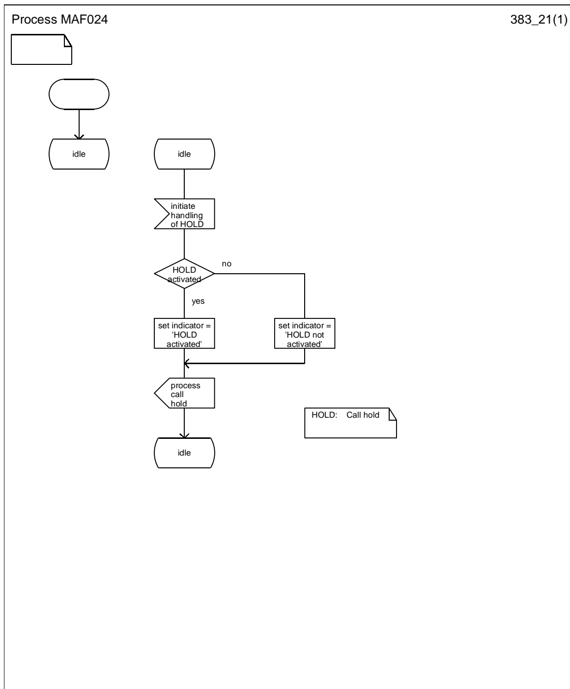
Figure 2.1: MAF024 Call hold related authorisations examination (VLR)
