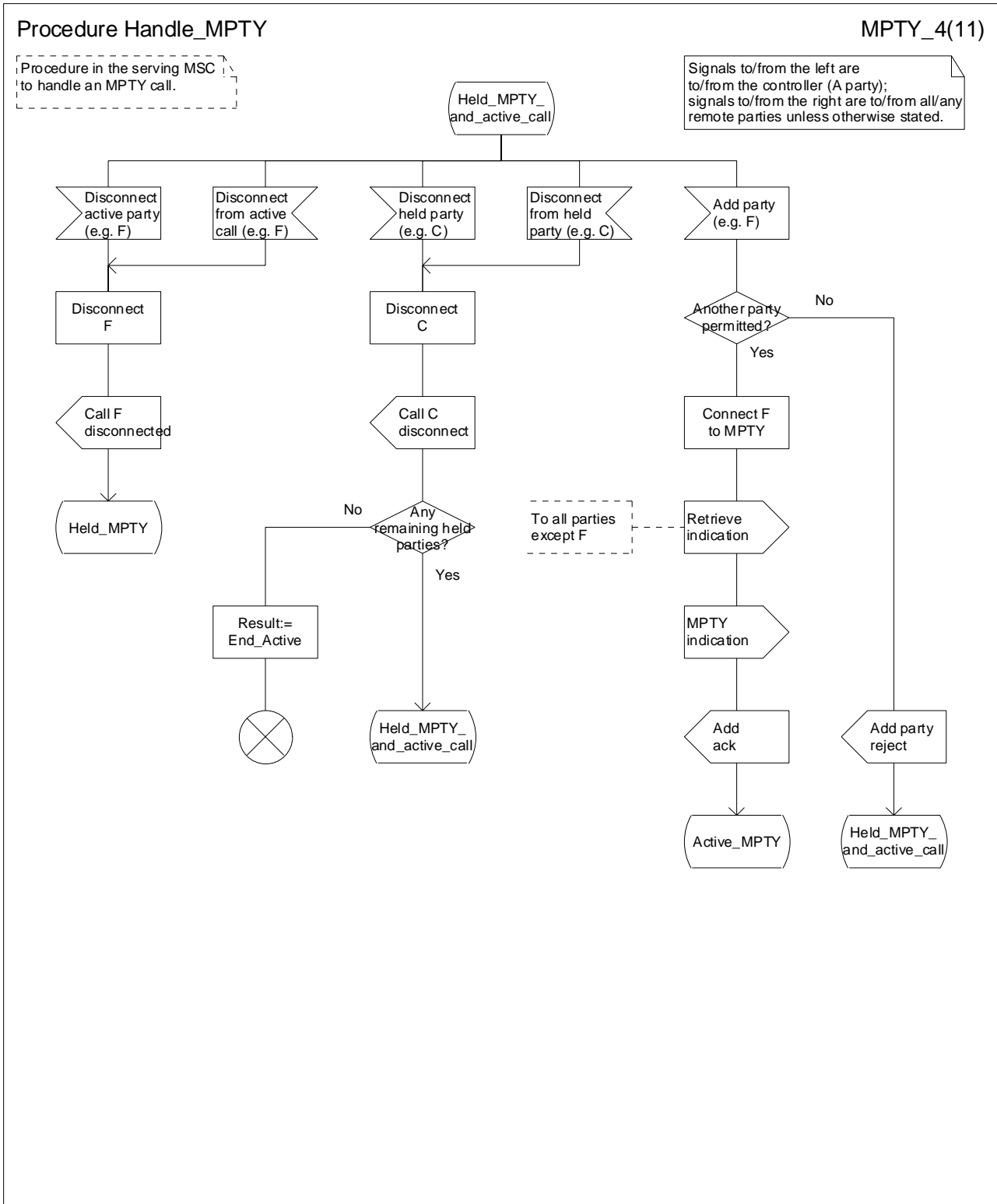
Figure 1.2 (sheet 4 of 11): Procedure Handle_MPTY
