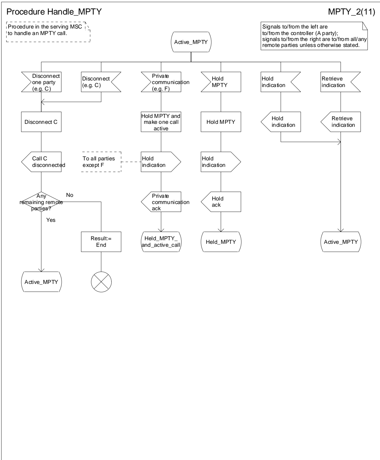
Figure 1.2 (sheet 2 of 11): Procedure Handle_MPTY
