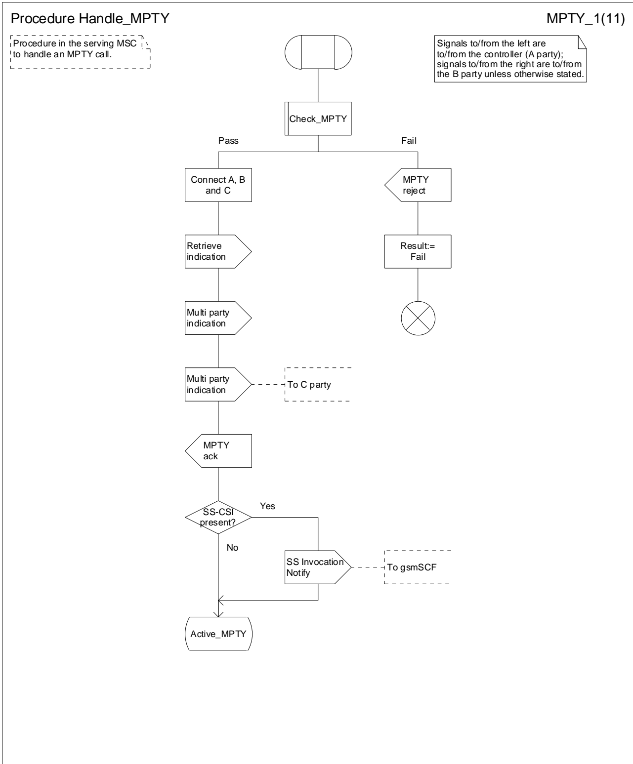
Figure 1.2 (sheet 1 of 11): Procedure Handle_MPTY
