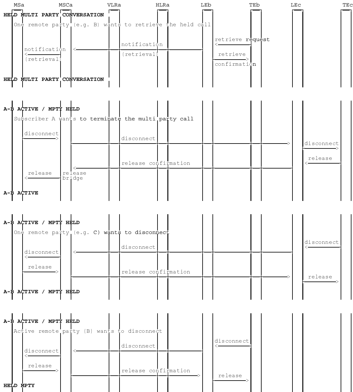
Figure 1.4 (sheet 5 of 7): Information flow for Multi Party service
