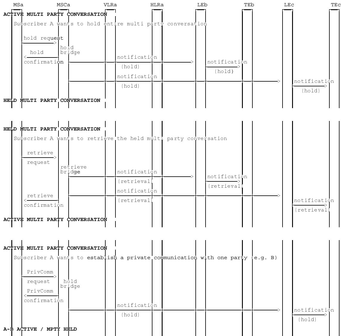
Figure 1.4 (sheet 3 of 7): Information flow for Multi Party service
