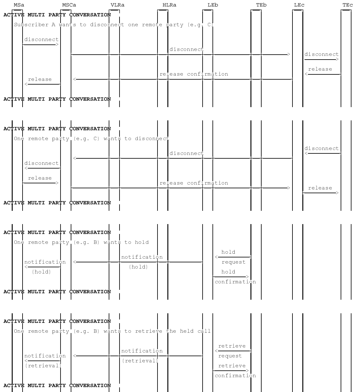
Figure 1.4 (sheet 2 of 7): Information flow for Multi Party service
