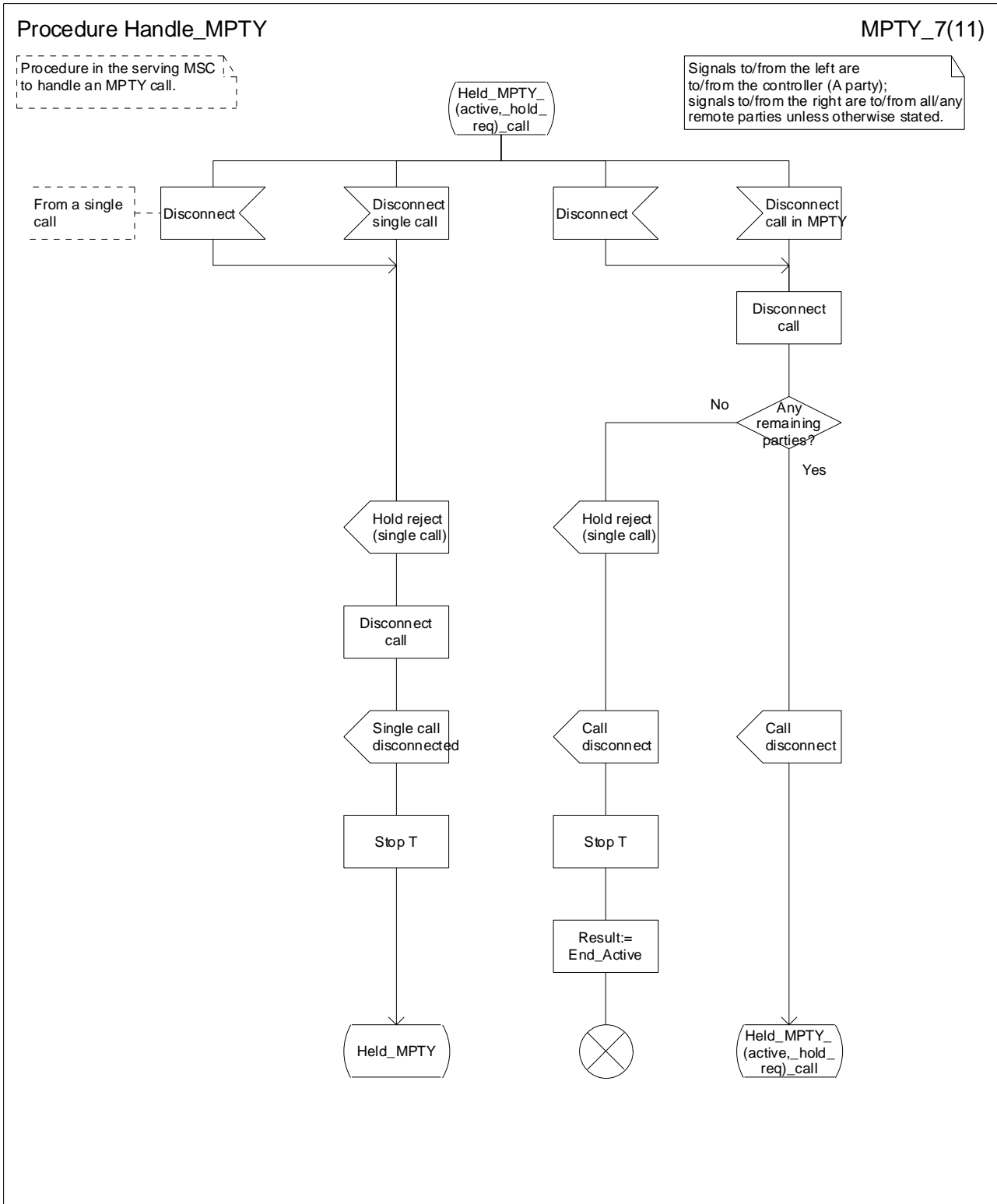
Figure 1.2 (sheet 7 of 11): Procedure Handle_MPTY
