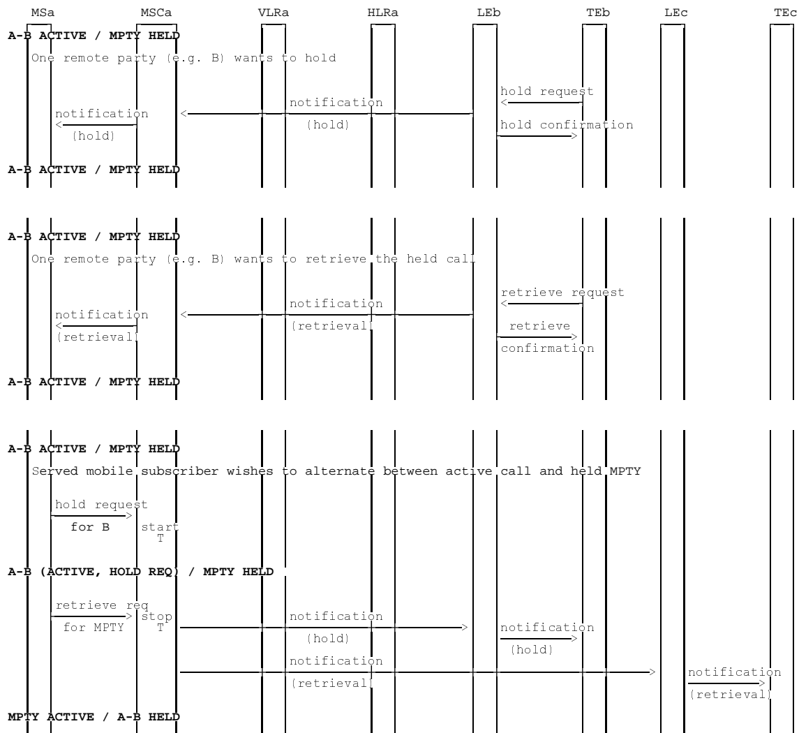
Figure 1.4 (sheet 7 of 7): Information flow for Multi Party service
