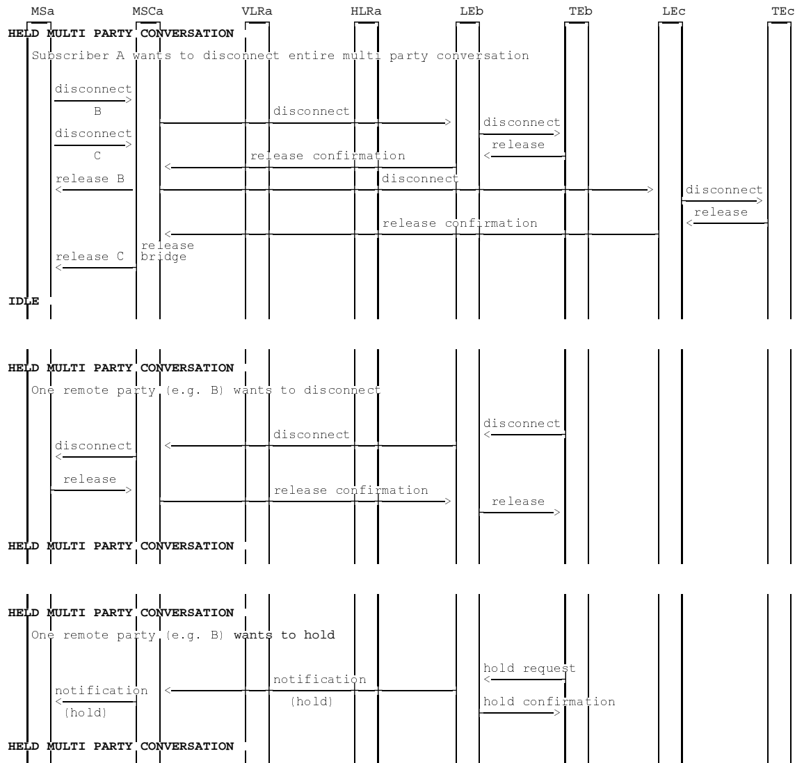
Figure 1.4 (sheet 4 of 7): Information flow for Multi Party service
