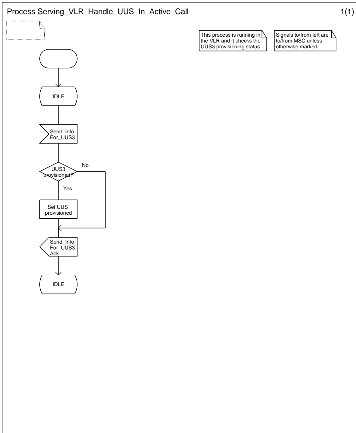
Figure 9.4.2.1: Process Serving_VLR_Handle_UUS_In_Active_Call
