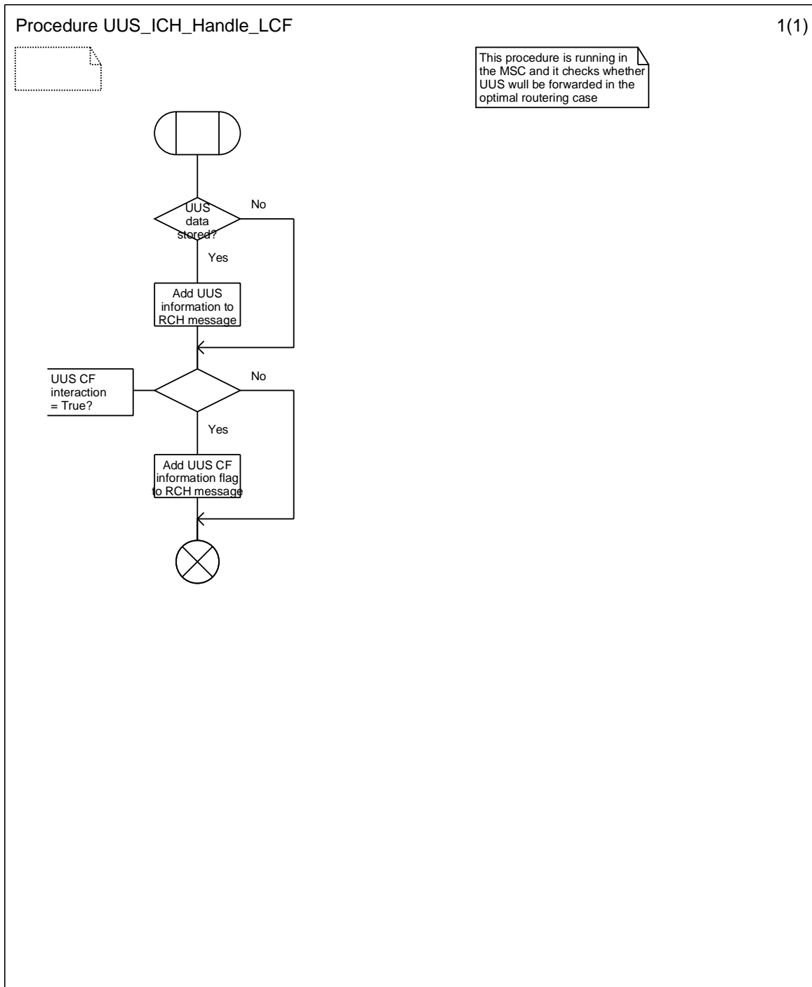
Figure 9.2.2.3: Procedure UUS_ICH_Handle_LCF
