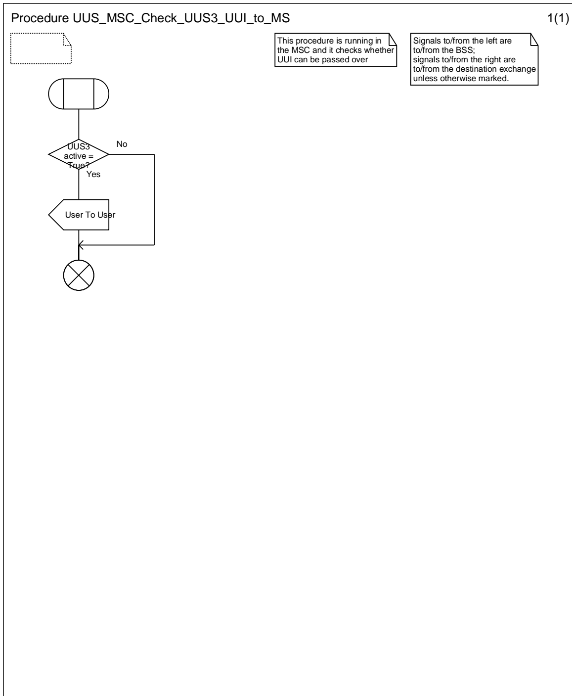
Figure 9.3.4: Procedure UUS_MSC_Check_UUS3_UUI_to_MS
