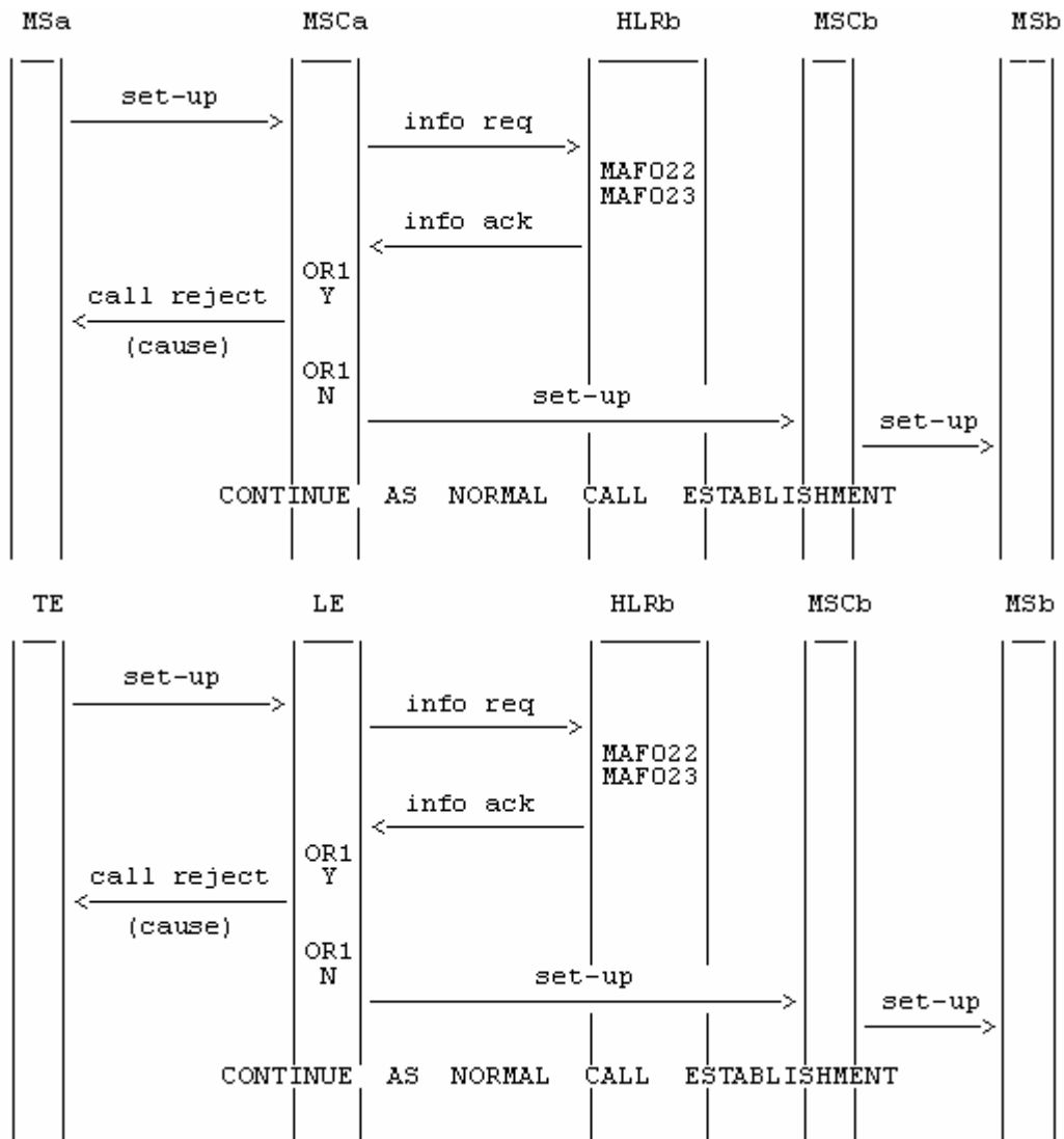
Figure 7.8: Information flow for barring of incoming calls
