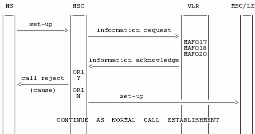
Figure 6.10: Information flow for barring of outgoing calls
