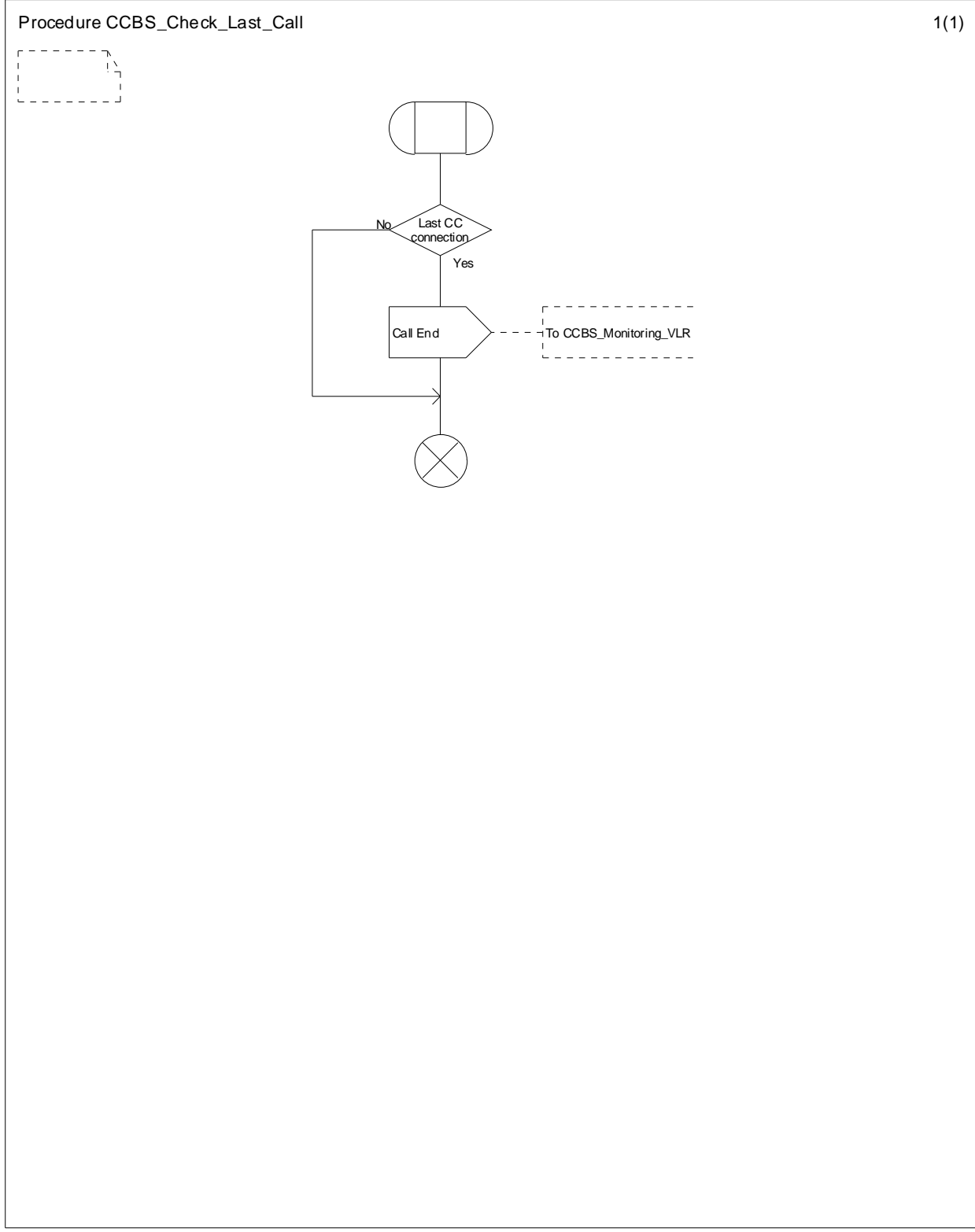
Figure 11.3.7: Procedure CCBS_Check_Last_Call
