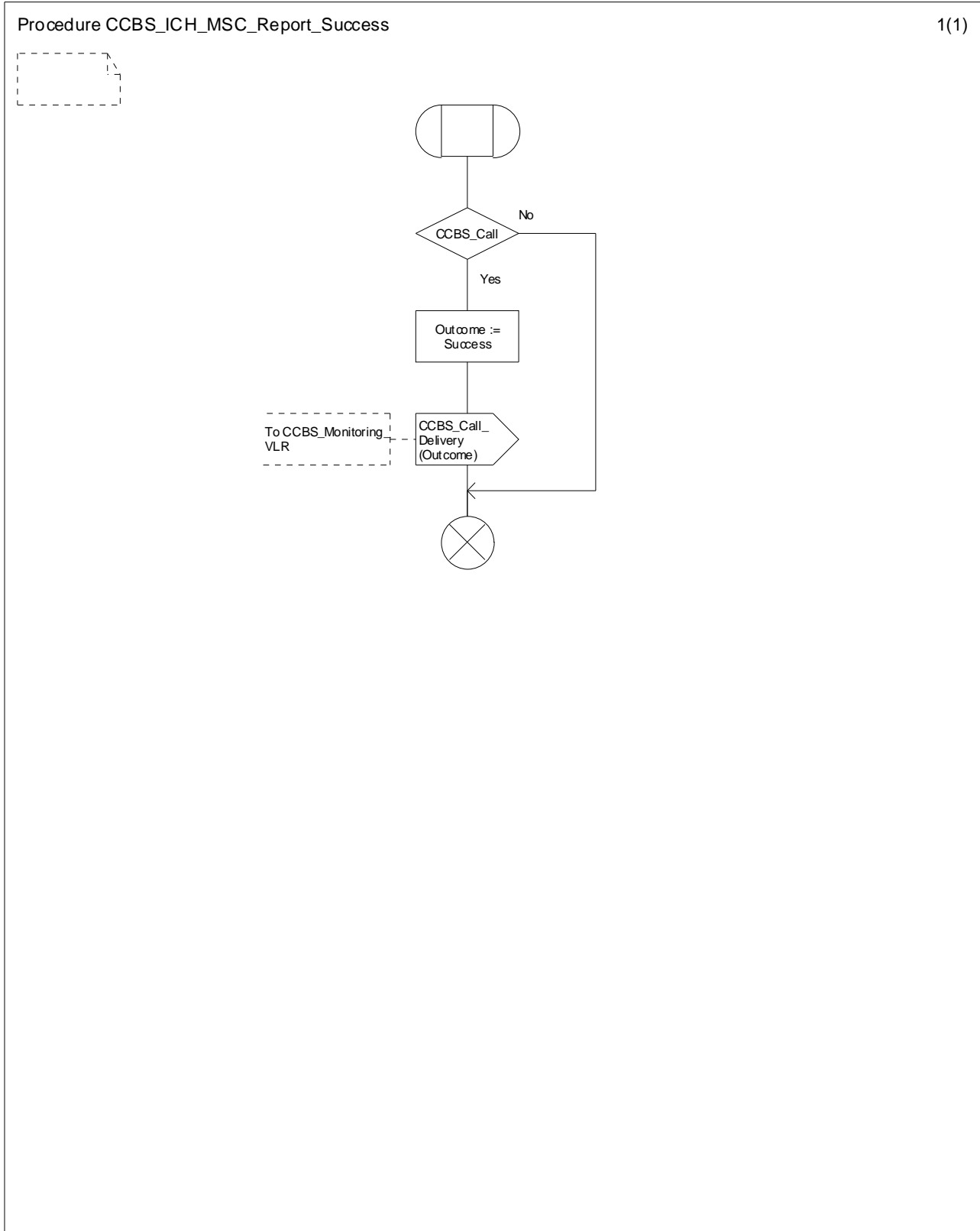
Figure 11.2.3.9: Procedure CCBS_ICH_MSC_Report_Success
