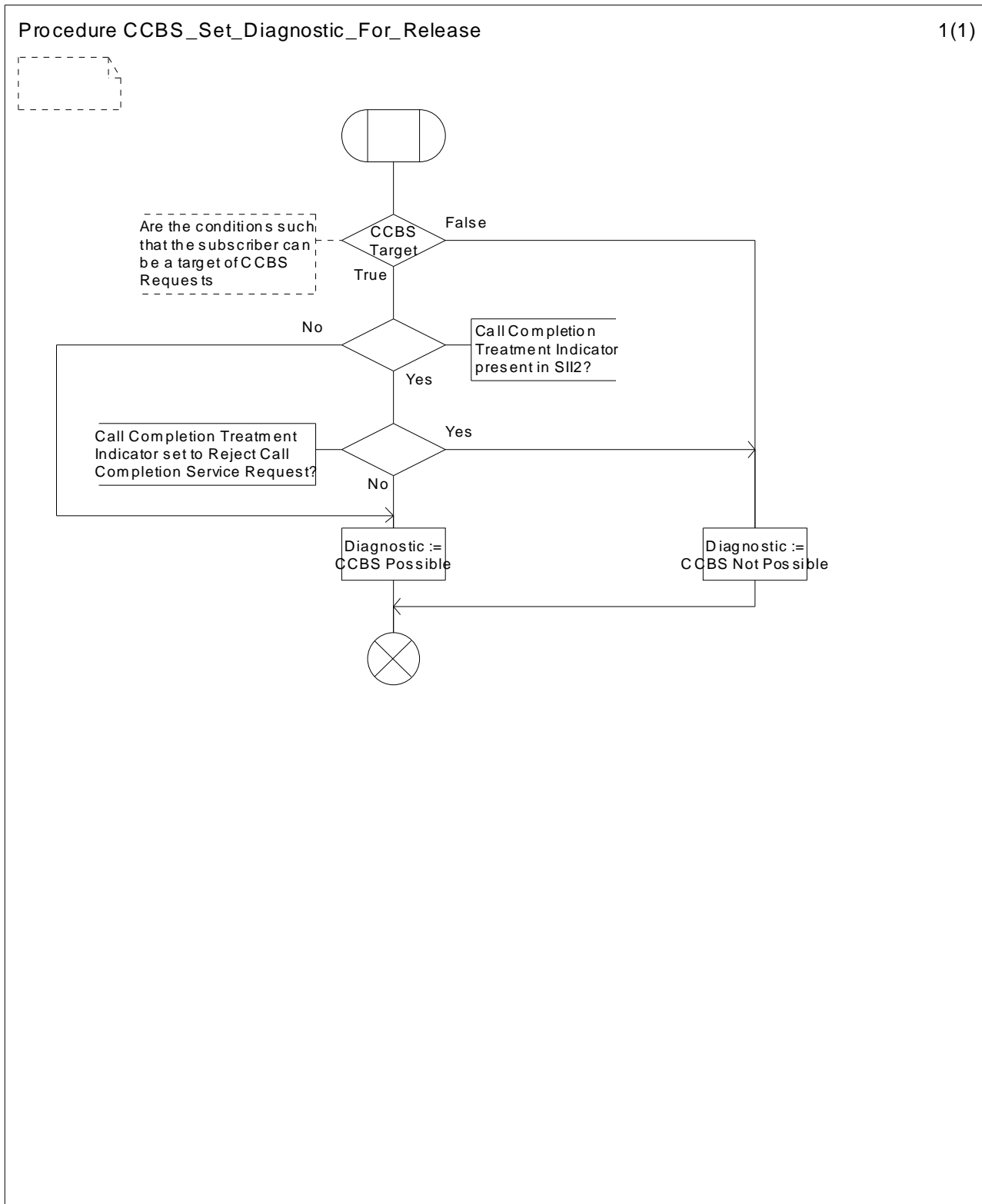
Figure 11.3.4: Procedure CCBS_Set_Diagnostic_For_Release
