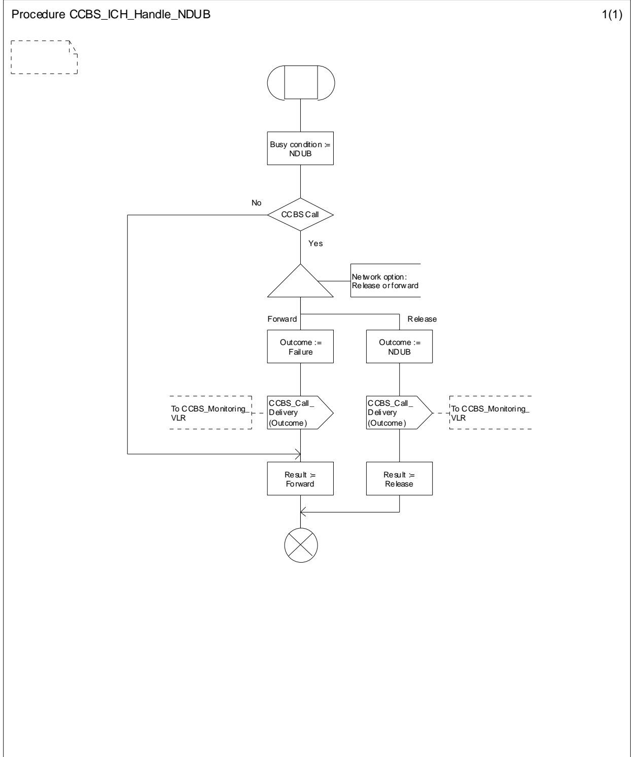
Figure 11.2.3.7: Procedure CCBS_ICH_Handle_NDUB
