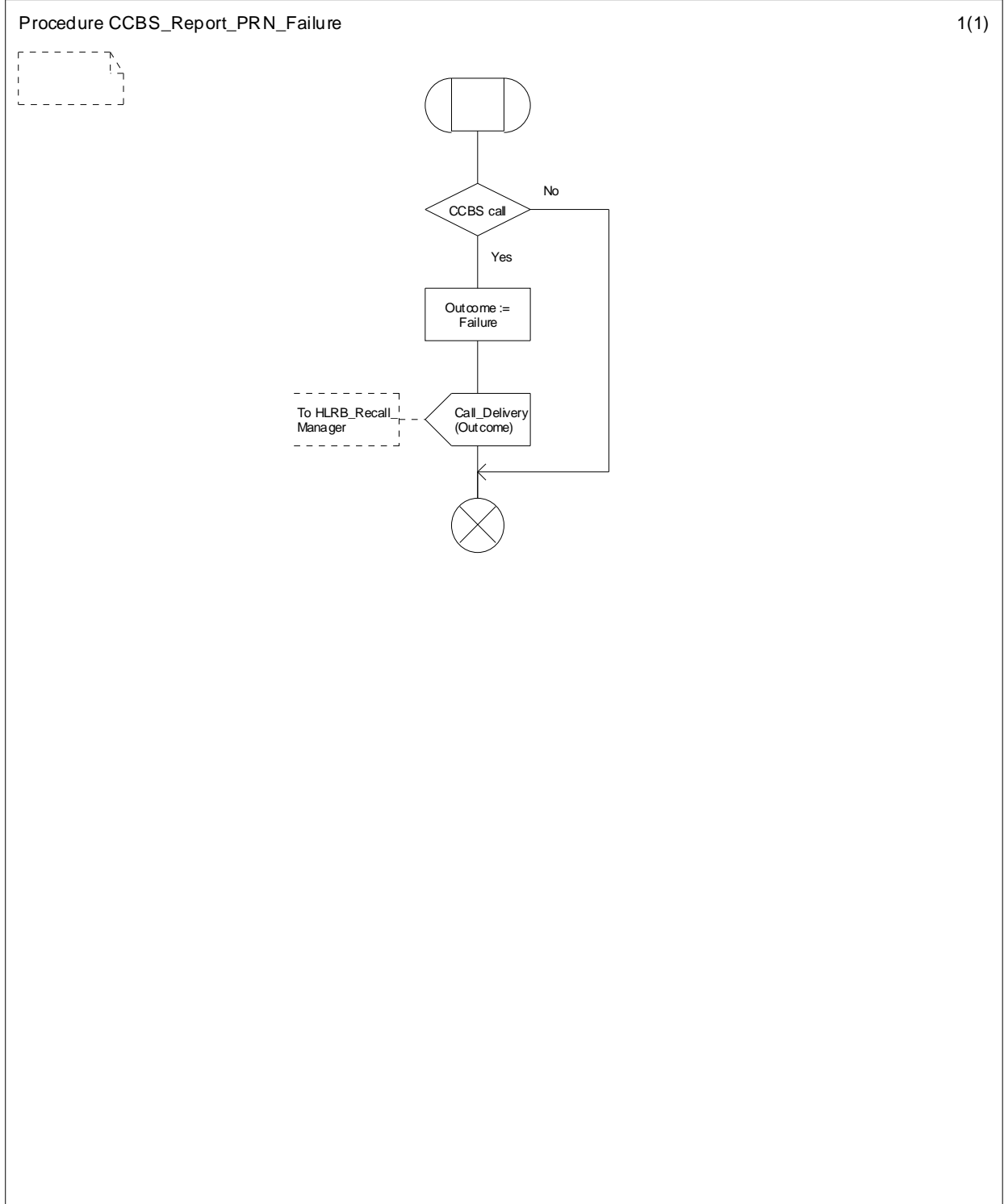
Figure 11.2.2.9: Procedure CCBS_Report_PRN_Failure
