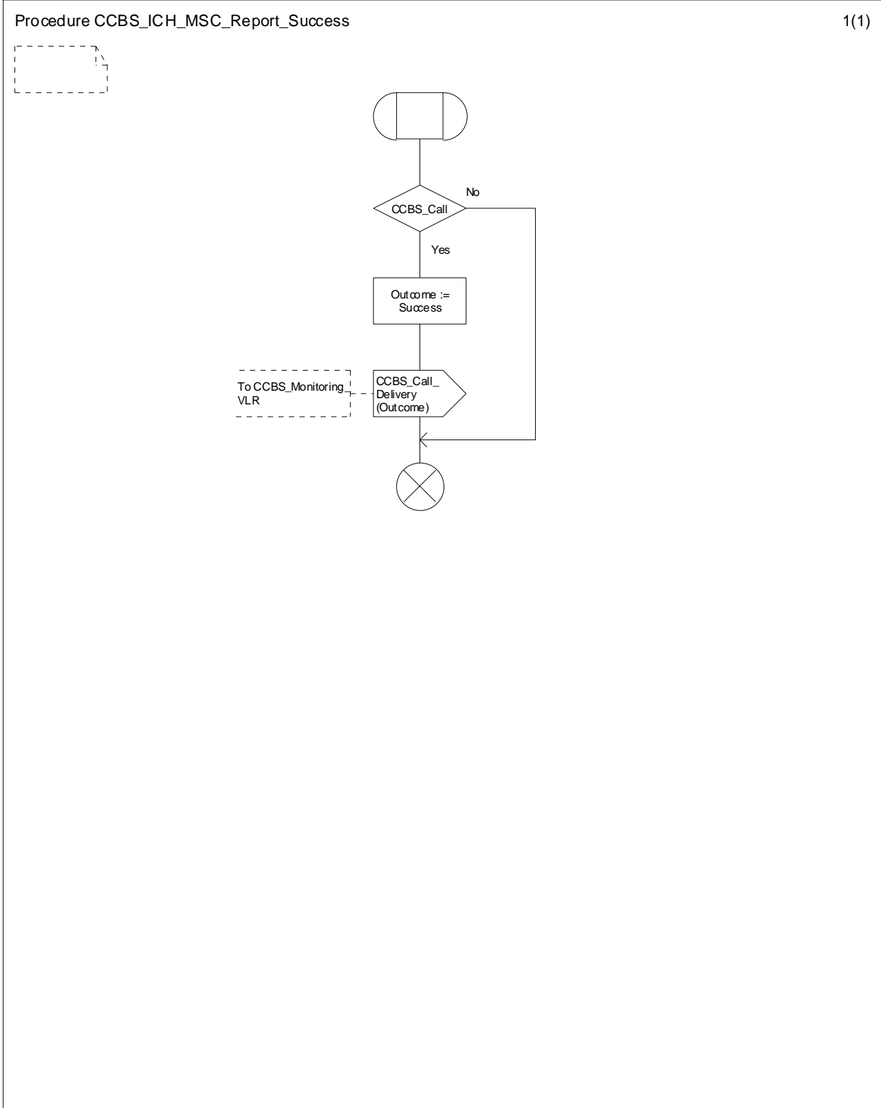
Figure 11.2.3.9: Procedure CCBS_ICH_MSC_Report_Success
