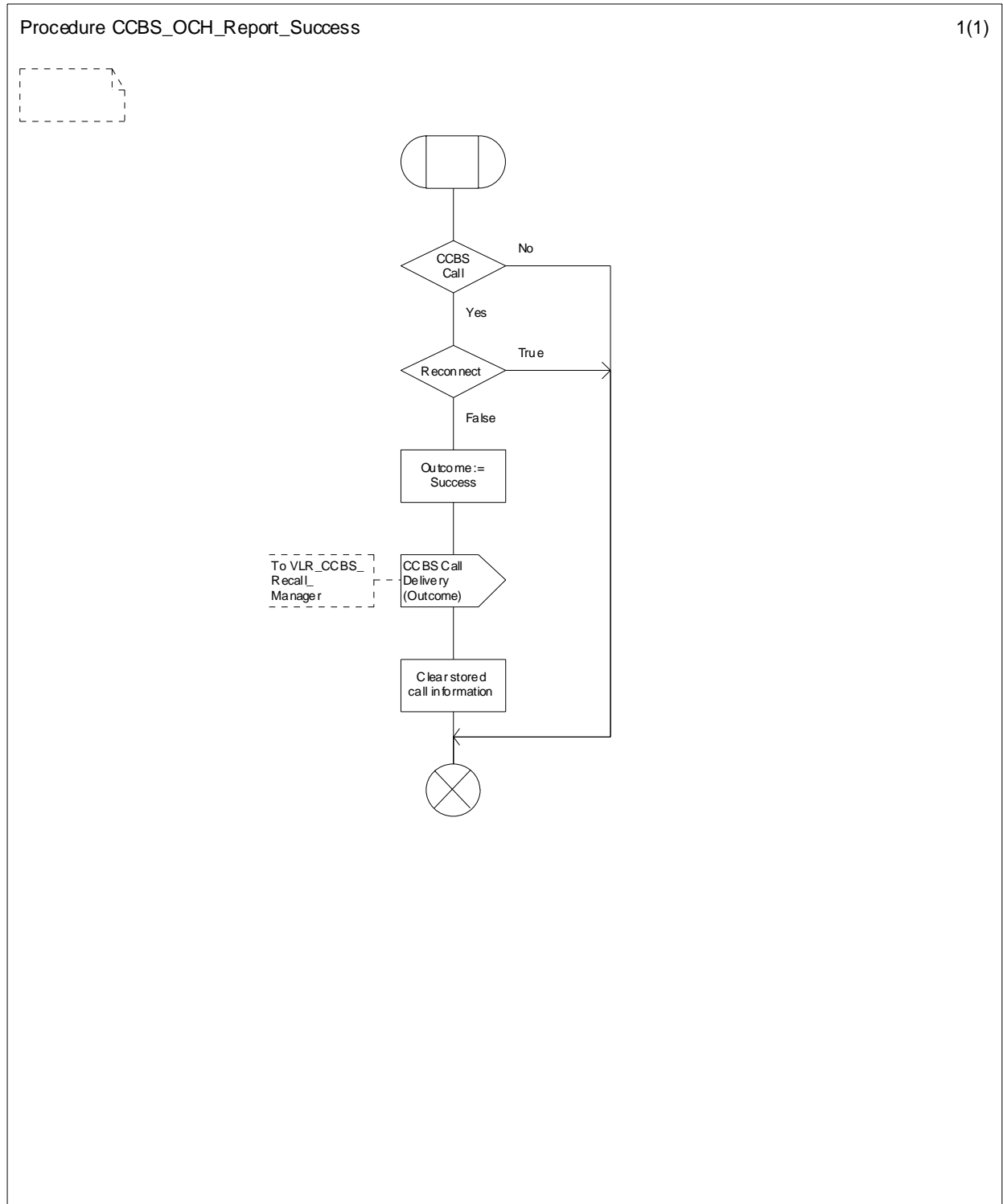
Figure 11.1.1.11: Procedure CCBS_OCH_Report_Success
