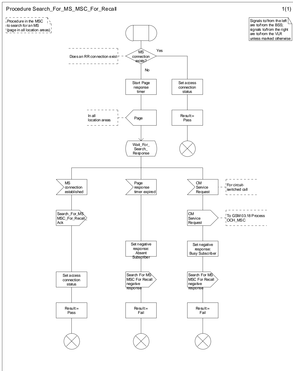
Figure 11.1.1.8: Procedure Search_For_MS_MSC_For_Recall
