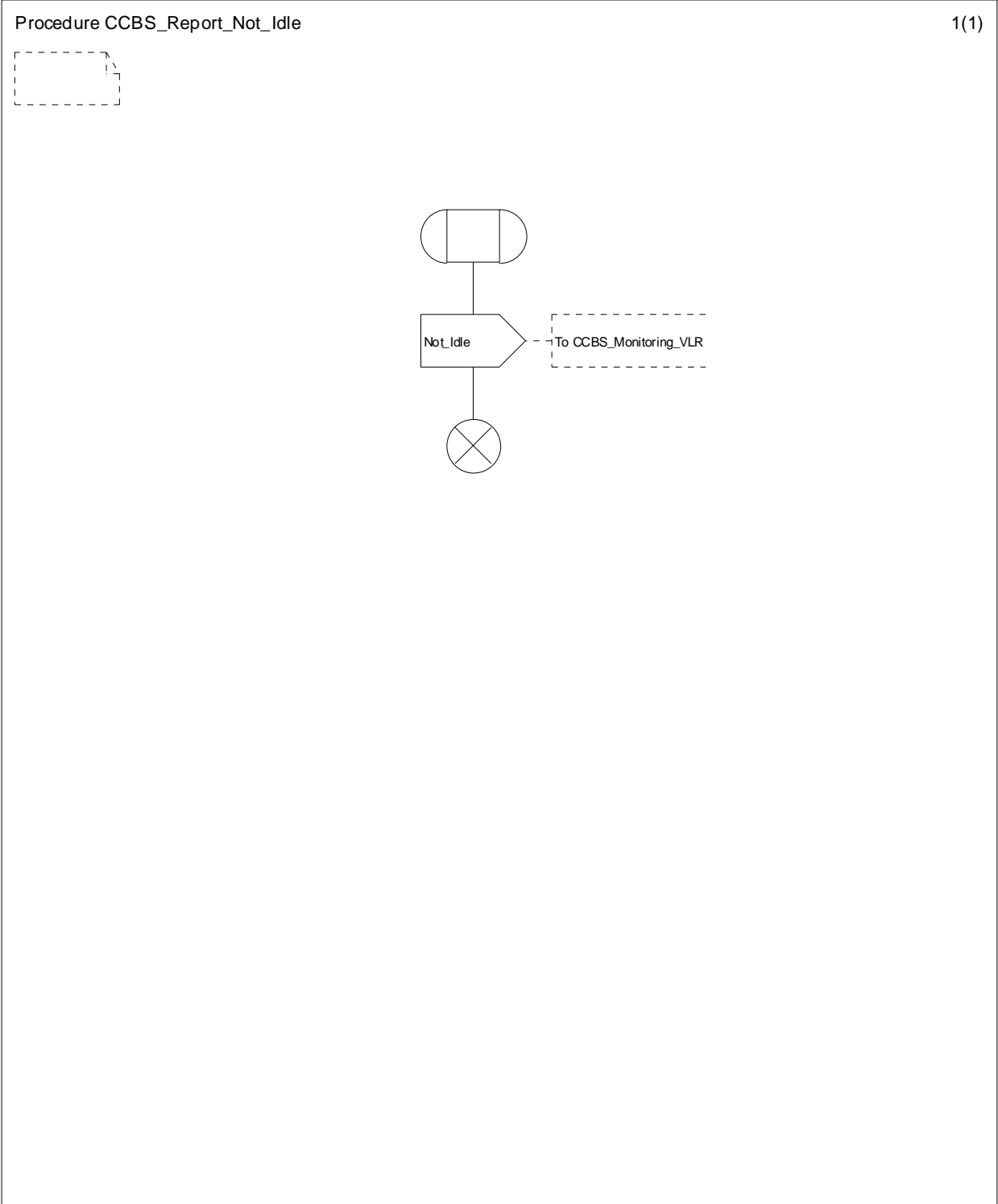
Figure 11.3.5: Procedure CCBS_Report_Not_Idle
