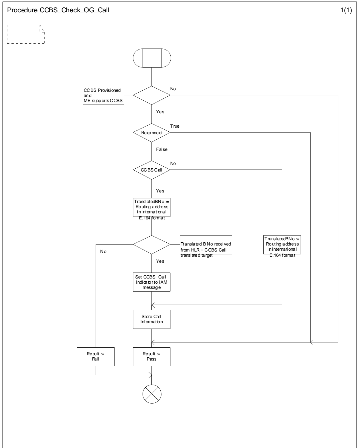
Figure 11.1.1.4: Procedure CCBS_Check_OG_Call
