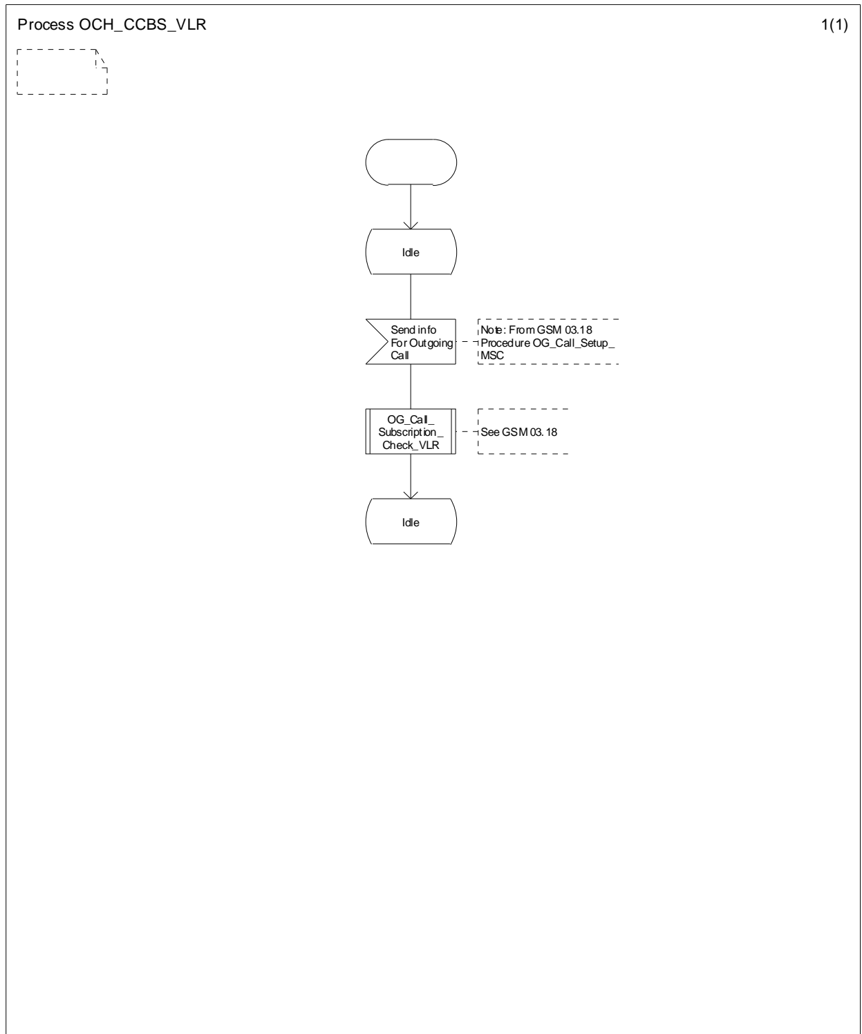
Figure 11.1.1.3: Process OCH_CCBS_VLR
