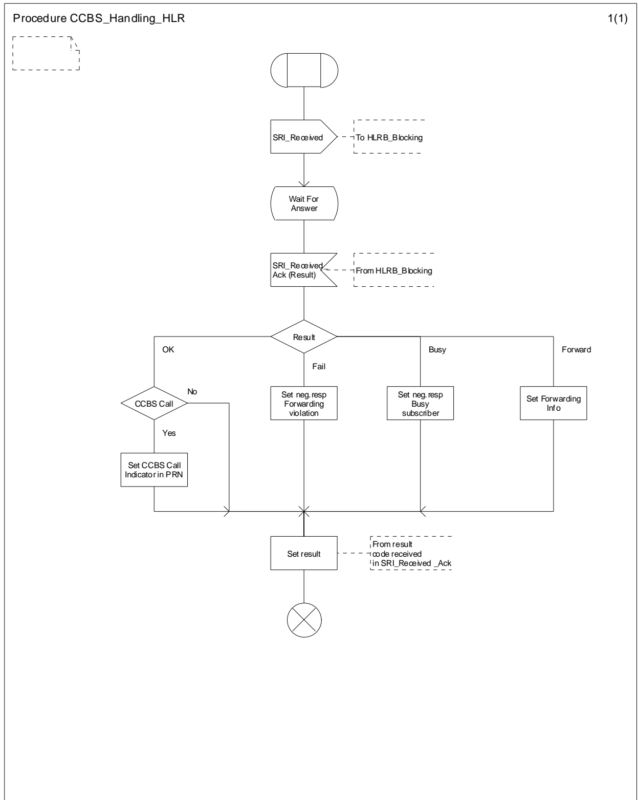
Figure 11.2.2.8: Procedure CCBS_Handling_HLR
