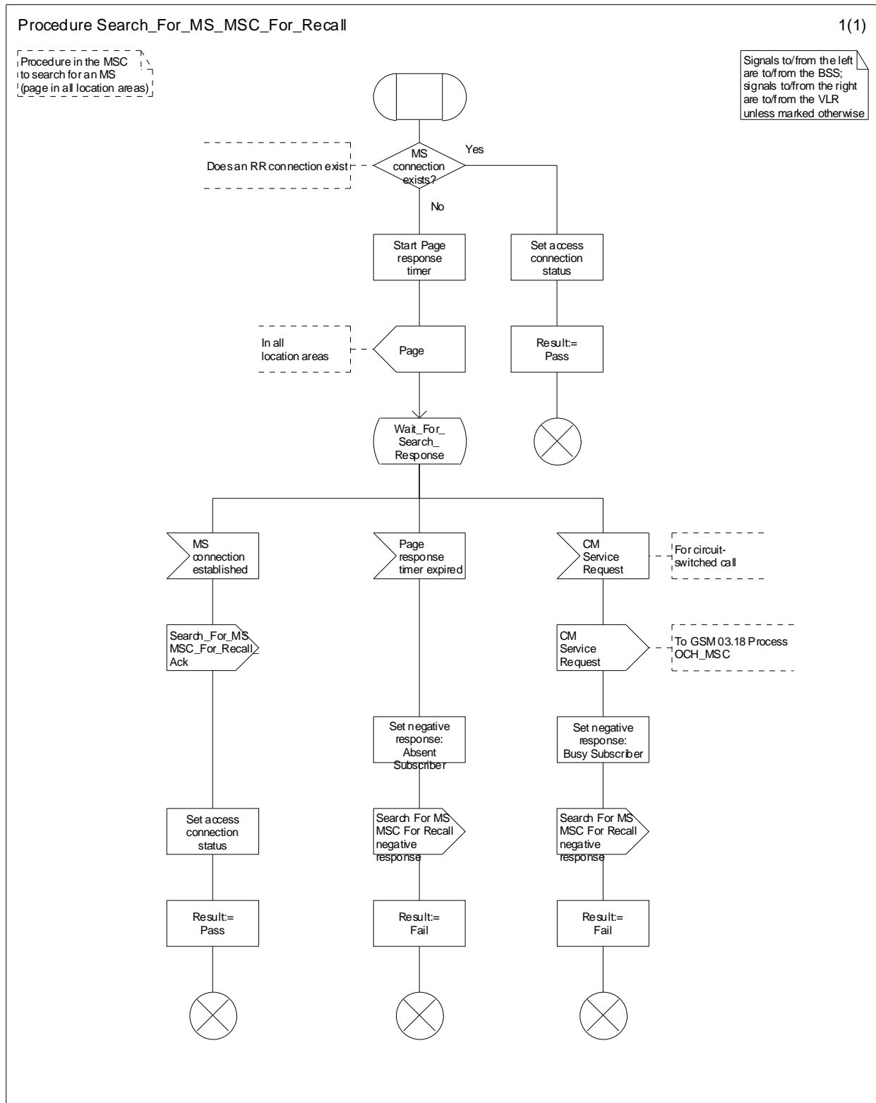
Figure 11.1.1.8: Procedure Search_For_MS_MSC_For_Recall
