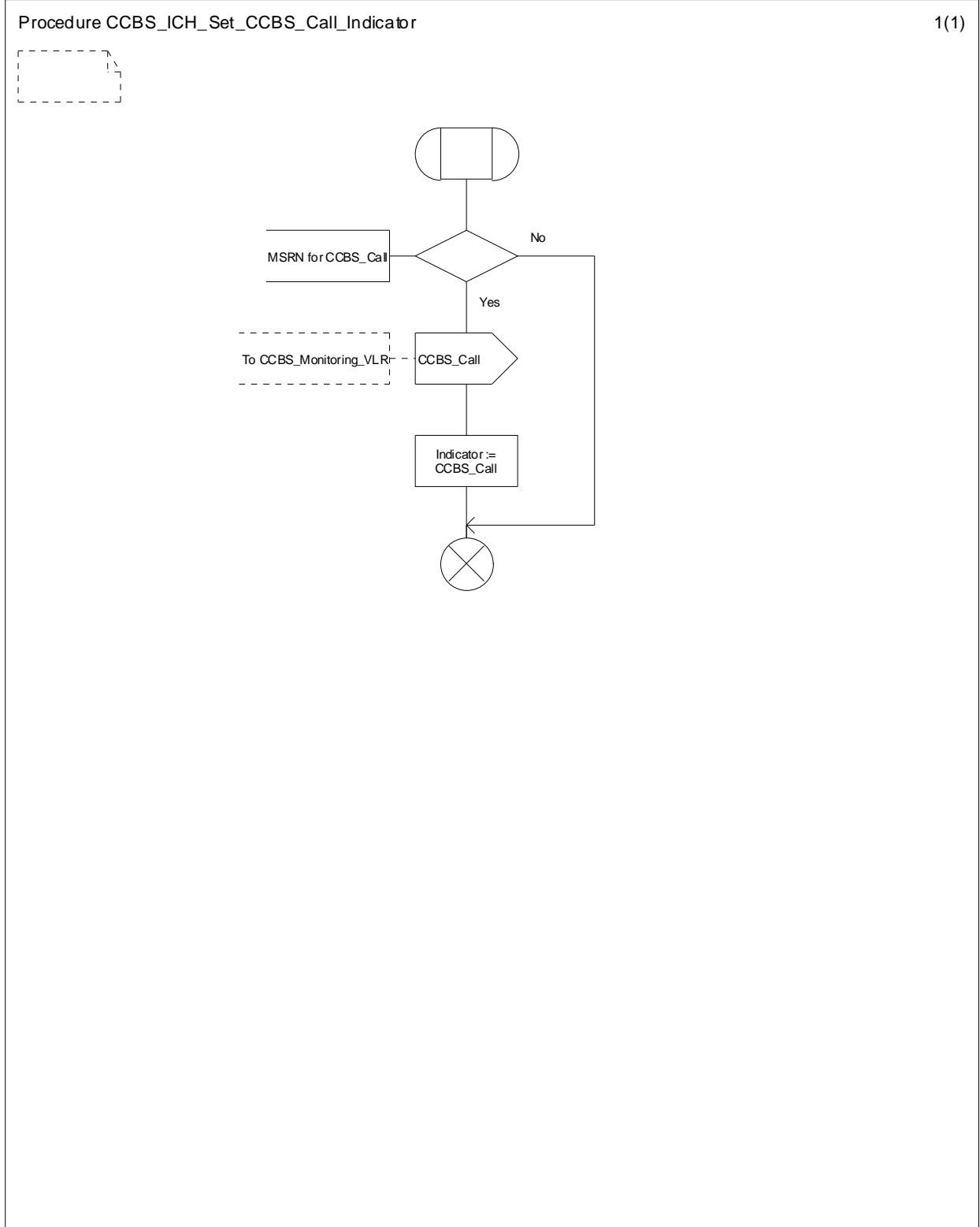
Figure 11.2.3.3: Procedure CCBS_ICH_Set_CCBS_Call_Indicator
