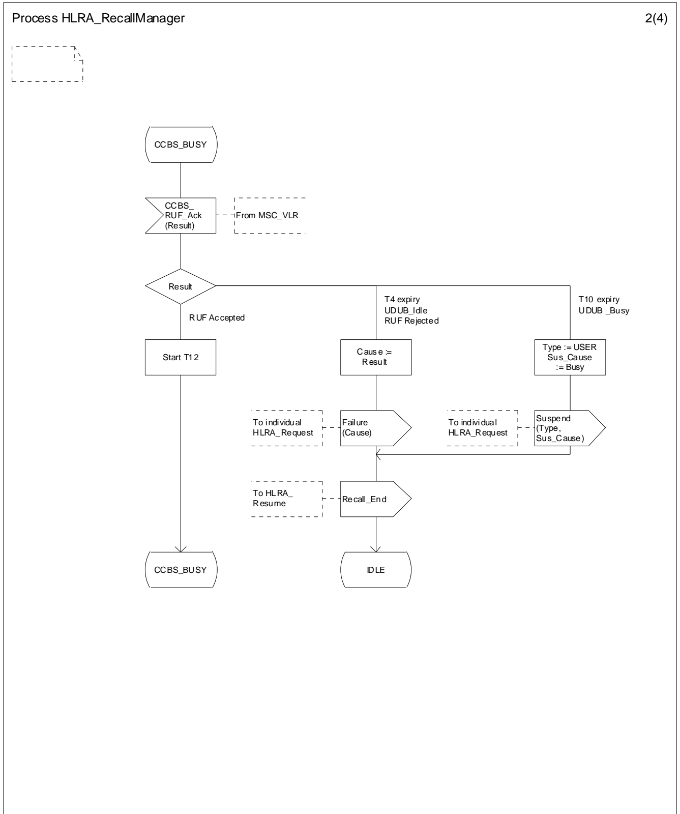
Figure 11.1.2.4: Process HLRA_Recall_Manager (sheet 2 of 4)
