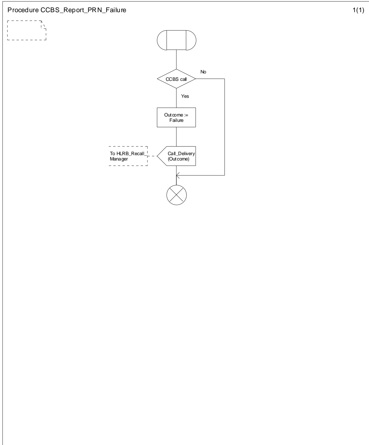
Figure 11.2.2.9: Procedure CCBS_Report_PRN_Failure
