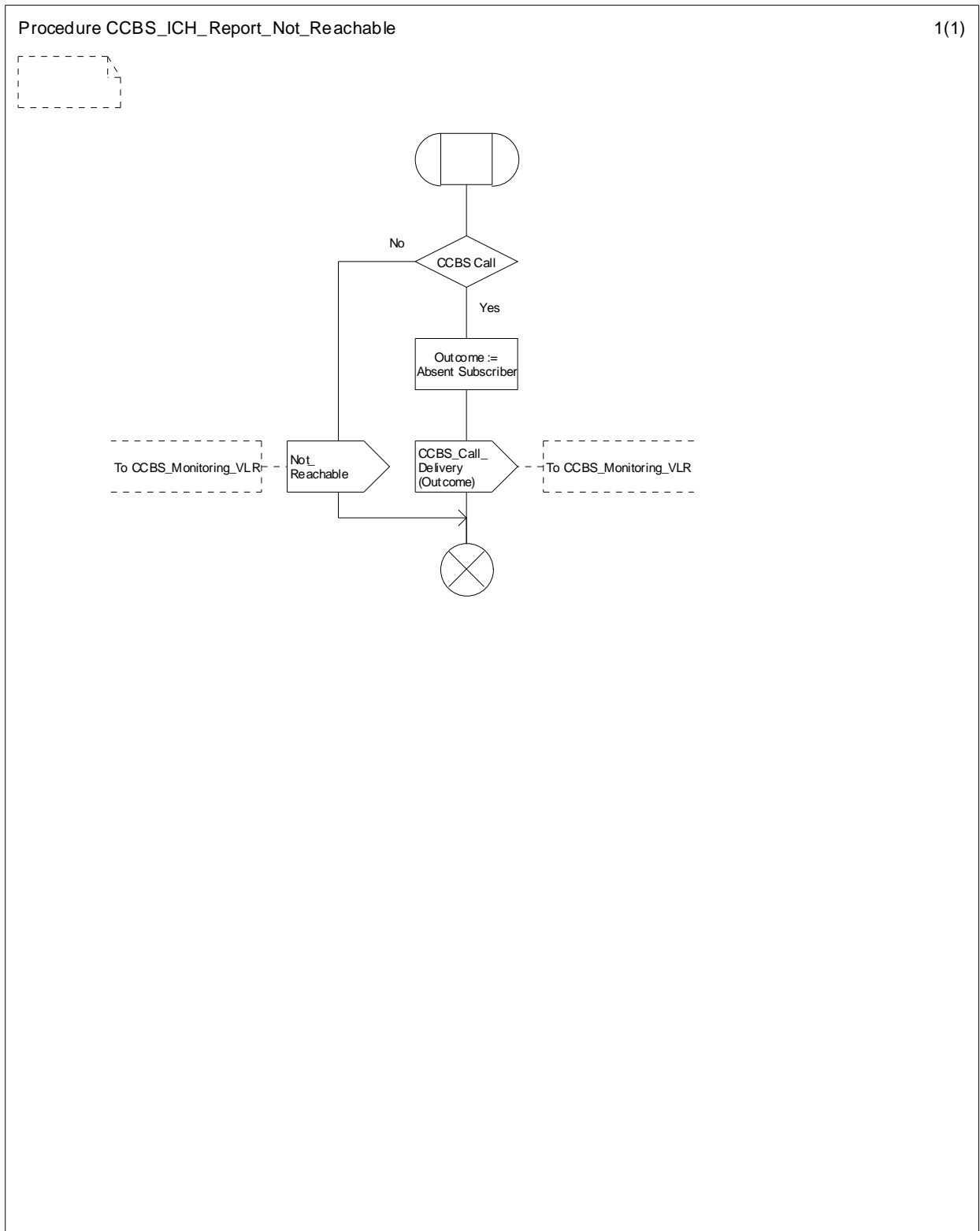
Figure 11.2.3.6: Procedure CCBS_ICH_Report_Not_Reachable
