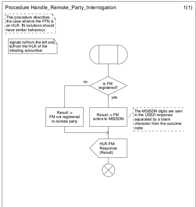
Figure 4.8: Procedure Handle_Remote_Party_Interrogation
