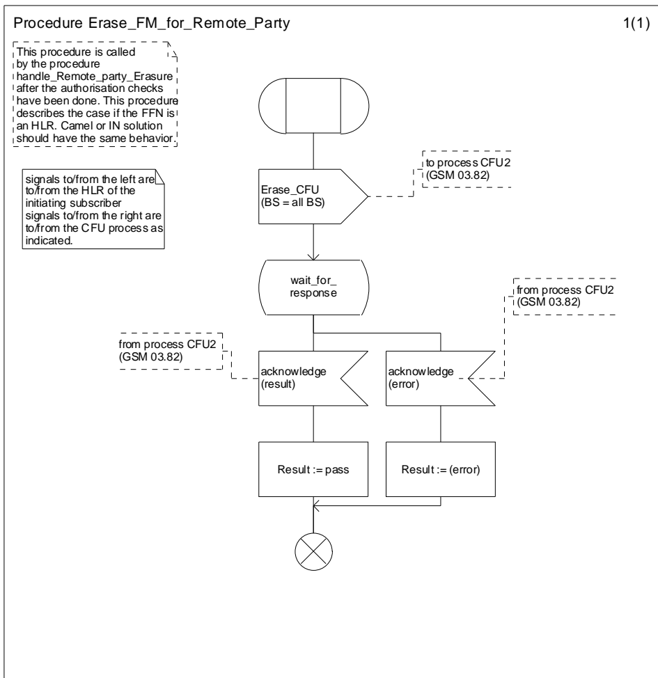
Figure 4.7a: Procedure Erase_FM_for_Remote_party
