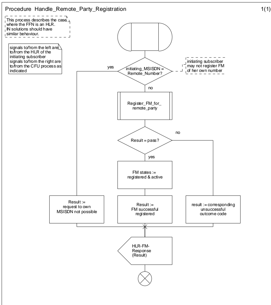
Figure 4.6: Procedure: Handle_Remote_Party_Registration
