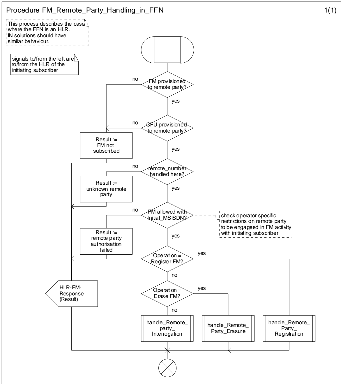
Figure 4.5: Procedure: FM_Remote_Party_Handling_in_FFN
