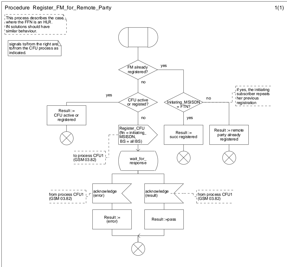
Figure 4.6a: Procedure Register_FM_for_Remote_Party
