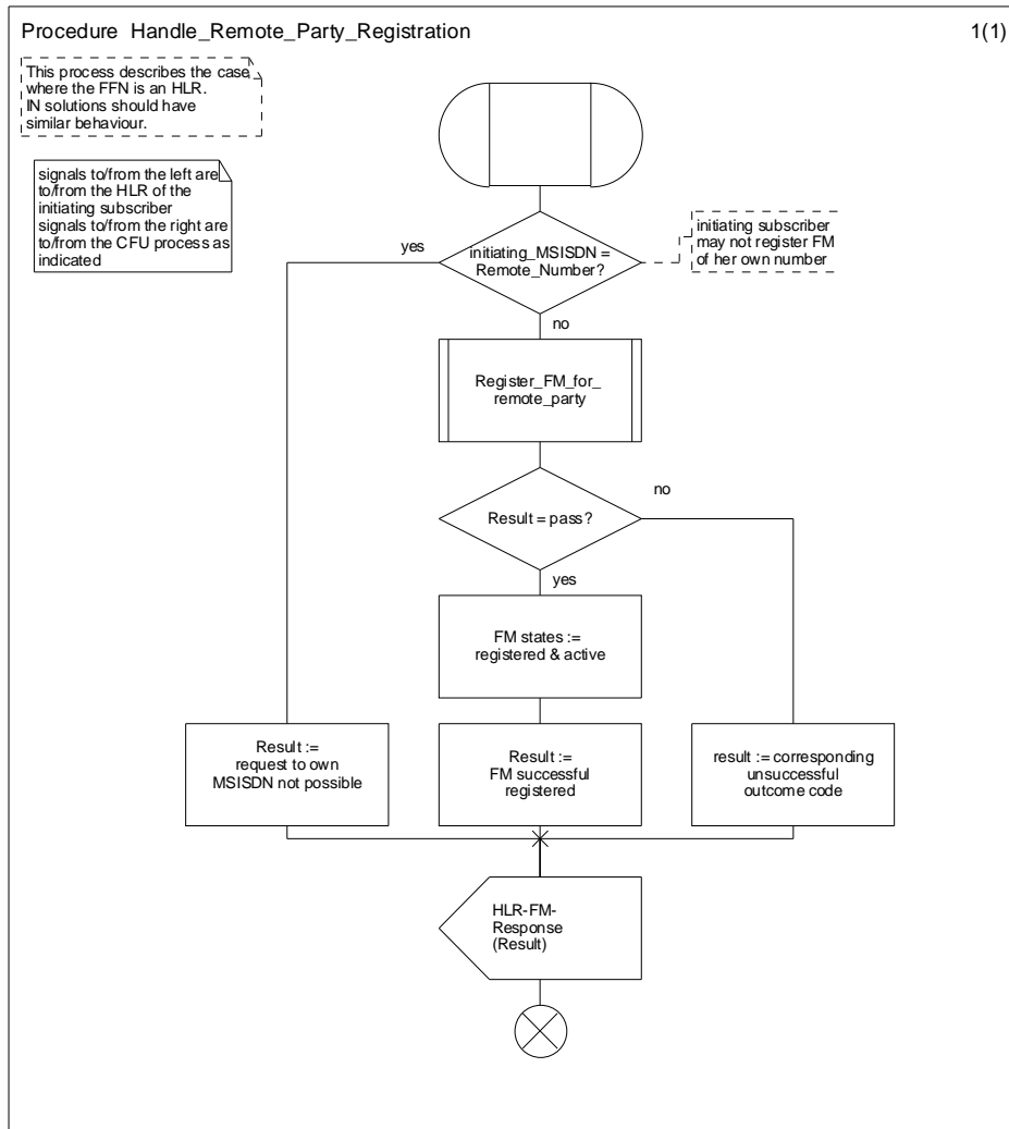
Figure 4.6: Procedure: Handle_Remote_Party_Registration
