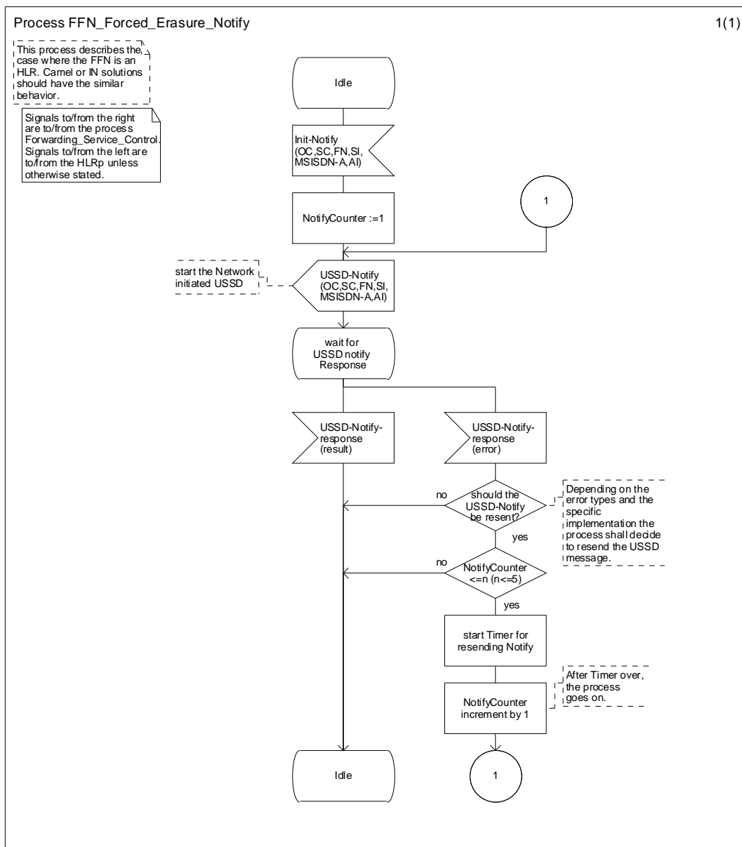
Figure 4.9: Process FFN_Forced_Erasure_Notify
