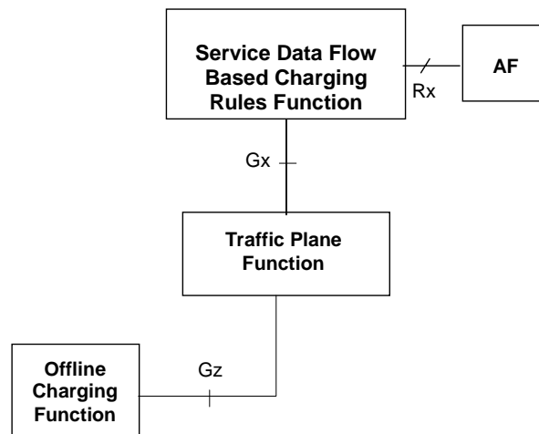
Figure 6.2: Overall architecture for service data flow based offline bearer charging
