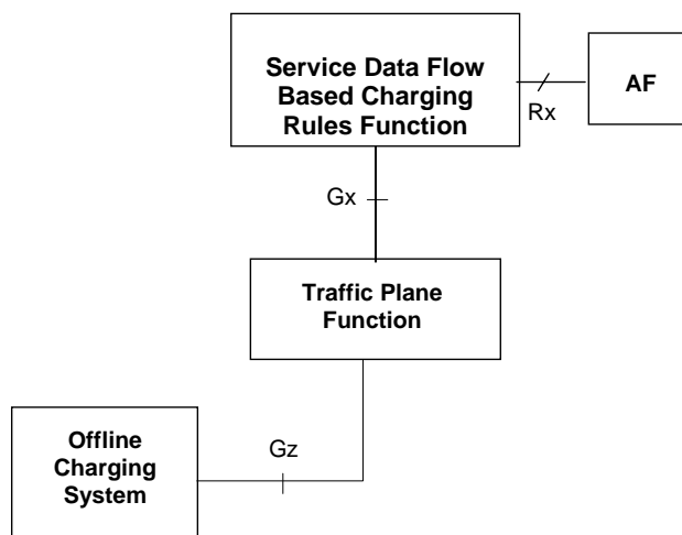
Figure 6.2: Overall architecture for service data flow based offline bearer charging
