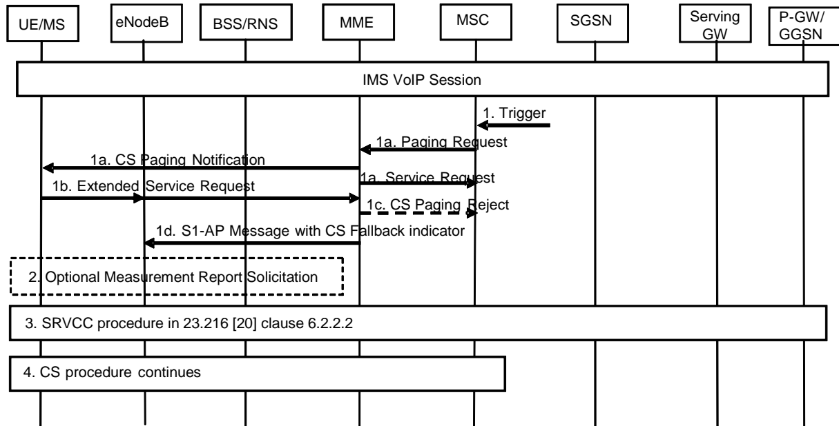
Figure 8.4.2.2-1: NW-Initiated CS Service procedure while UE is in IMS VoIP session
