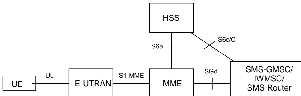
Figure C.2-1: SMS in MME Architecture
