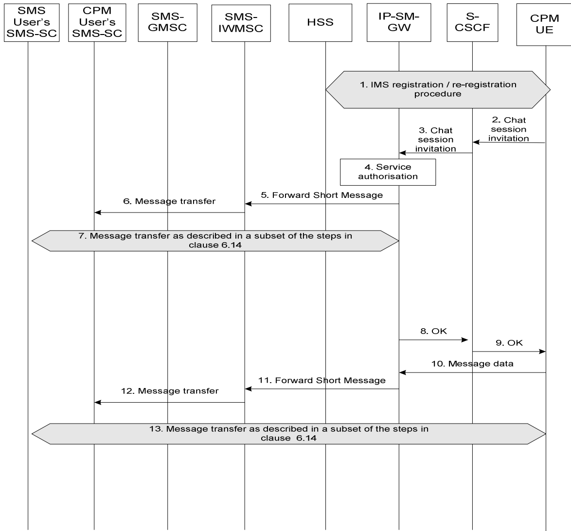
Figure 6.15.1: Chat session invitation to SMS user and Message data exchange (IP-SM-GW in originating network)
