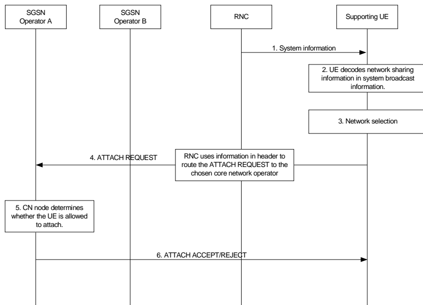
Figure 6: Network selection by a supporting UE in a UTRAN MOCN
