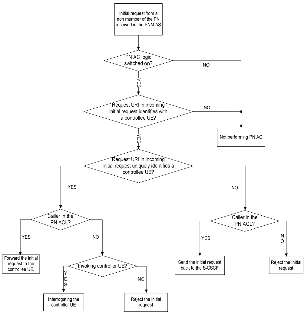
Figure 7.1-2: PN access control execution flow at the PNM AS (AC and ACL stand for Access Control and Access Control List, respectively)
