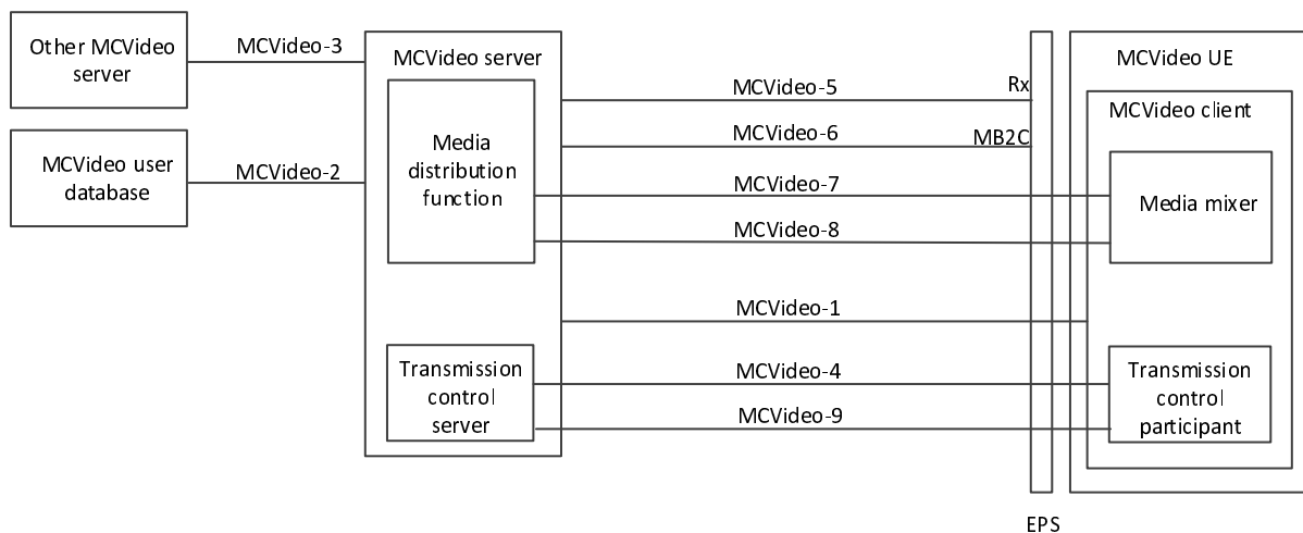
Figure 6.1.1-1: Functional model for application plane of MCVideo service
