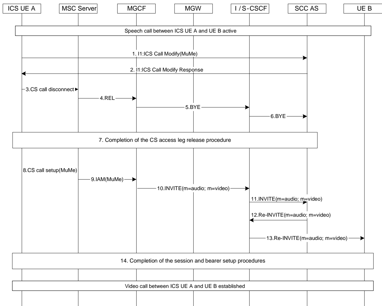
Figure 7.9.2.5-2: Addition of video media flow for ICS UE via the MSC Server not enhanced for ICS through redial using I1 reference point
