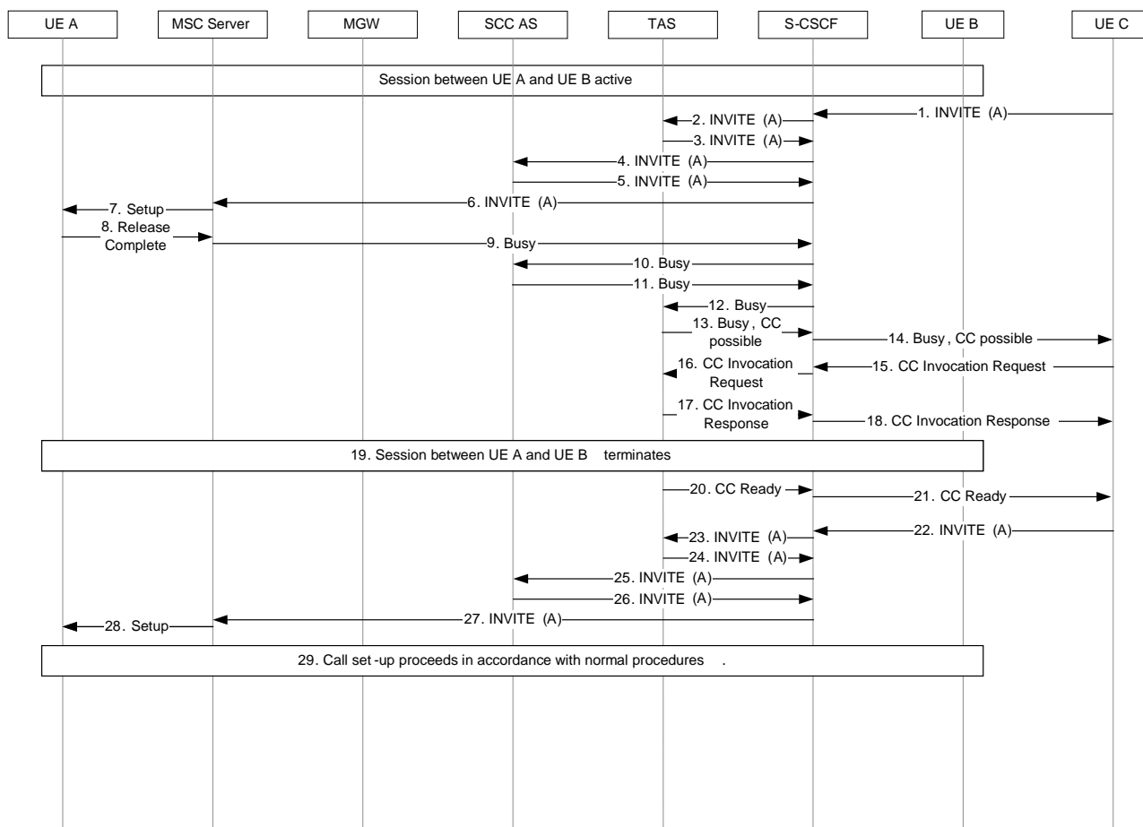
Figure 7.6.2.11.1-1: IMS Communication Completion to Busy Subscriber via MSC Server enhanced for ICS
