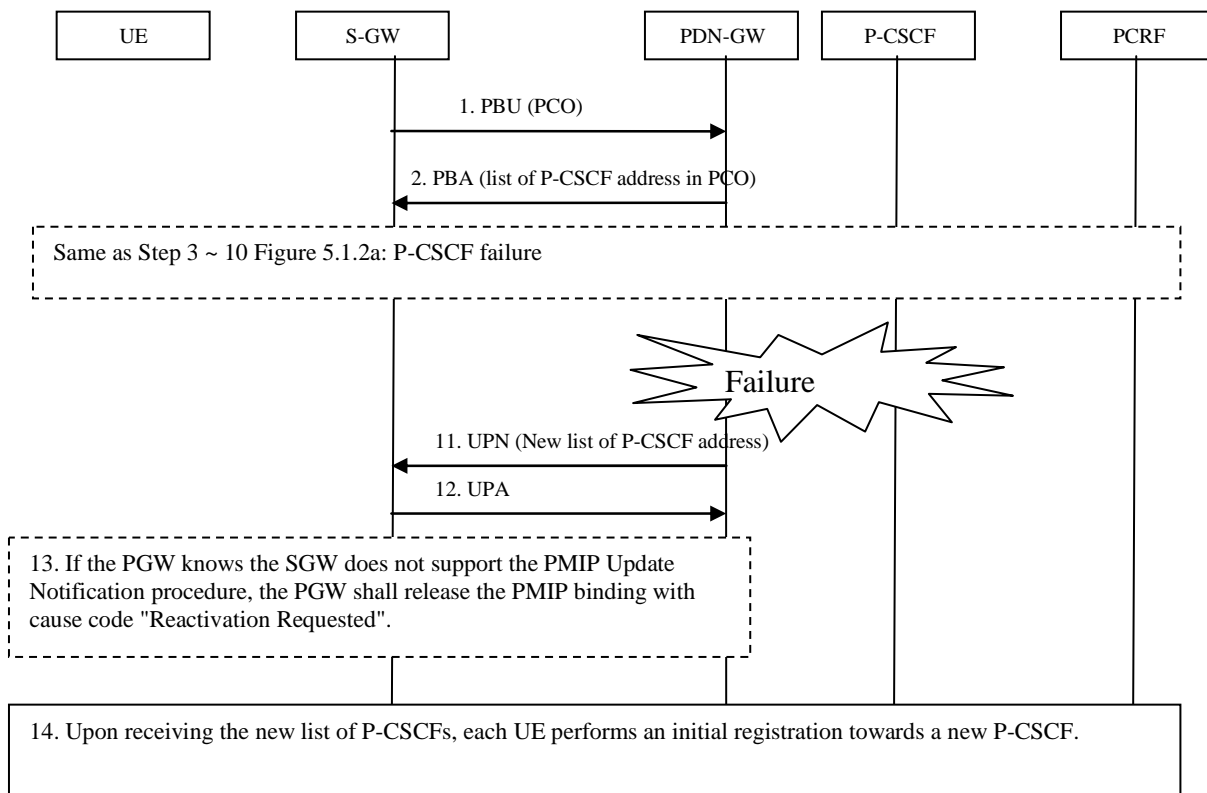
Figure 5.1.3: P-CSCF failure with S5 PMIP
