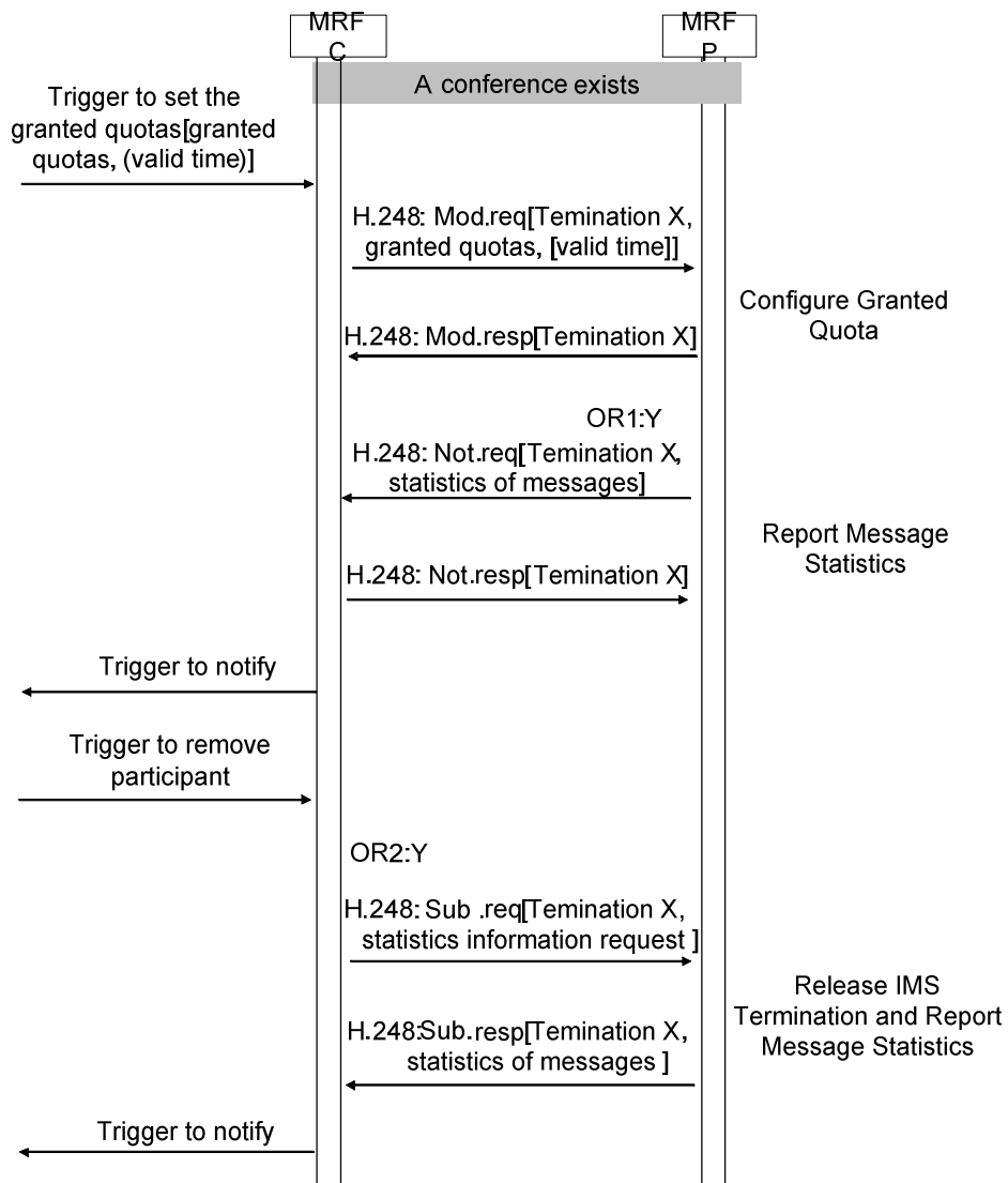
Figure 6.2.10.3.2.1 shows the message sequence chart example for reporting message statistics.
