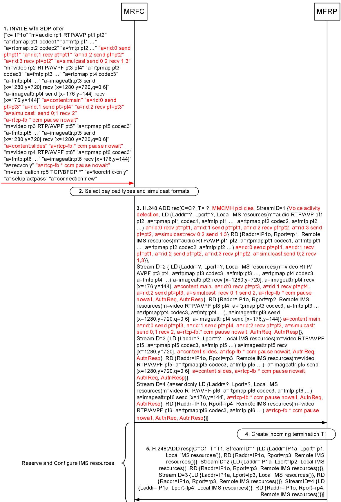
Figure 6.2.10.2.7.2.1: Multi-stream multiparty conference establishment ("dial-in" procedure) with support of "simulcast" and "RTP-level pause and resume"
