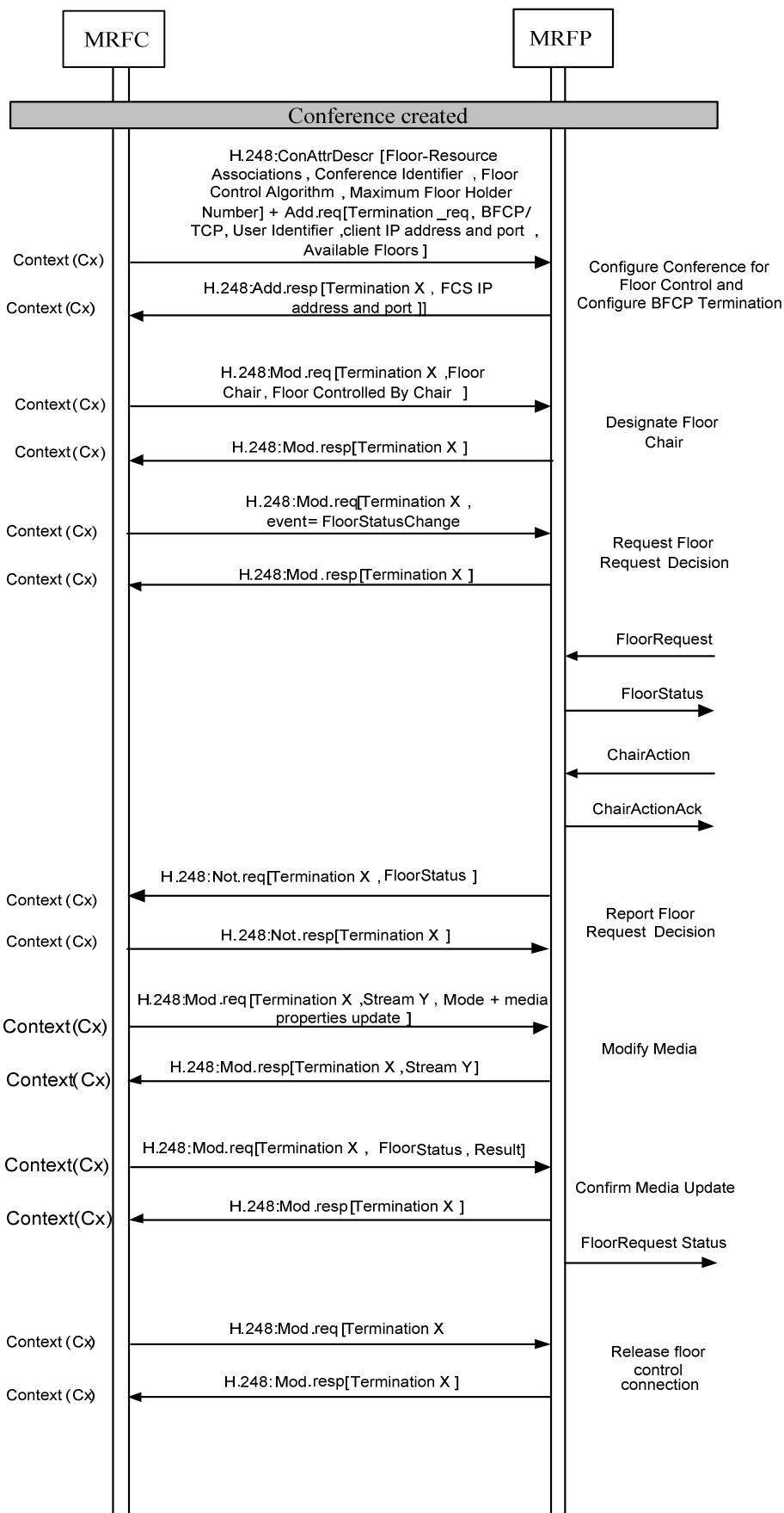
Figure 6.2.13.1 Floor control (message sequence chart)
