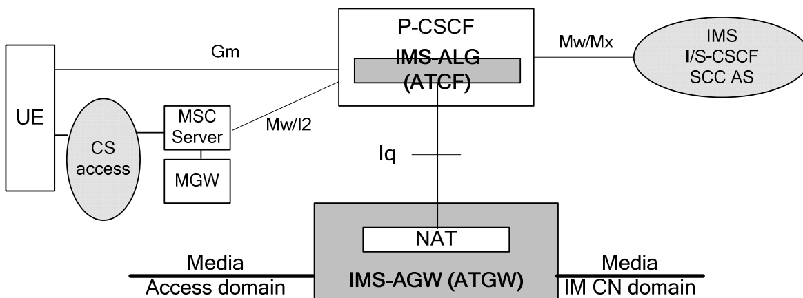
Figure 4.1.2: Reference Architecture for IMS-ALG/IMS-AGW with ATCF/ATGW function
