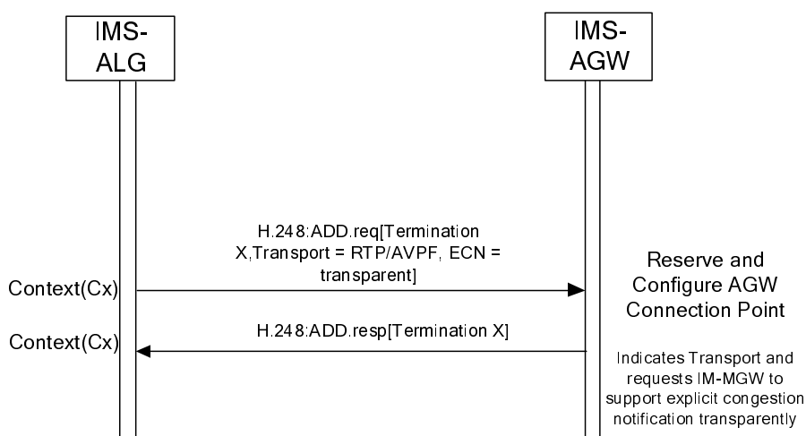
Figure 6.2.13.2.1: Procedure to indicate ECN negotiated
