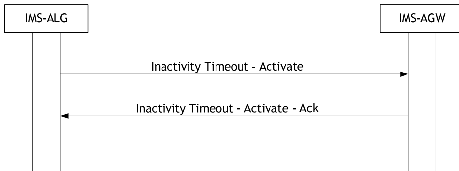
Figure 6.1.13.1: Inactivity Timeout - Activate
